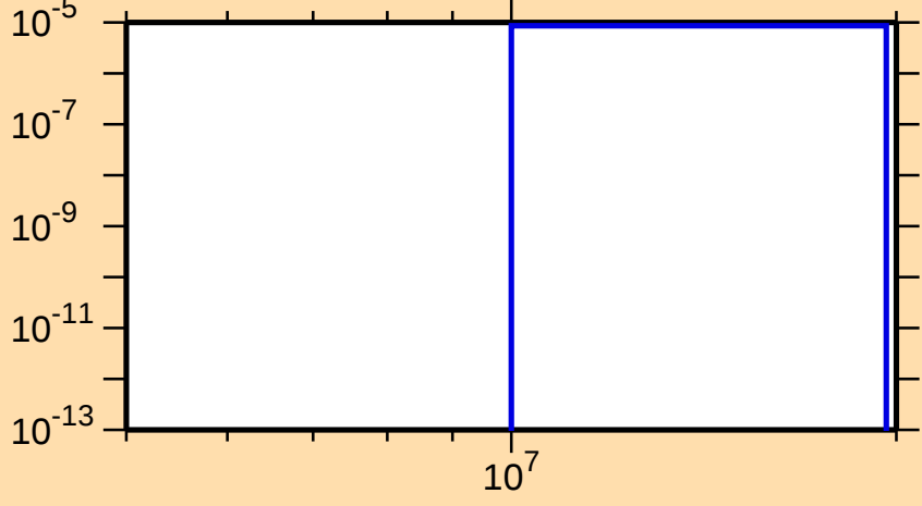
\sigma vs. E for ^{142}\text{Nd}(n,t)
