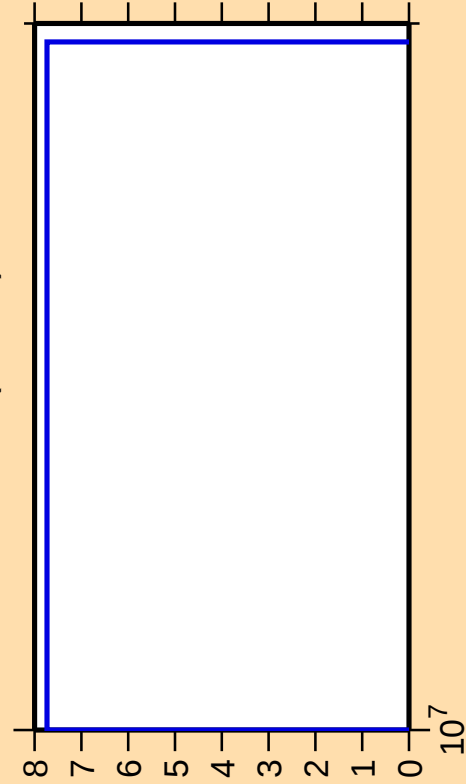
\Delta\sigma/\sigma vs. E for ^{142}\text{Nd}(n,2n\alpha)
