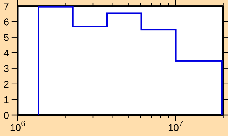
\Delta\sigma/\sigma vs. E for ^{142}\text{Nd}(\text{n,nonel.})
