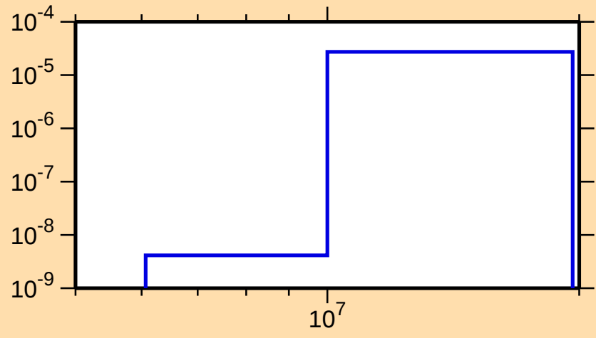
\sigma vs. E for ^{142}\text{Nd}(n,\alpha)
