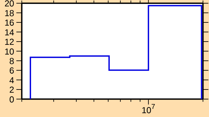
\Delta\sigma/\sigma vs. E for ^{142}\text{Nd}(n,n\text{cont.})
