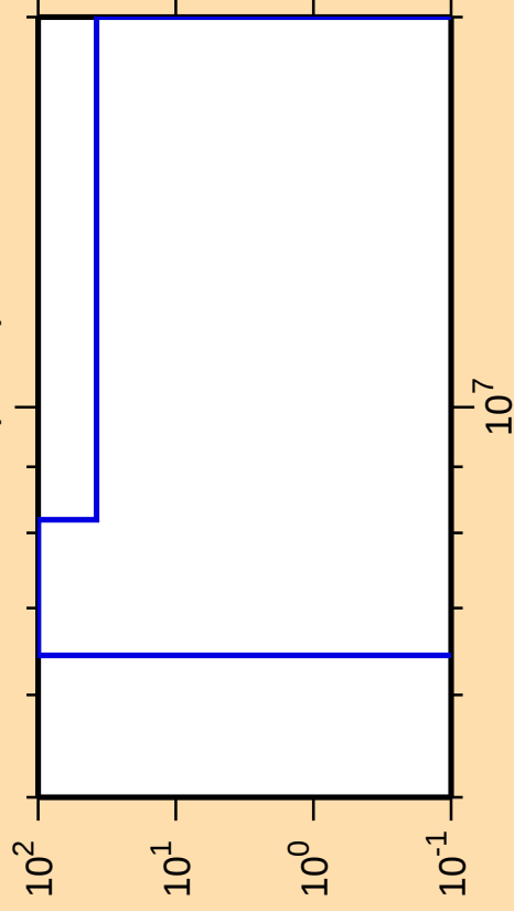
\Delta\sigma/\sigma vs. E for ^{142}\text{Nd}(n,\alpha)
