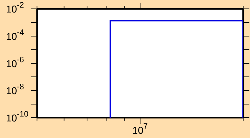
\sigma vs. E for ^{142}\text{Nd}(n,d)
