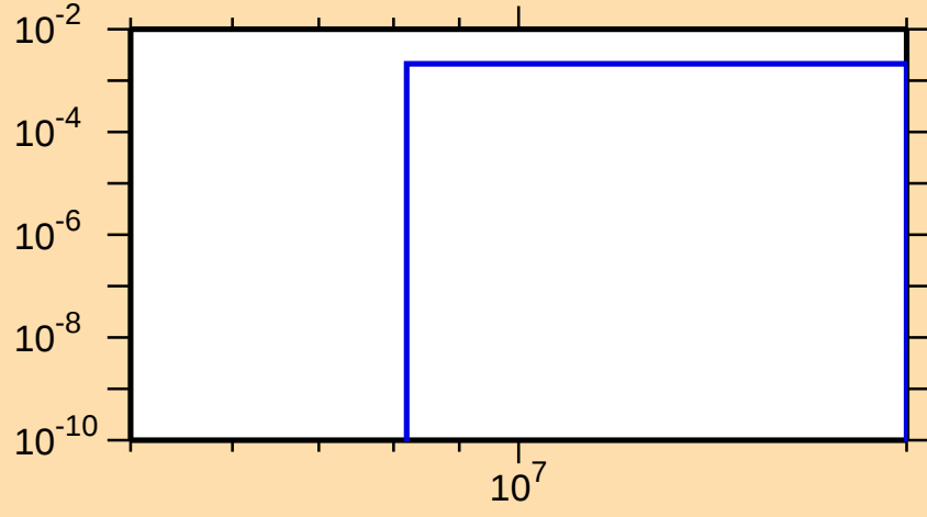
\sigma vs. E for ^{142}\text{Nd}(n,np)
