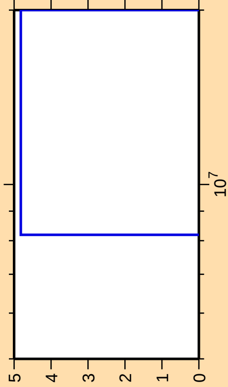
\Delta\sigma/\sigma vs. E for ^{142}\text{Nd}(n,\text{pd})
