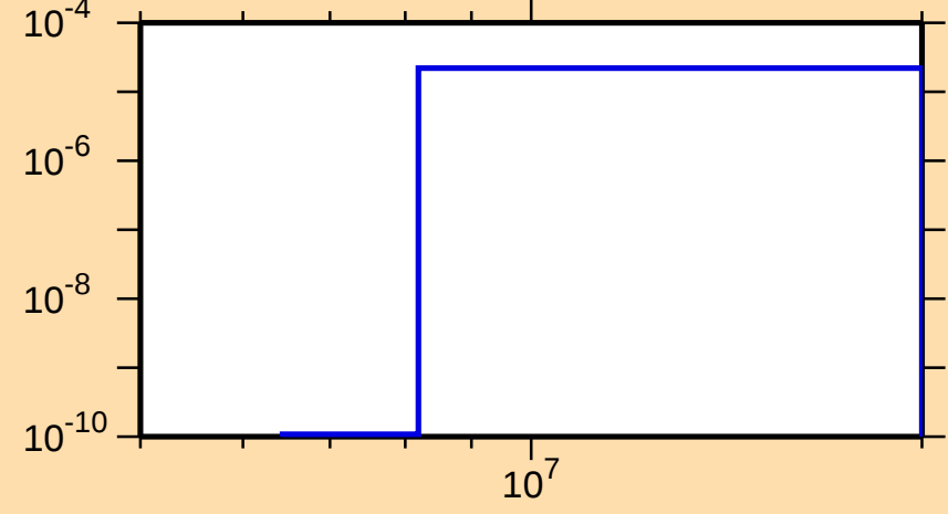
\sigma vs. E for ^{142}\text{Nd}(n,\alpha)
