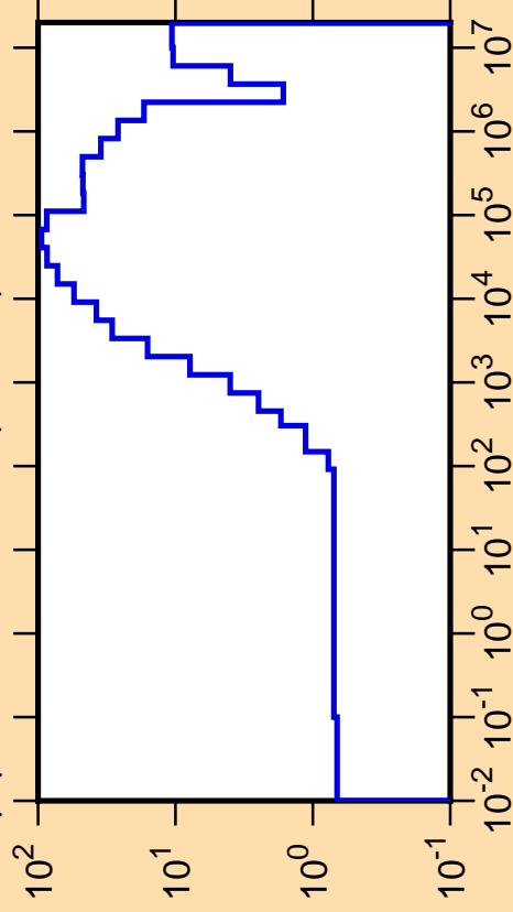
\Delta\mu/\mu vs. E for ^{143}\text{Nd}(\text{mt251})
