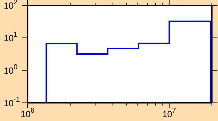
\Delta\sigma/\sigma vs. E for ^{143}\text{Nd}(n,\text{inel.})
