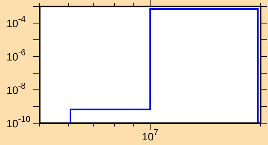
\sigma vs. E for ^{143}\text{Nd}(n,d)
