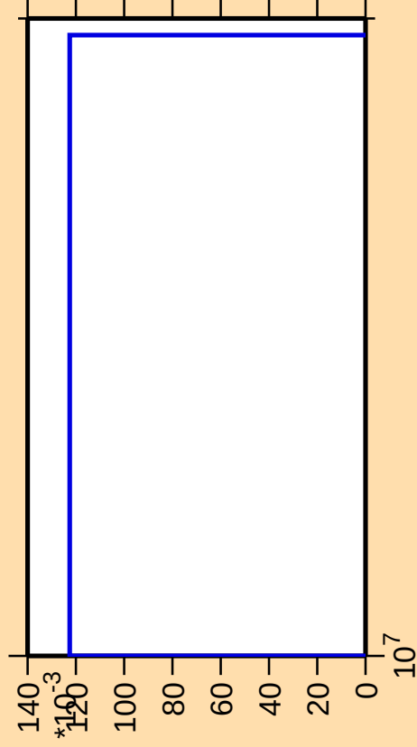
\Delta\sigma/\sigma vs. E for ^{143}\text{Nd}(\text{mt } 34)
