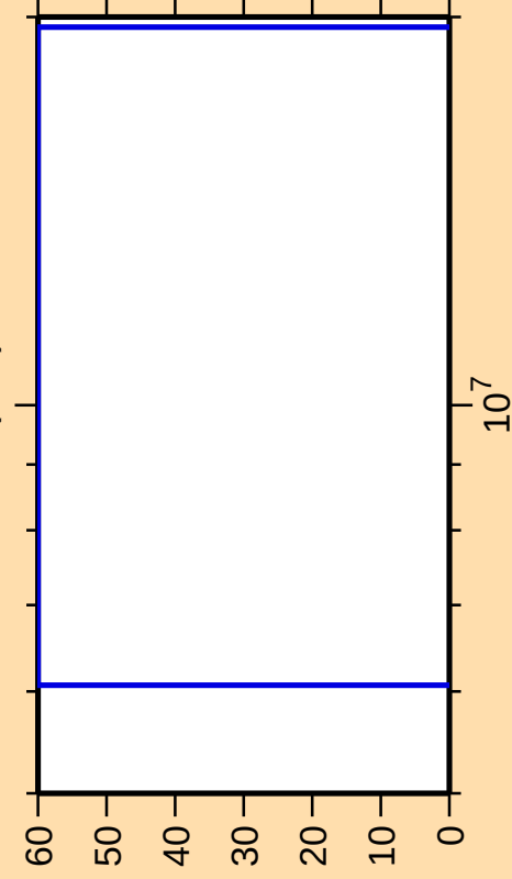
\Delta\sigma/\sigma vs. E for ^{143}\text{Nd}(n,d)
