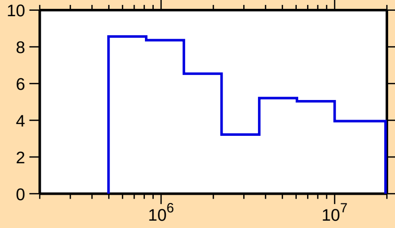
\Delta\sigma/\sigma vs. E for ^{143}\text{Nd}(\text{n,nonel.})
