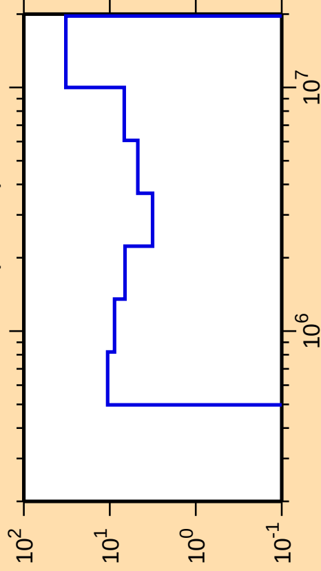
\Delta\sigma/\sigma vs. E for ^{143}\text{Nd}(\text{n,inel.})
