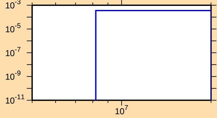
\sigma vs. E for ^{143}\text{Nd}(n,t)
