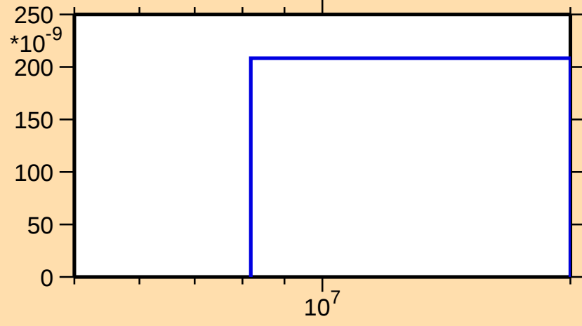
\sigma vs. E for ^{143}\text{Nd}(n,\text{nd})
