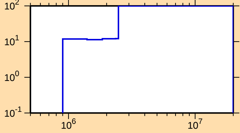
\Delta\sigma/\sigma vs. E for ^{143}\text{Nd}(n,\gamma)
