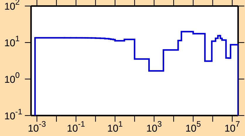
\Delta\sigma/\sigma vs. E for ^{143}\text{Nd}(n,\text{el.})
