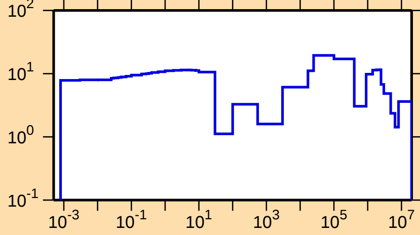
\Delta\sigma/\sigma vs. E for ^{143}\text{Nd}(n,\text{tot.})
