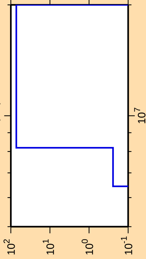
\Delta\sigma/\sigma vs. E for ^{143}\text{Nd}(n,t)
