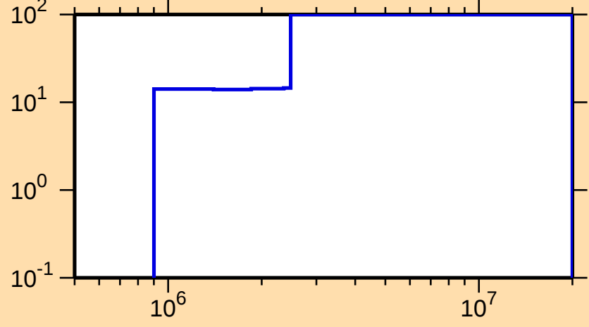
\Delta\sigma/\sigma vs. E for ^{143}\text{Nd}(n,n_1)
