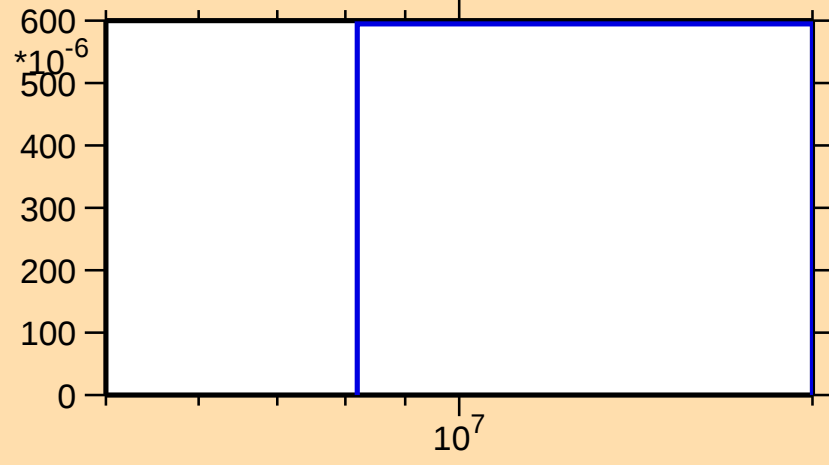
\sigma vs. E for ^{143}\text{Nd}(n,np)
