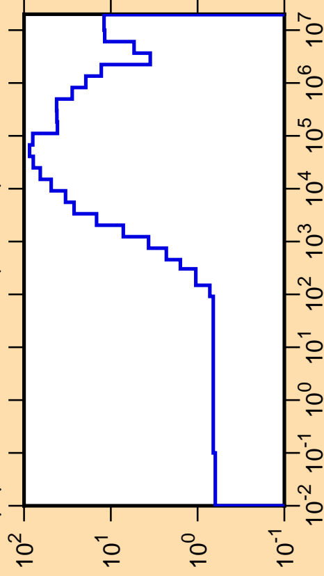
\Delta\mu/\mu vs. E for ^{145}\text{Nd}(\text{mt251})
