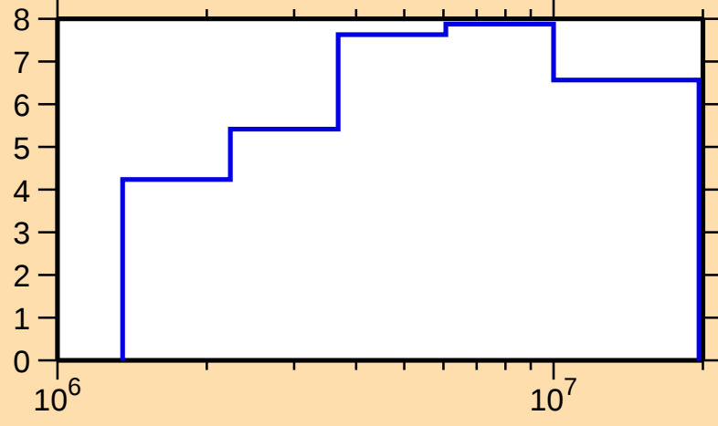
\Delta\sigma/\sigma vs. E for ^{145}\text{Nd}(n,n\text{nonel.})
