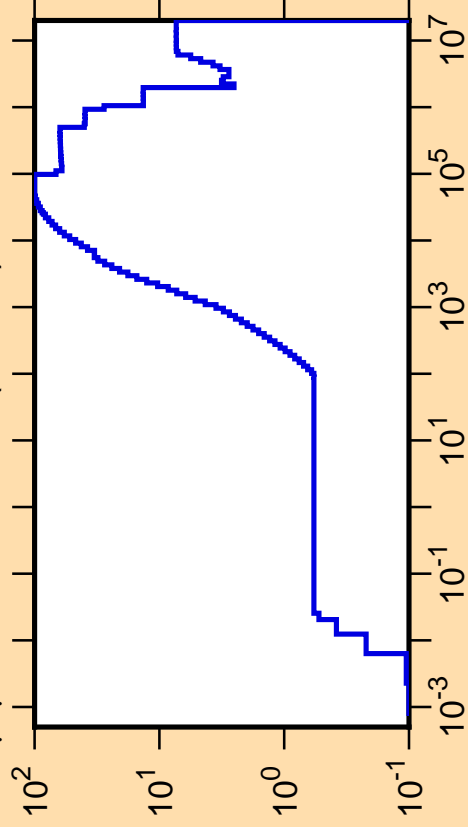
\Delta\mu/\mu vs. E for ^{146}\text{Nd}(\text{mt251})
