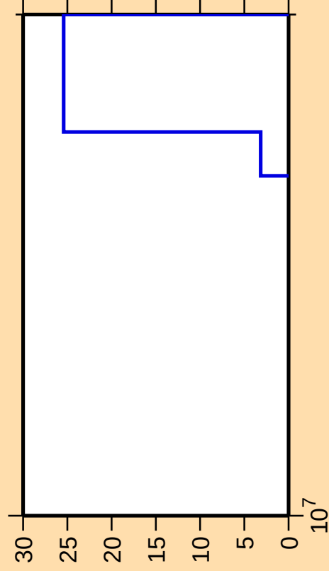
\Delta\sigma/\sigma vs. E for ^{146}\text{Nd}(n,p\alpha)
