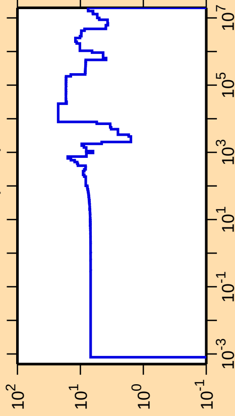
\Delta\sigma/\sigma vs. E for ^{146}\text{Nd}(n,\text{el.})
