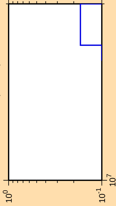
\Delta\sigma/\sigma vs. E for ^{146}\text{Nd}(\text{mt117})
