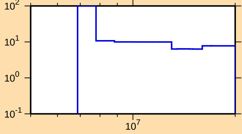
\Delta\sigma/\sigma vs. E for ^{146}\text{Nd}(n,2n)
