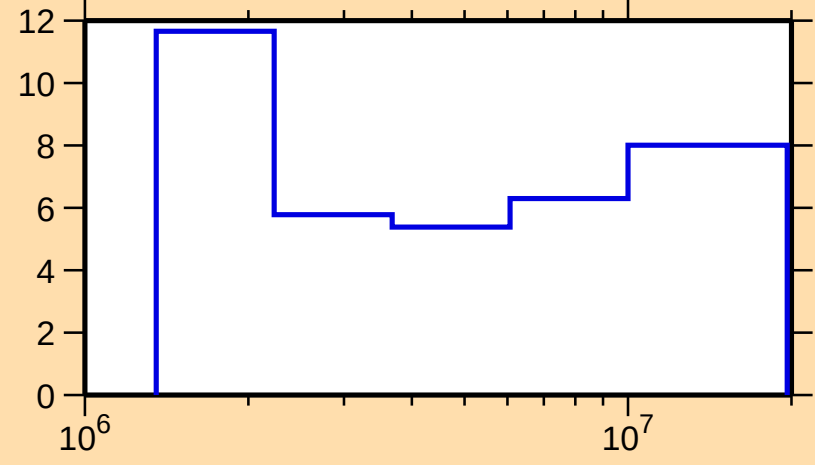
\Delta\sigma/\sigma vs. E for ^{146}\text{Nd}(\text{n},\text{nonel.})
