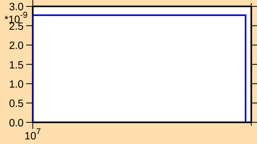
\sigma vs. E for ^{146}\text{Nd}(n,\text{nt})
