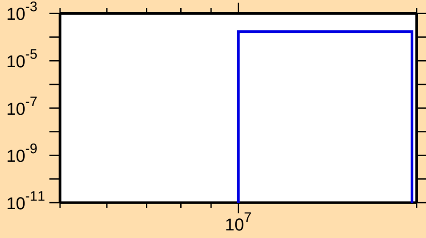
\sigma vs. E for ^{146}\text{Nd}(n,np)
