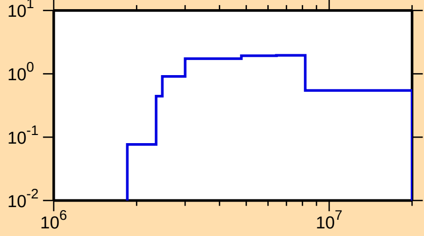
\sigma vs. E for ^{146}\text{Nd}(n,n\text{cont.})
