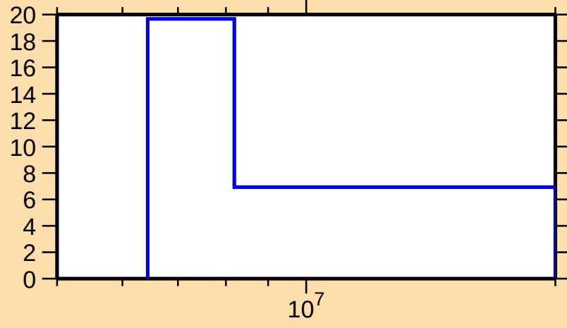
\Delta\sigma/\sigma vs. E for ^{146}\text{Nd}(n,2n)
