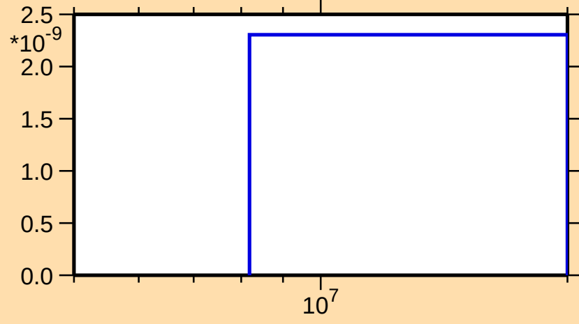
\sigma vs. E for ^{146}\text{Nd}(n,\text{nd})
