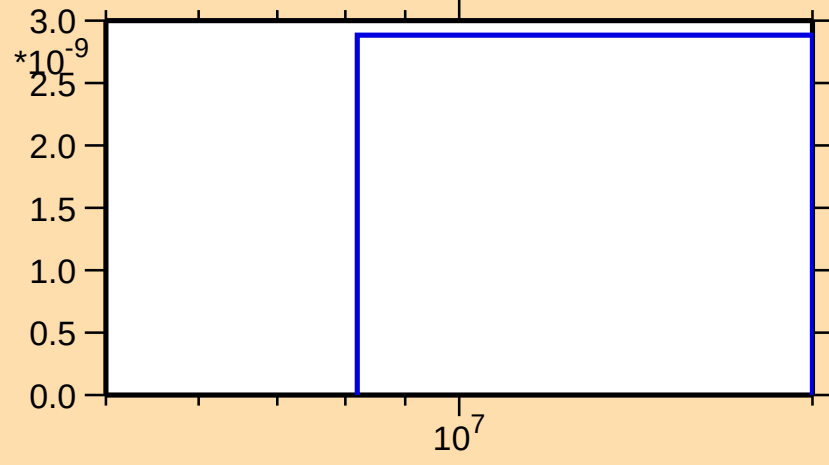
\sigma vs. E for ^{146}\text{Nd}(n,\text{nt})
