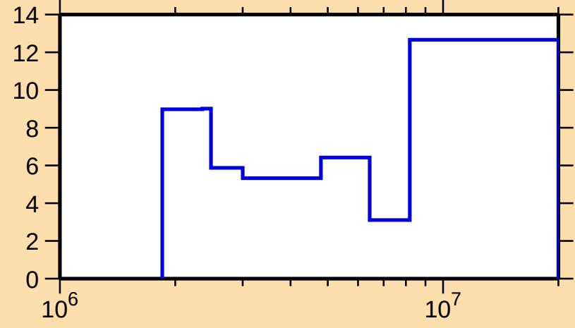
\Delta\sigma/\sigma vs. E for ^{146}\text{Nd}(n,\text{inel.})
