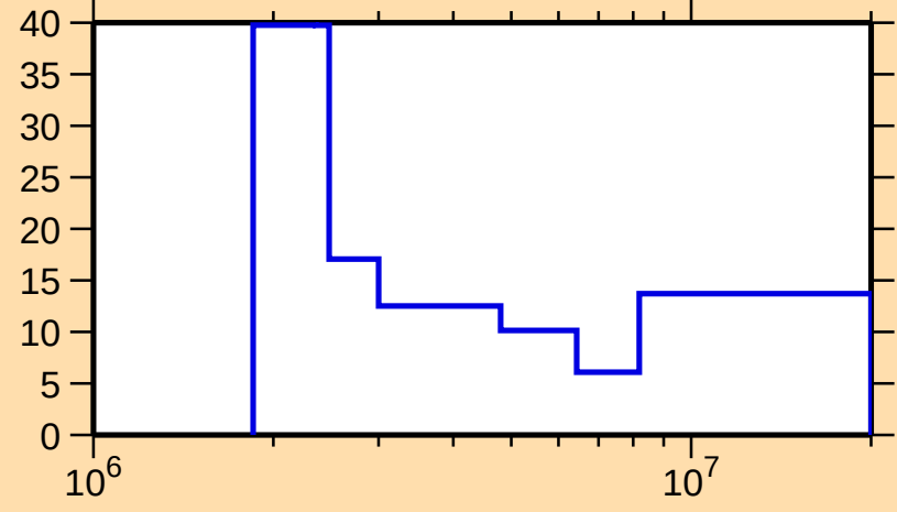
\Delta\sigma/\sigma vs. E for ^{146}\text{Nd}(n,n\text{cont.})
