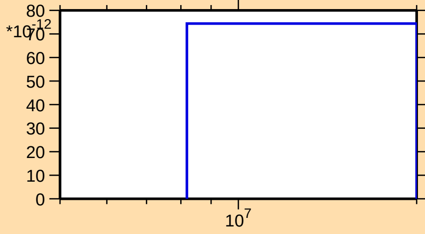
\sigma vs. E for ^{146}\text{Nd}(n,2np)
