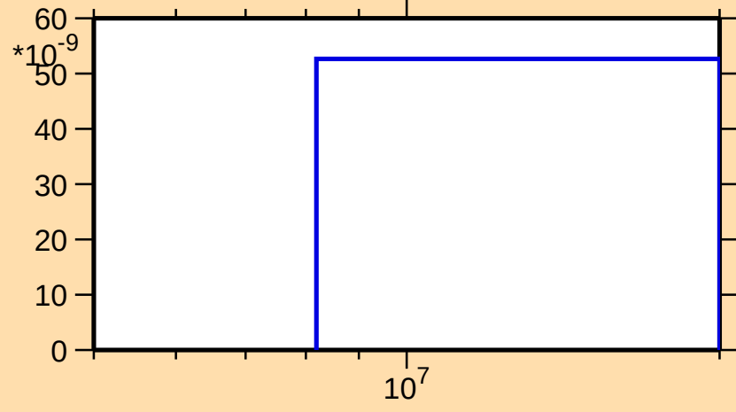
\sigma vs. E for ^{146}\text{Nd}(n,2n\alpha)
