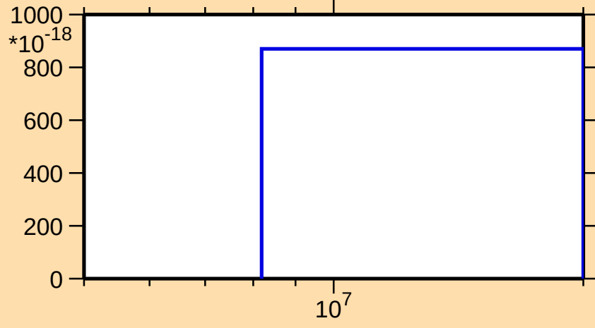
\sigma vs. E for ^{146}\text{Nd}(\text{mt117})
