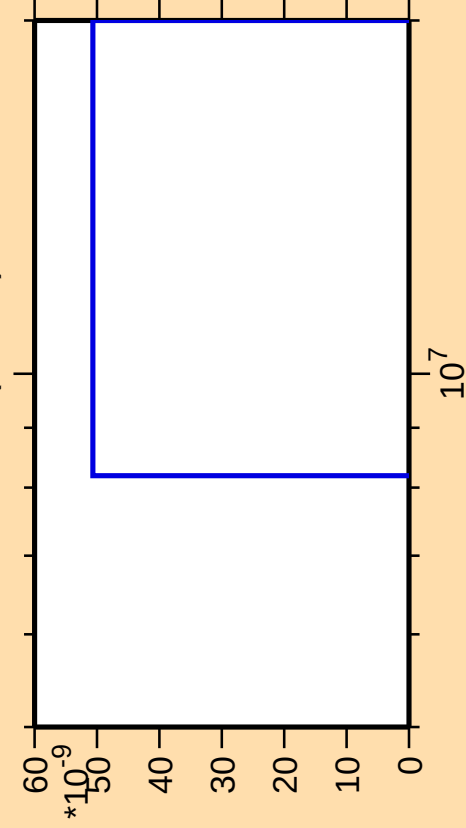
\Delta\sigma/\sigma vs. E for ^{146}\text{Nd}(\text{mt } 11)
