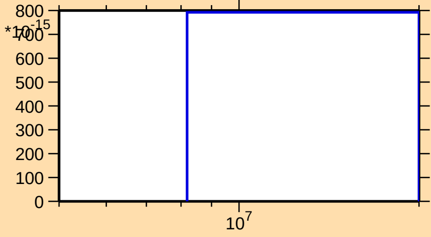
\sigma vs. E for ^{146}\text{Nd}(n,3n\alpha)
