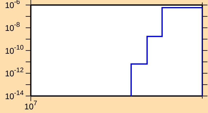
\sigma vs. E for ^{149}\text{Nd}(n,\text{nt})
