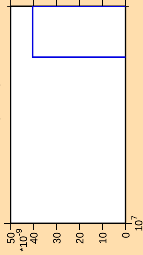
\Delta\sigma/\sigma vs. E for ^{149}\text{Nd}(\text{mt } 11)
