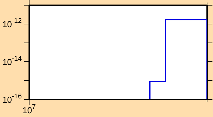
\sigma vs. E for ^{149}\text{Nd}(n,\text{He}3)
