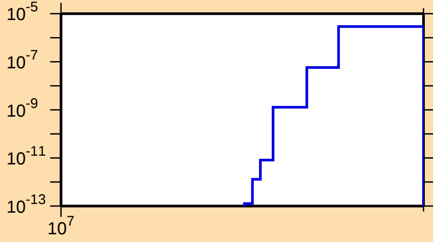
\sigma vs. E for ^{149}\text{Nd}(n,\text{nd})
