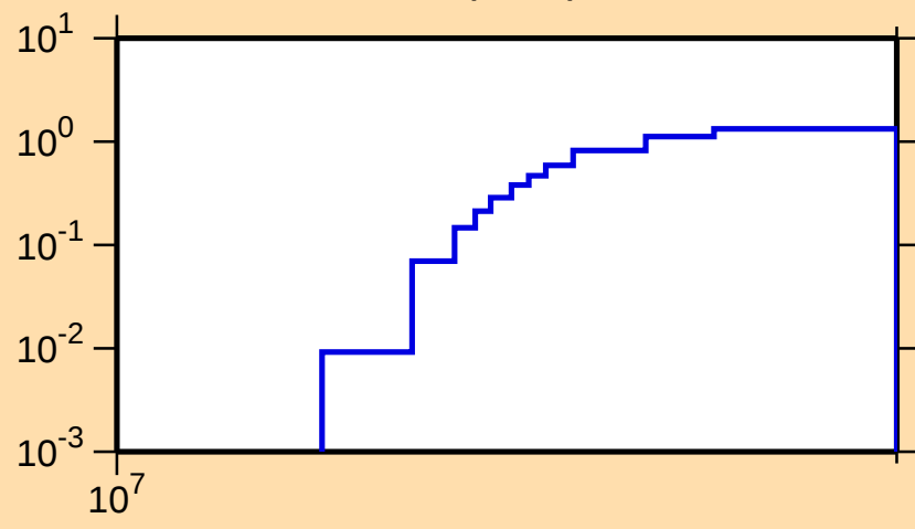
\sigma vs. E for ^{149}\text{Nd}(n,3n)
