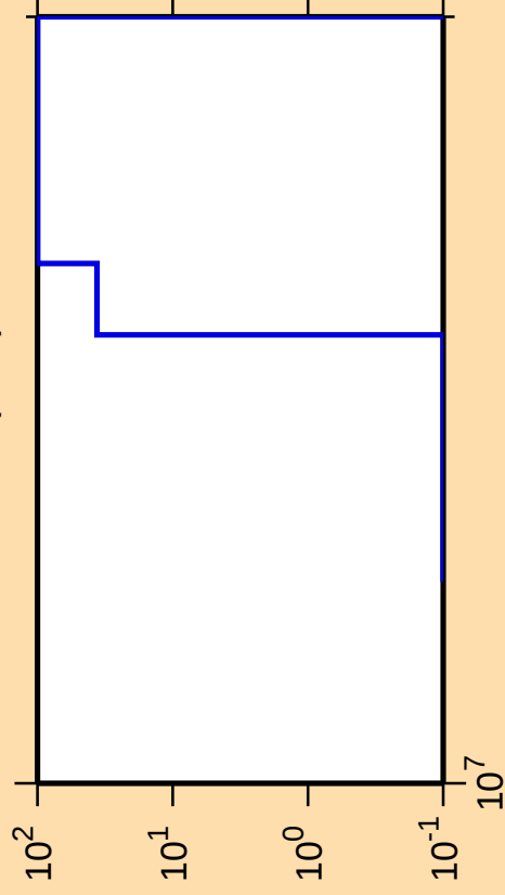
\Delta\sigma/\sigma vs. E for ^{149}\text{Nd}(n,\text{nt})
