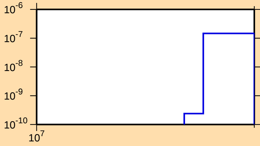
\sigma vs. E for ^{149}\text{Nd}(n,2np)
