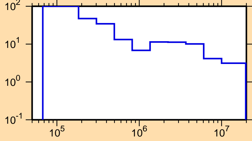
\Delta\sigma/\sigma vs. E for ^{149}\text{Nd}(n,\text{tot.})
