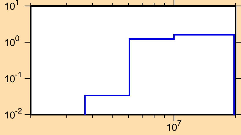
\sigma vs. E for ^{149}\text{Nd}(n,2n)
