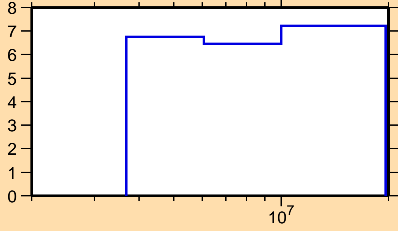
\Delta\sigma/\sigma vs. E for ^{149}\text{Nd}(n,\text{nonel.})
