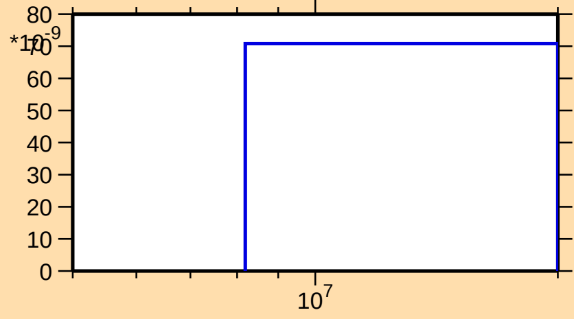
\sigma vs. E for ^{149}\text{Nd}(n,2n\alpha)
