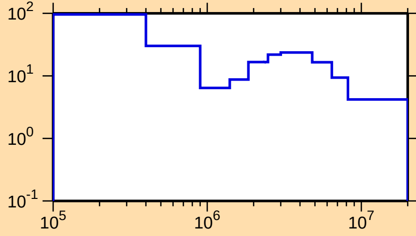
\Delta\sigma/\sigma vs. E for ^{149}\text{Nd}(n,\text{el.})
