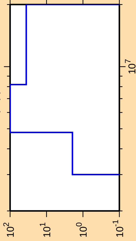
\Delta\sigma/\sigma vs. E for ^{149}\text{Nd}(n,p)
