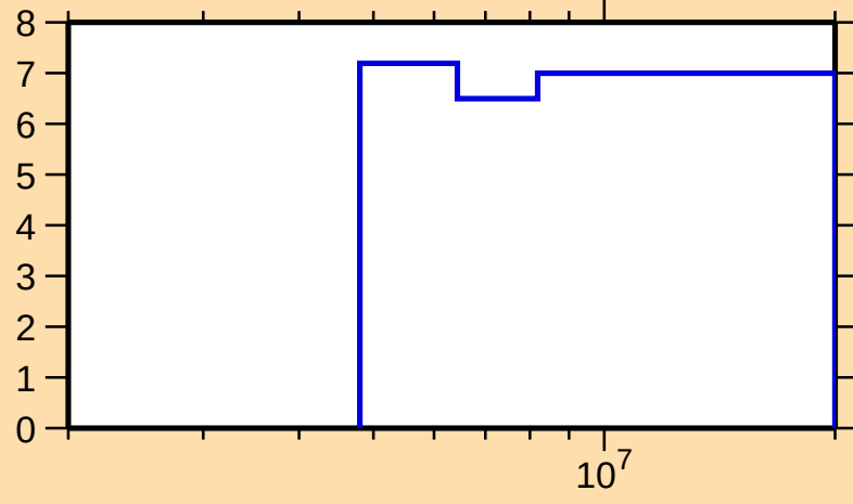
\Delta\sigma/\sigma vs. E for ^{149}\text{Nd}(n,\text{nonel.})
