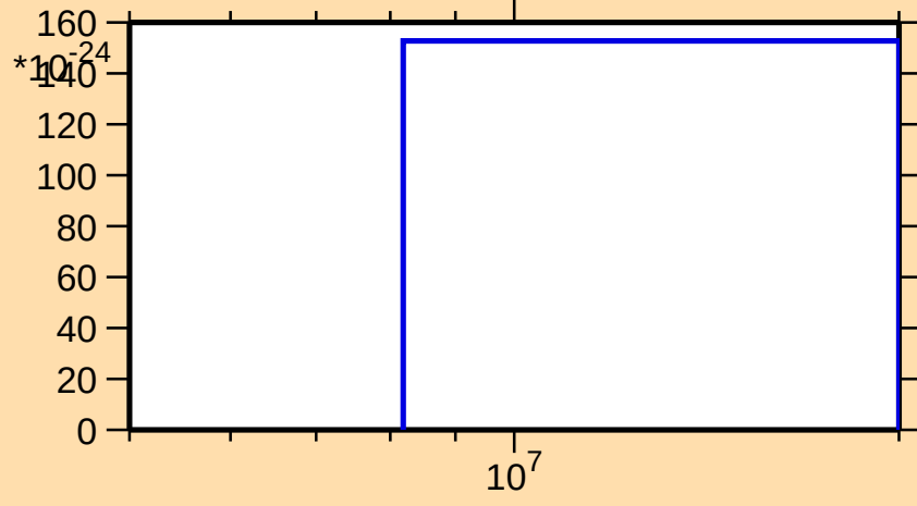
\sigma vs. E for ^{149}\text{Nd}(\text{mt } 11)
