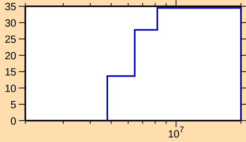
\Delta\sigma/\sigma vs. E for ^{149}\text{Nd}(n,\text{inel.})
