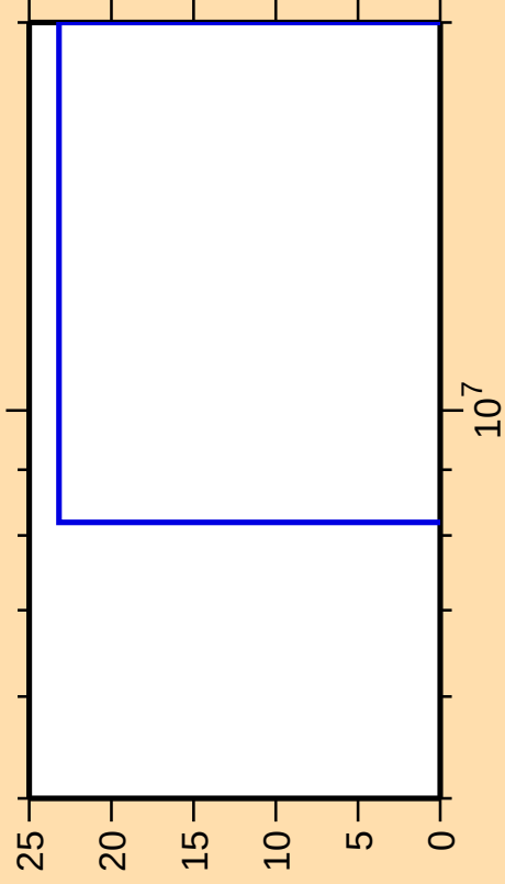
\Delta\sigma/\sigma vs. E for ^{149}\text{Nd}(n,3n)
