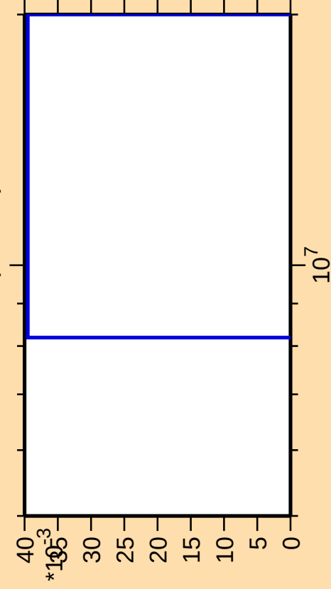
\Delta\sigma/\sigma vs. E for ^{149}\text{Nd}(n,\text{He}3)
