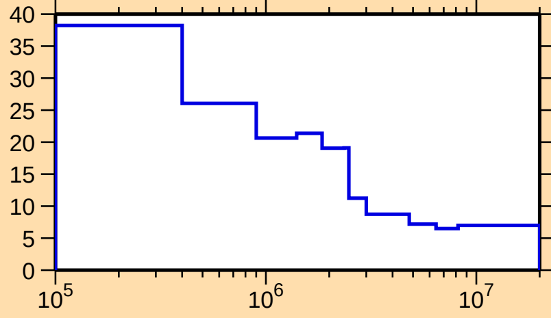
\Delta\sigma/\sigma vs. E for ^{149}\text{Nd}(n,\text{nonel.})
