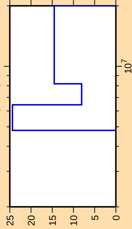
\Delta\sigma/\sigma vs. E for ^{149}\text{Nd}(n,2n)
