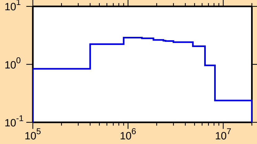
\sigma vs. E for ^{149}\text{Nd}(n,\text{inel.})
