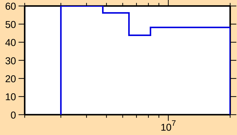
\Delta\sigma/\sigma vs. E for ^{149}\text{Nd}(n,n_1)
