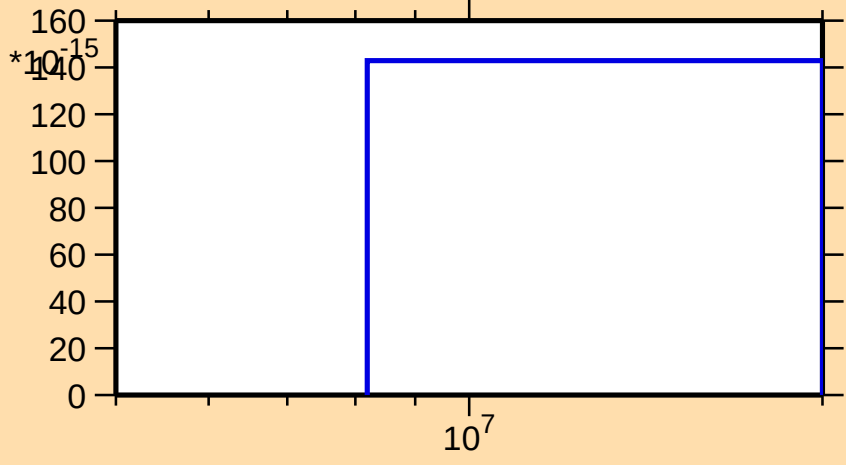
\sigma vs. E for ^{149}\text{Nd}(n,3n\alpha)
