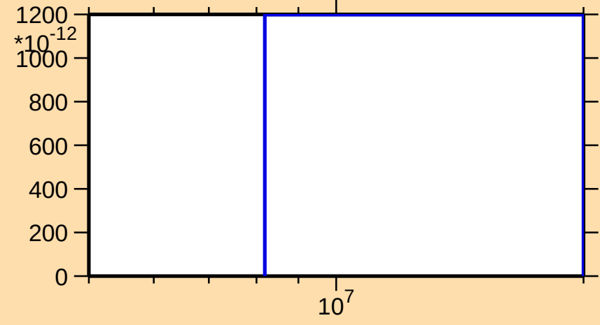
\sigma vs. E for ^{149}\text{Nd}(n,2np)
