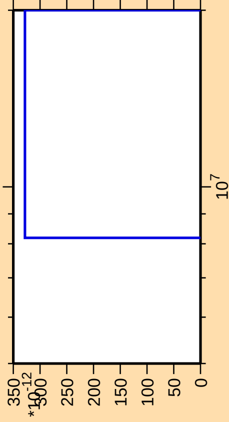
\Delta\sigma/\sigma vs. E for ^{149}\text{Nd}(\text{mt } 11)
