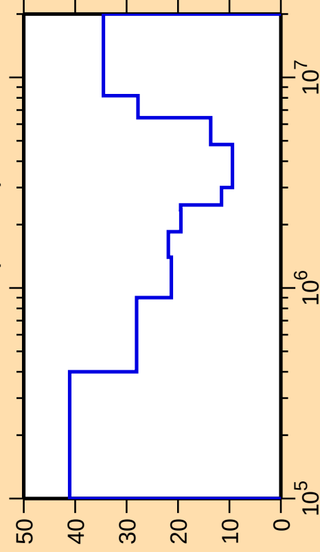
\Delta\sigma/\sigma vs. E for ^{149}\text{Nd}(n,\text{inel.})
