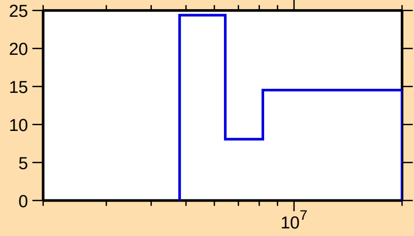
\Delta\sigma/\sigma vs. E for ^{149}\text{Nd}(n,2n)
