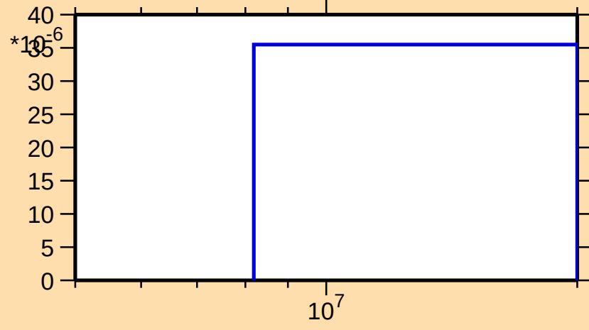
\sigma vs. E for ^{149}\text{Nd}(n,t)
