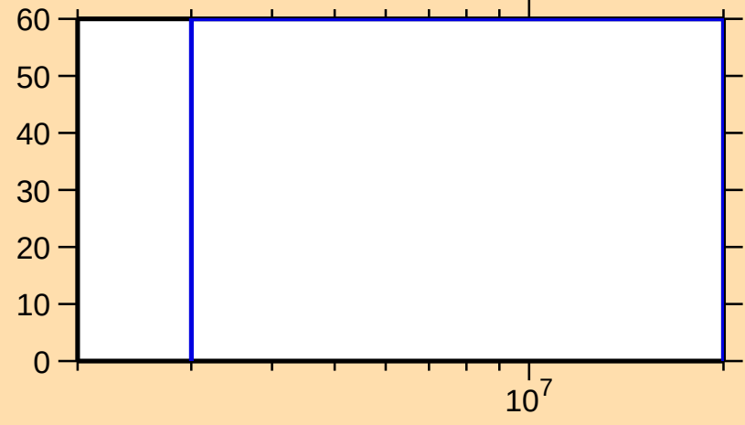
\Delta\sigma/\sigma vs. E for ^{149}\text{Nd}(n,\gamma)
