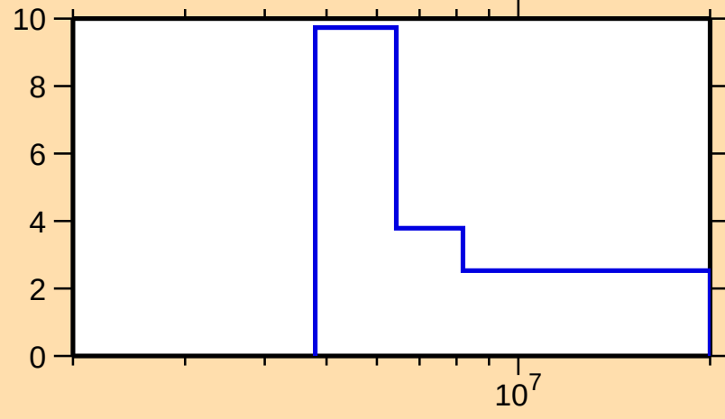
\Delta\sigma/\sigma vs. E for ^{149}\text{Nd}(n,\text{tot.})
