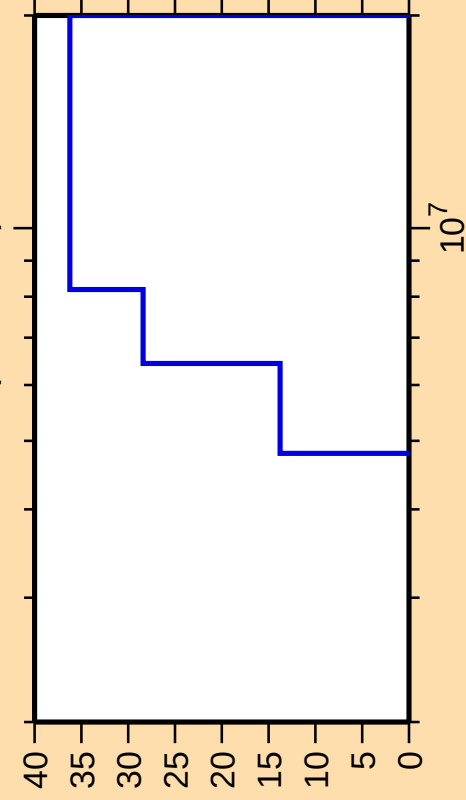
\Delta\sigma/\sigma vs. E for ^{149}\text{Nd}(n,n\text{cont.})
