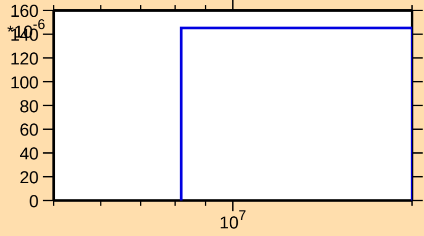
\sigma vs. E for ^{149}\text{Nd}(n,d)
