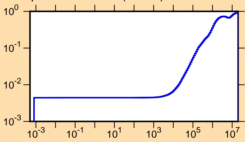
\mu vs. E for ^{152}\text{Nd}(\text{mt251})
