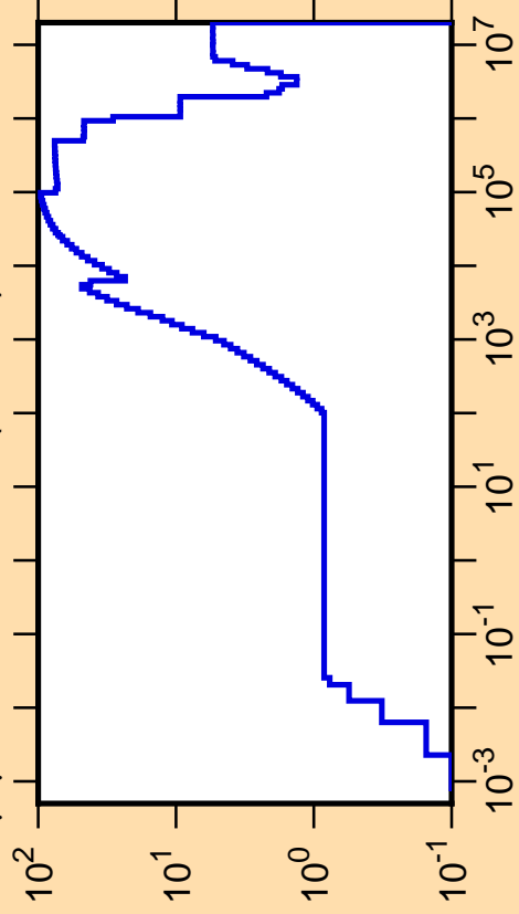
\Delta\mu/\mu vs. E for ^{152}\text{Nd}(\text{mt251})
