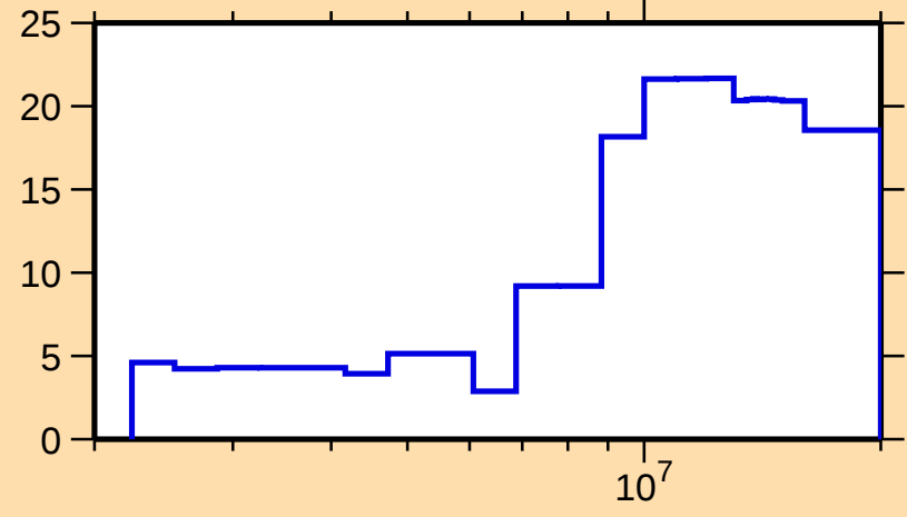
\Delta\sigma/\sigma vs. E for ^{152}\text{Nd}(\text{n},\text{inel.})
