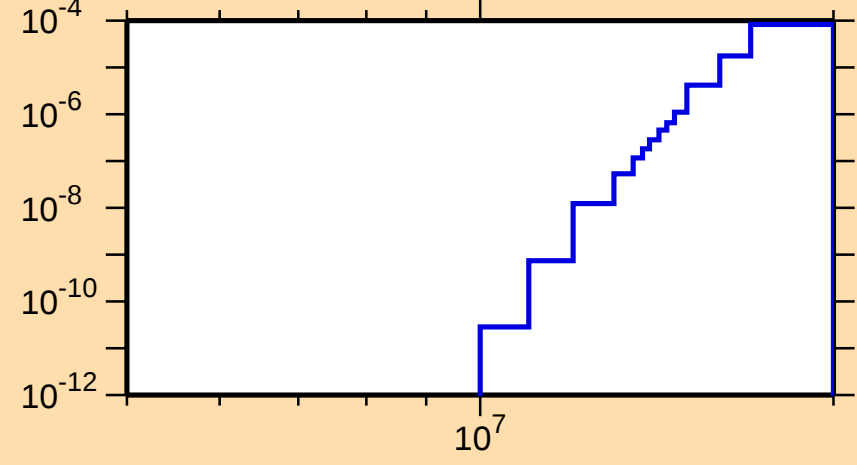
\sigma vs. E for ^{152}\text{Nd}(n,\alpha)
