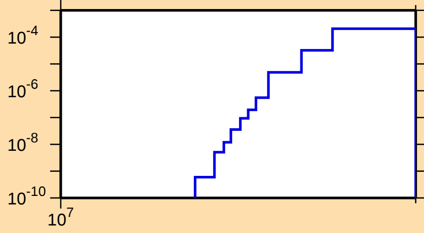
\sigma vs. E for ^{152}\text{Nd}(n,np)
