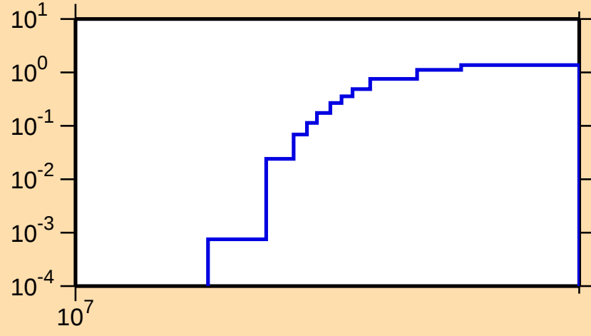
\sigma vs. E for ^{152}\text{Nd}(n,3n)
