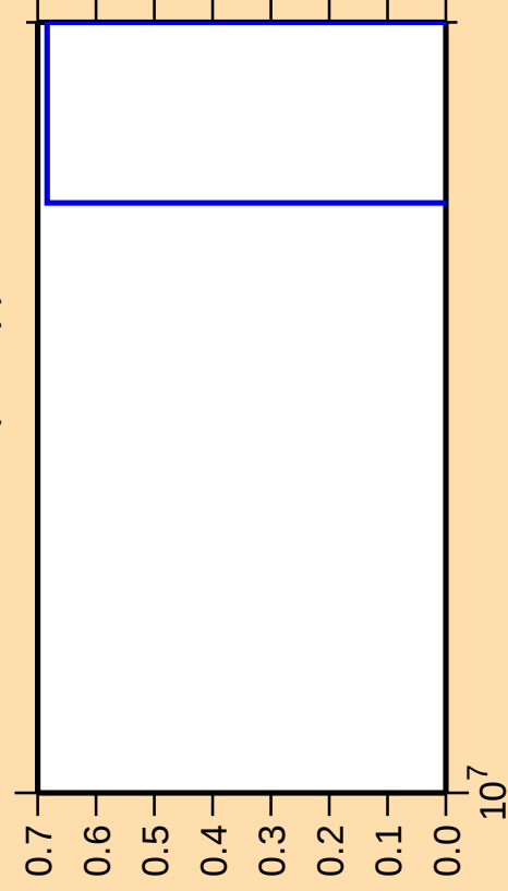
\Delta\sigma/\sigma vs. E for ^{152}\text{Nd}(n,2np)
