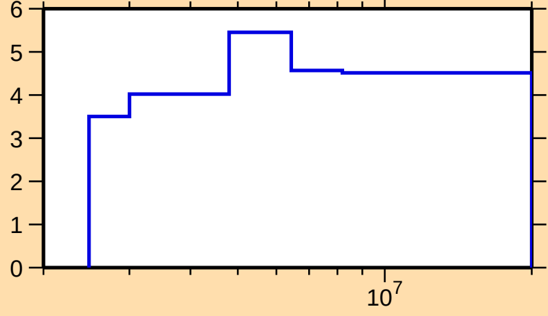
\Delta\sigma/\sigma vs. E for ^{152}\text{Nd}(\text{n},\text{nonel.})
