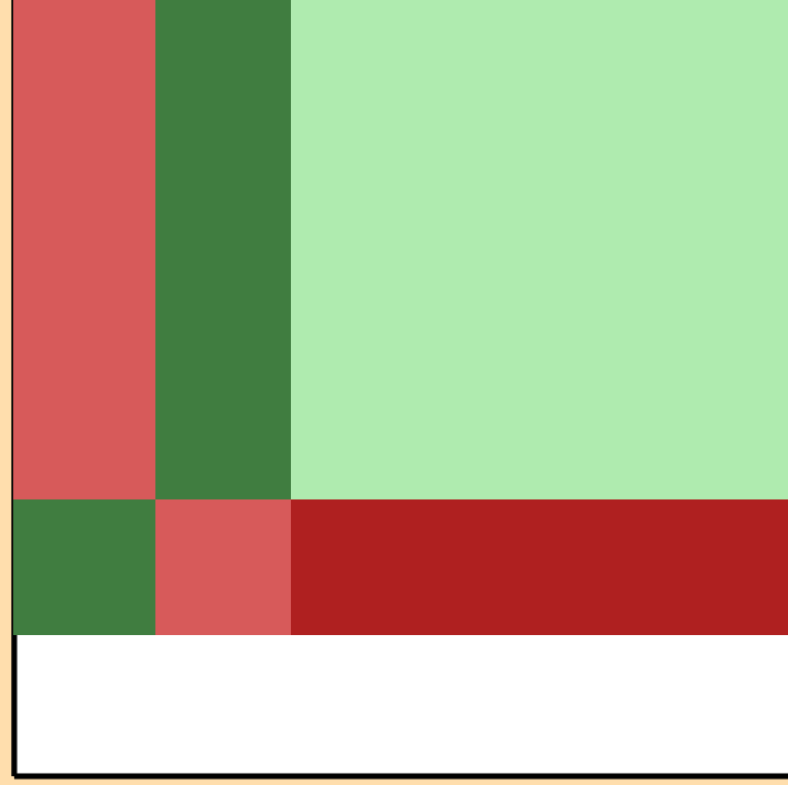
\Delta\sigma/\sigma vs. E for ^{152}\text{Nd}(n,\text{el.})
