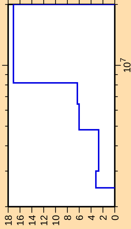
\Delta\sigma/\sigma vs. E for ^{152}\text{Nd}(\text{n},\text{ncont.})
