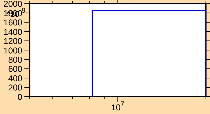
\sigma vs. E for ^{152}\text{Nd}(n,t)
