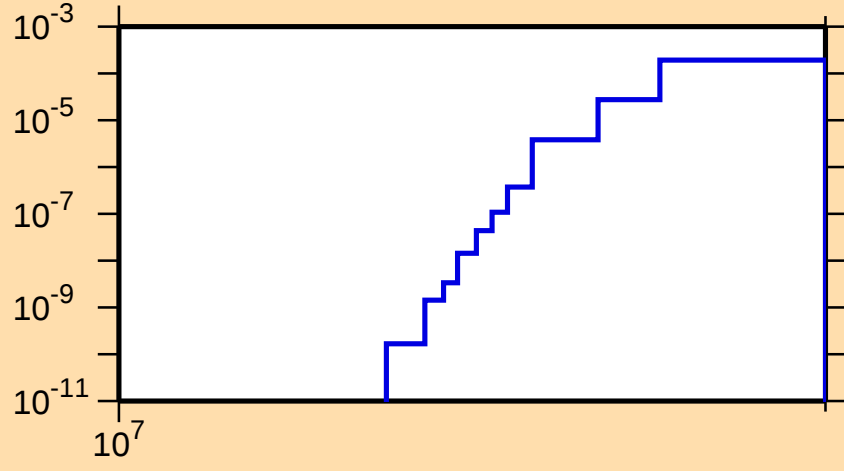
\sigma vs. E for ^{153}\text{Nd}(n,np)
