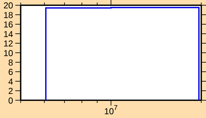
\Delta\sigma/\sigma vs. E for ^{153}\text{Nd}(n,2n)
