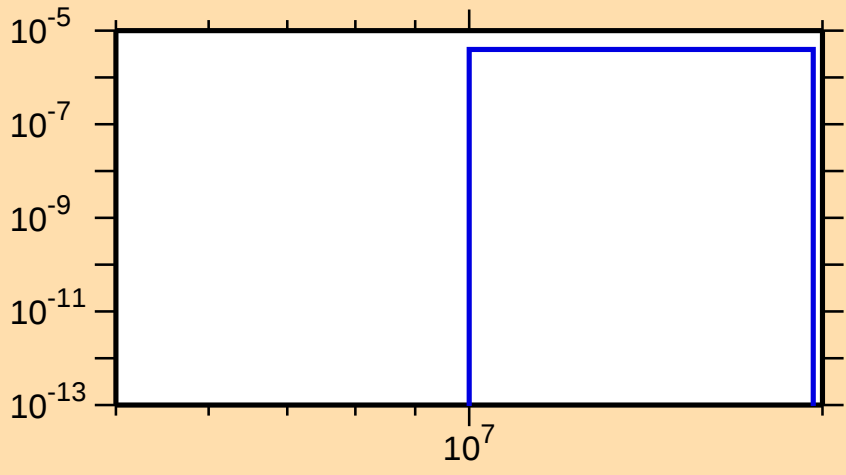
\sigma vs. E for ^{153}\text{Nd}(n,t)
