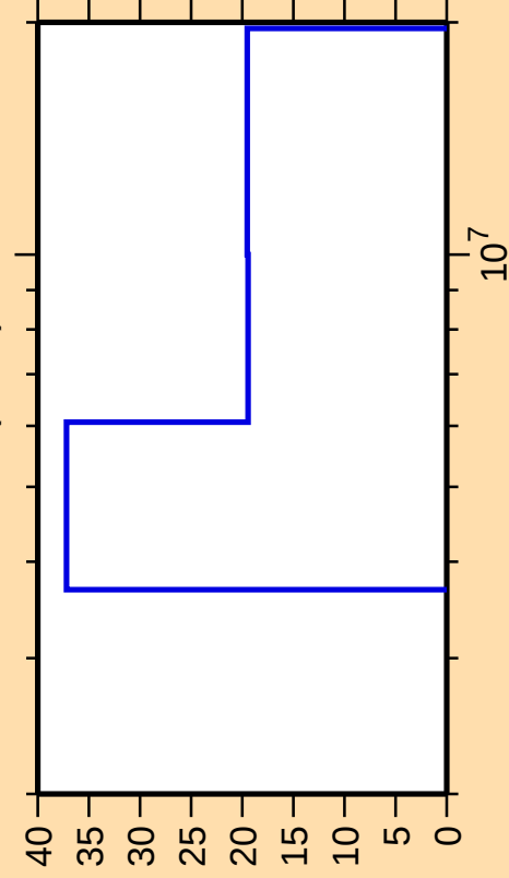
\Delta\sigma/\sigma vs. E for ^{153}\text{Nd}(n,2n)
