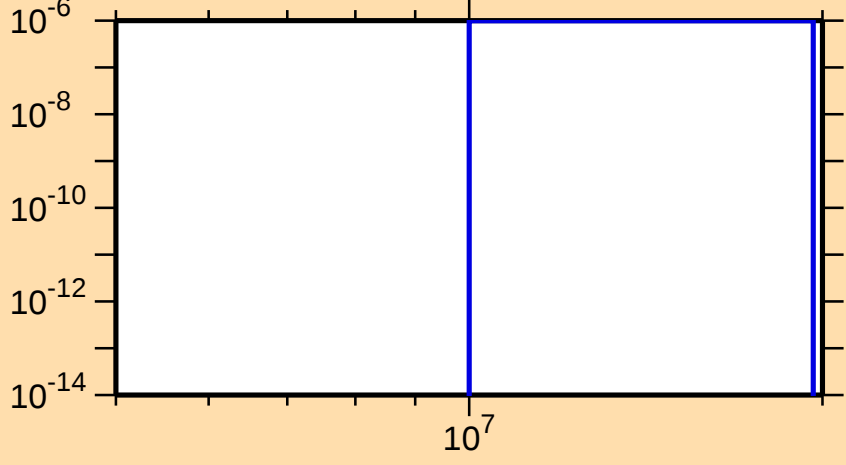
\sigma vs. E for ^{153}\text{Nd}(n,\alpha)
