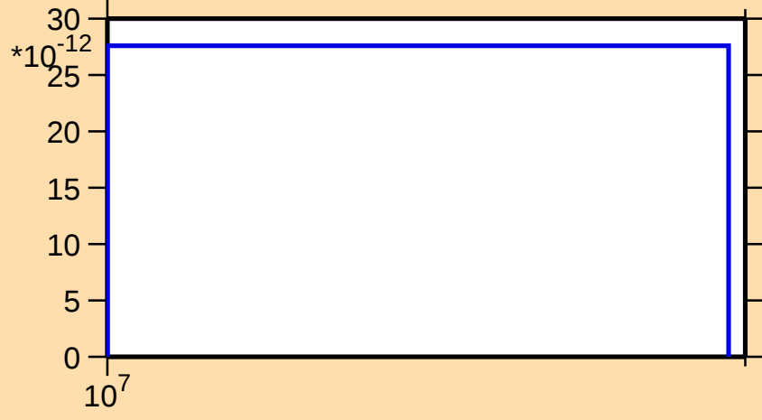
\sigma vs. E for ^{153}\text{Nd}(n,\text{nt})
