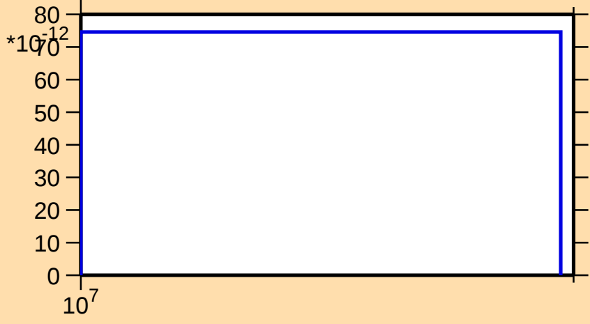
\sigma vs. E for ^{153}\text{Nd}(n,2n\alpha)
