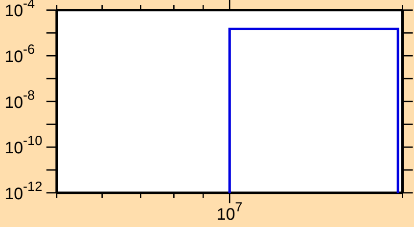
\sigma vs. E for ^{153}\text{Nd}(n,d)
