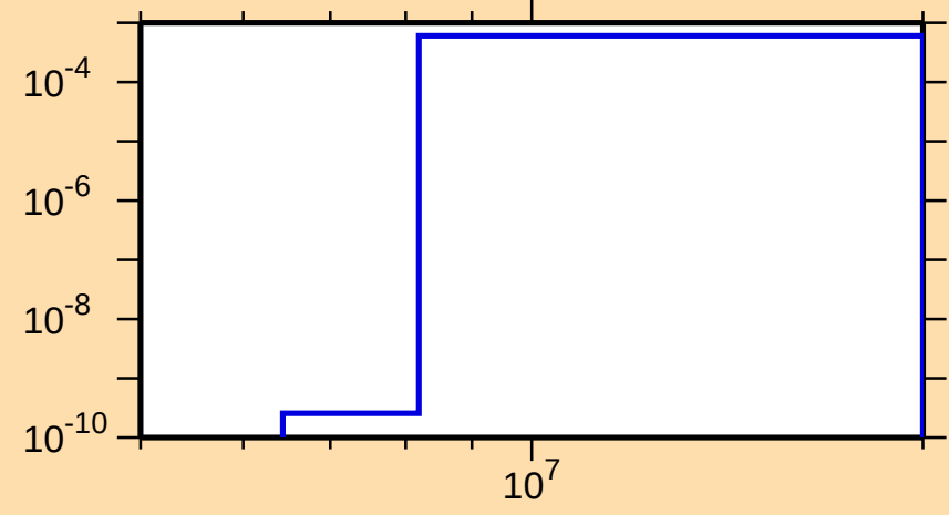
\sigma vs. E for ^{153}\text{Nd}(n,p)
