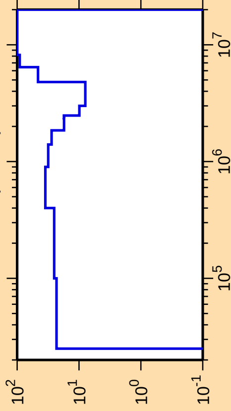
\Delta\sigma/\sigma vs. E for ^{153}\text{Nd}(n,\text{inel.})
