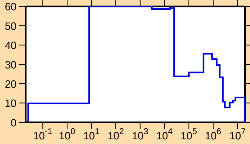
\Delta\sigma/\sigma vs. E for ^{153}\text{Nd}(n,\text{nonel.})
