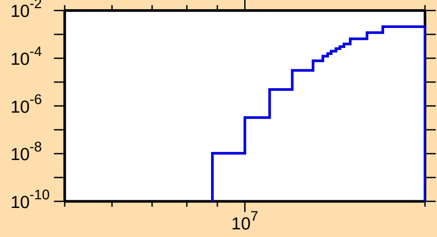
\sigma vs. E for ^{155}\text{Nd}(n,p)
