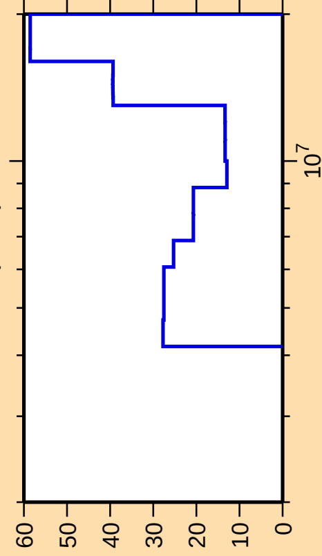
\Delta\sigma/\sigma vs. E for ^{155}\text{Nd}(n,2n)
