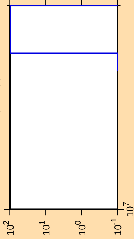
\Delta\sigma/\sigma vs. E for ^{155}\text{Nd}(n,2np)
