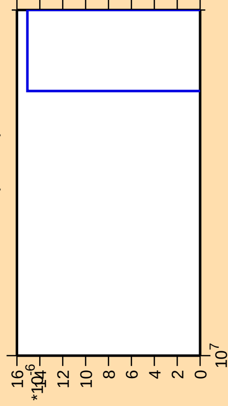
\Delta\sigma/\sigma vs. E for ^{155}\text{Nd}(\text{mt } 11)
