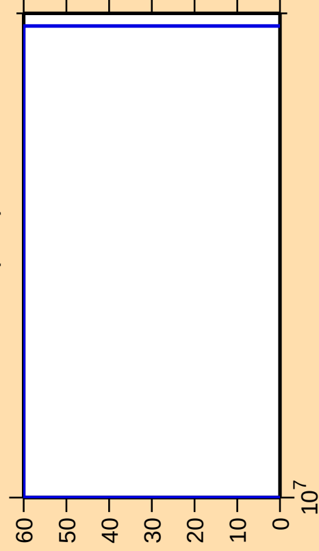
\Delta\sigma/\sigma vs. E for ^{155}\text{Nd}(n,\text{nt})
