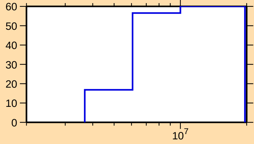
\Delta\sigma/\sigma vs. E for ^{155}\text{Nd}(n,n\text{cont.})
