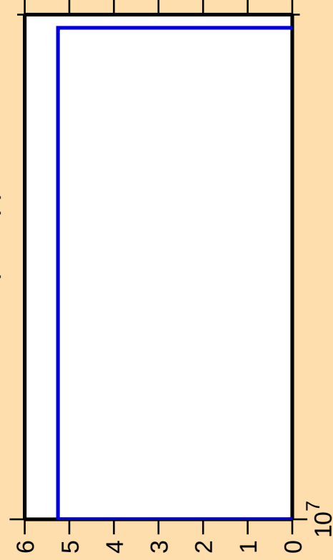
\Delta\sigma/\sigma vs. E for ^{155}\text{Nd}(n,2np)
