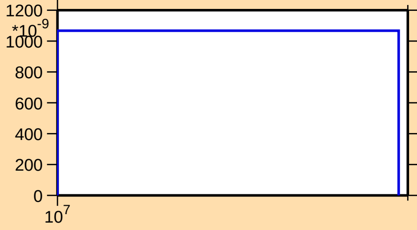
\sigma vs. E for ^{155}\text{Nd}(n,np)
