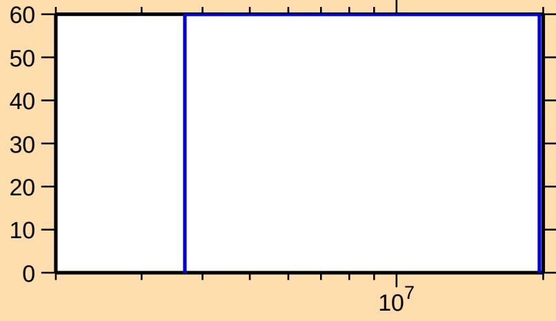
\Delta\sigma/\sigma vs. E for ^{155}\text{Nd}(n,\gamma)
