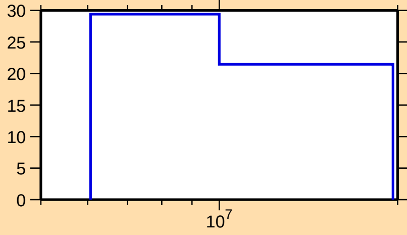
\Delta\sigma/\sigma vs. E for ^{155}\text{Nd}(n,\text{el.})
