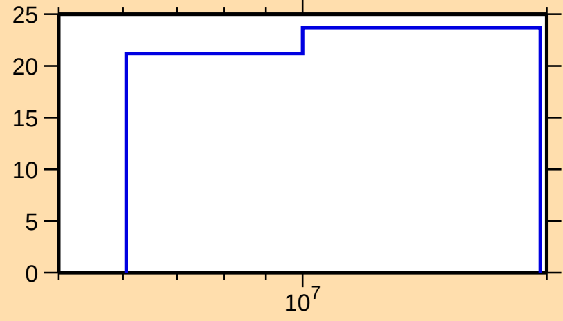
\Delta\sigma/\sigma vs. E for ^{155}\text{Nd}(n,2n)
