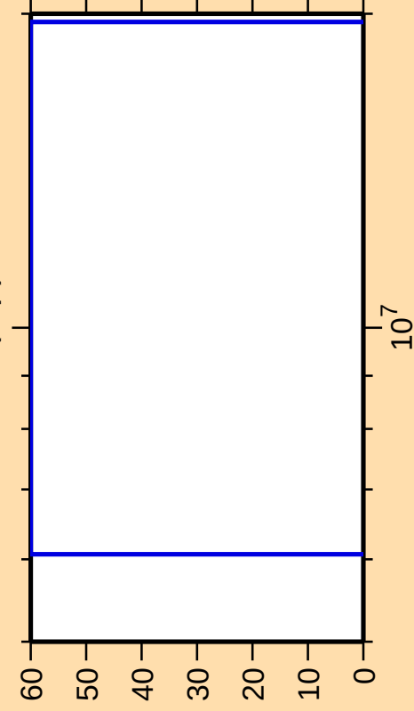
\Delta\sigma/\sigma vs. E for ^{155}\text{Nd}(n,p)
