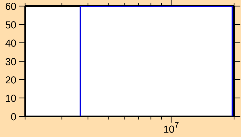
\Delta\sigma/\sigma vs. E for ^{155}\text{Nd}(n,n_1)
