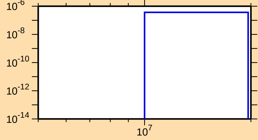
\sigma vs. E for ^{155}\text{Nd}(n,\alpha)
