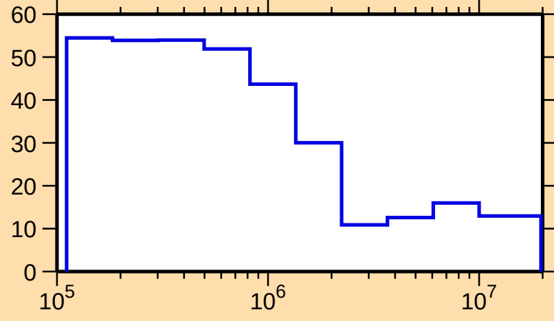
\Delta\sigma/\sigma vs. E for ^{155}\text{Nd}(n,n\text{onel.})
