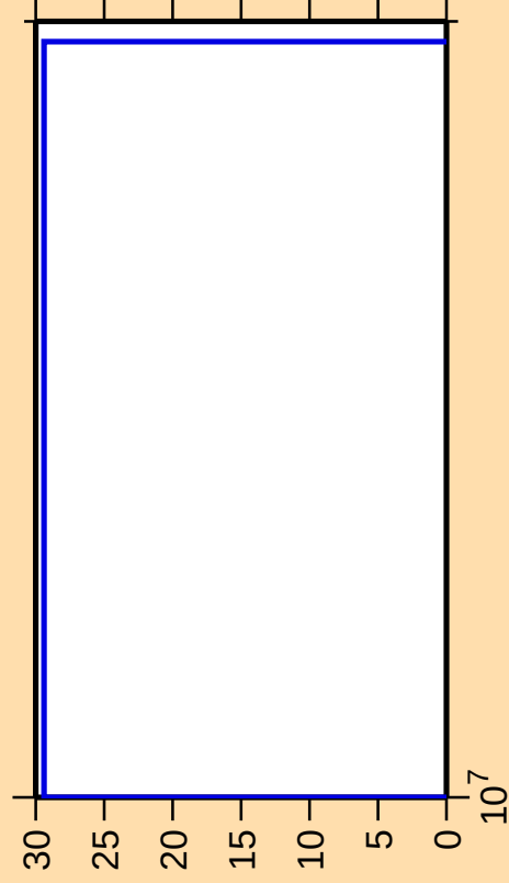
\Delta\sigma/\sigma vs. E for ^{155}\text{Nd}(n,3n)
