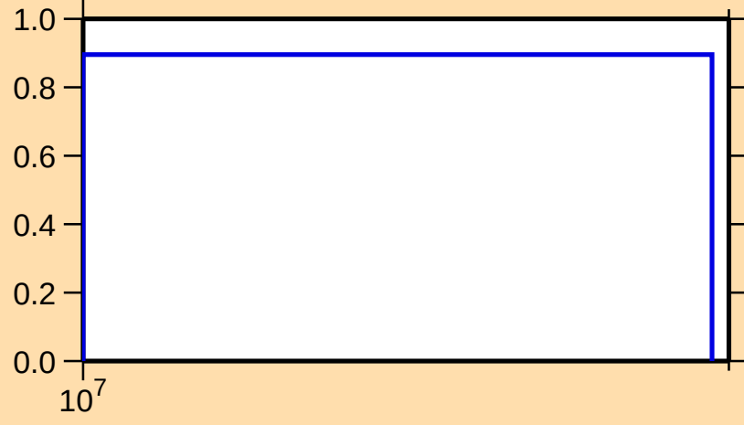
\sigma vs. E for ^{155}\text{Nd}(n,3n)
