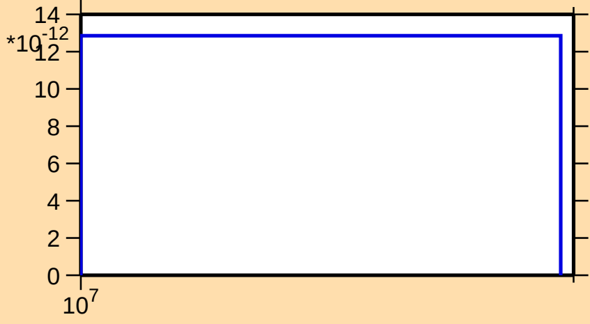
\sigma vs. E for ^{155}\text{Nd}(n,2n\alpha)
