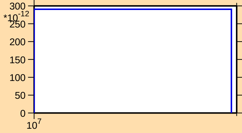
\sigma vs. E for ^{155}\text{Nd}(n,\text{nd})
