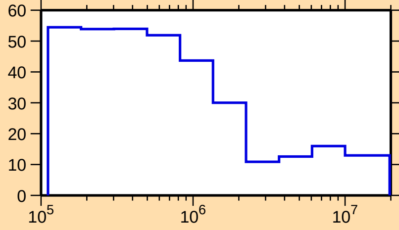
\Delta\sigma/\sigma vs. E for ^{155}\text{Nd}(n,\text{nonel.})
