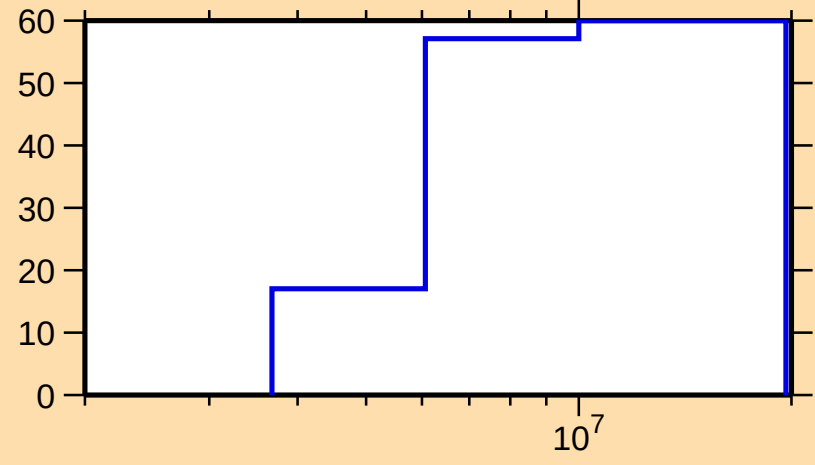
\Delta\sigma/\sigma vs. E for ^{155}\text{Nd}(n,\text{inel.})
