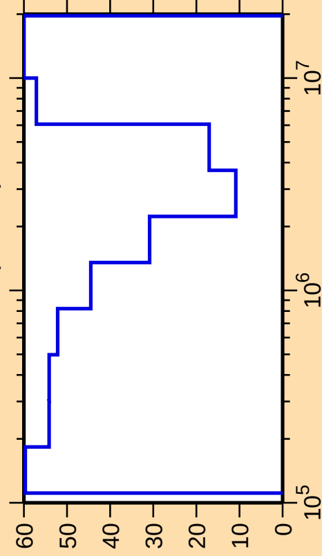
\Delta\sigma/\sigma vs. E for ^{155}\text{Nd}(n,\text{inel.})
