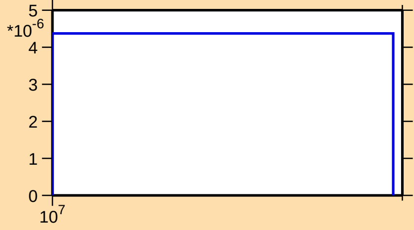
\sigma vs. E for ^{155}\text{Nd}(n,d)
