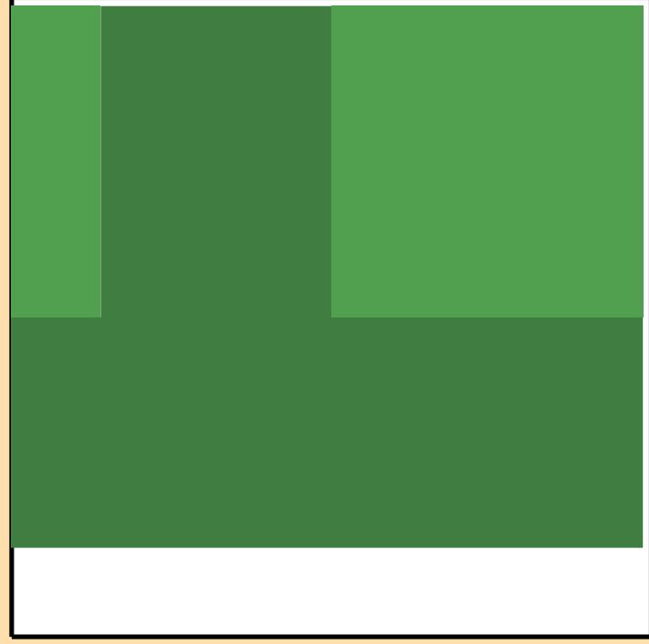
\Delta\sigma/\sigma vs. E for ^{155}\text{Nd}(n,\text{nonel.})
