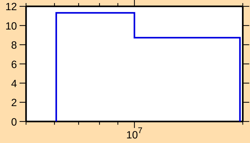
\Delta\sigma/\sigma vs. E for ^{155}\text{Nd}(n,\text{tot.})
