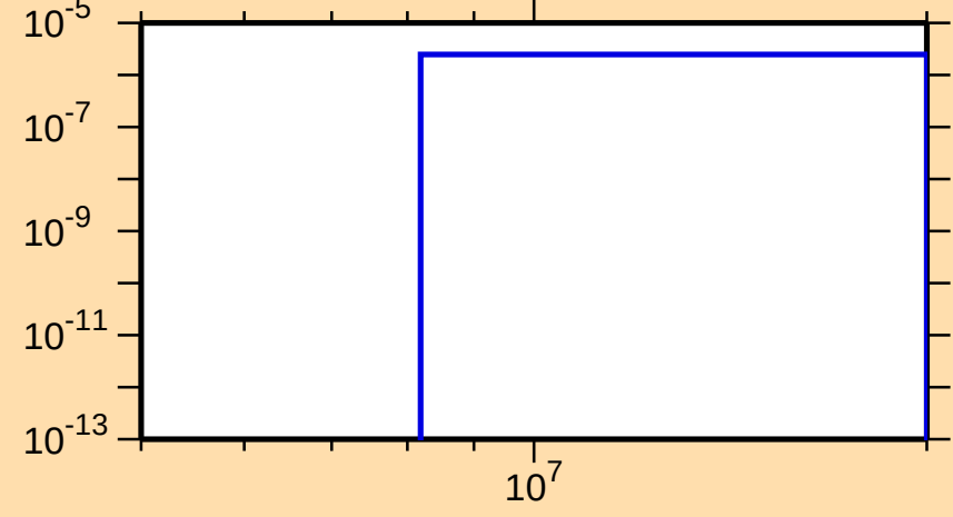
\sigma vs. E for ^{155}\text{Nd}(n,t)
