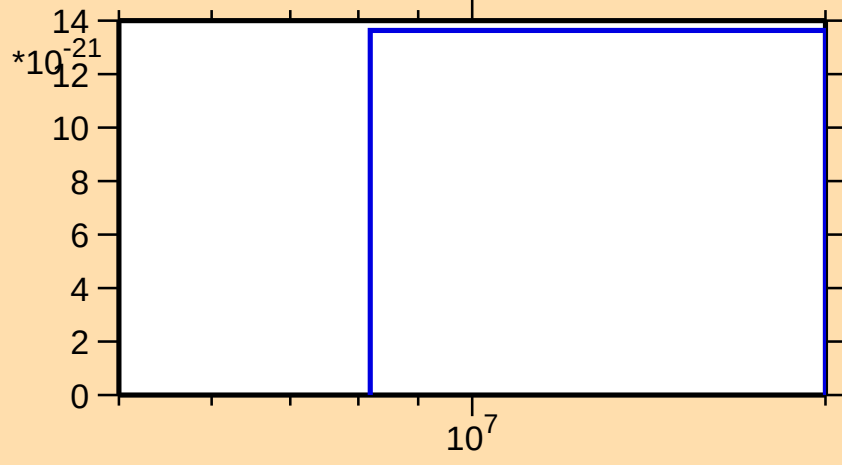
\sigma vs. E for ^{155}\text{Nd}(\text{mt } 11)
