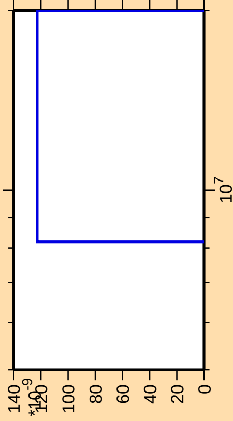
\Delta\sigma/\sigma vs. E for ^{155}\text{Nd}(\text{mt } 11)
