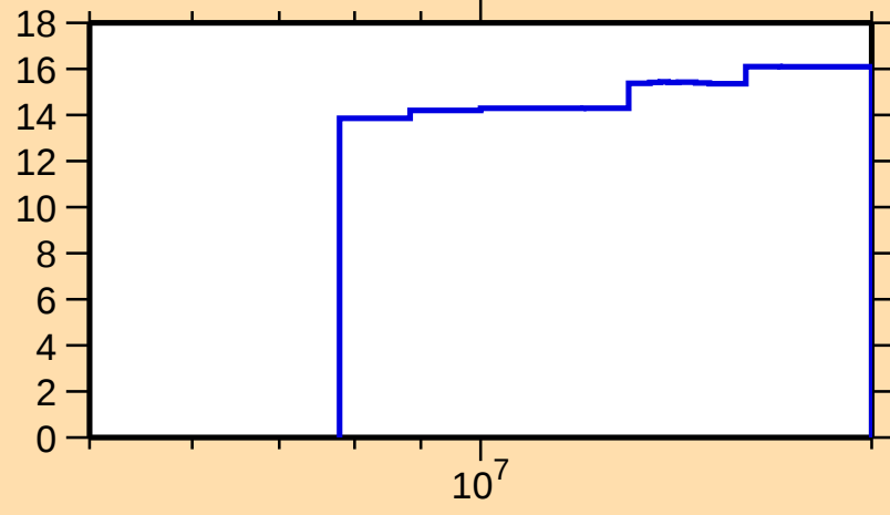
\Delta\sigma/\sigma vs. E for ^{156}\text{Nd}(n,\text{nonel.})
