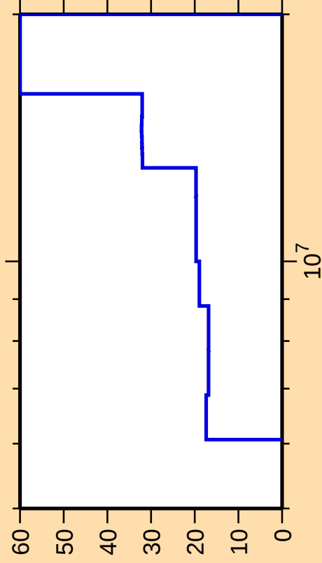
\Delta\sigma/\sigma vs. E for ^{156}\text{Nd}(n,2n)
