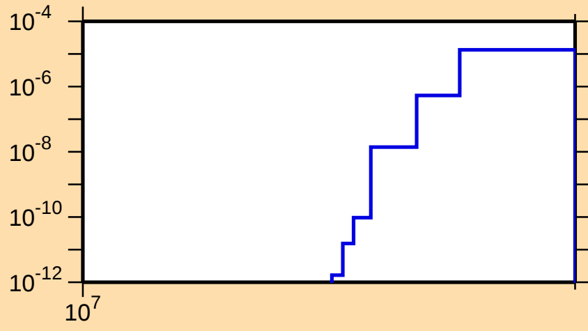
\sigma vs. E for ^{156}\text{Nd}(n,np)
