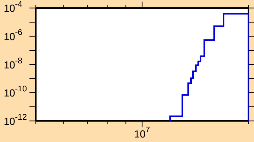
\sigma vs. E for ^{156}\text{Nd}(n,t)
