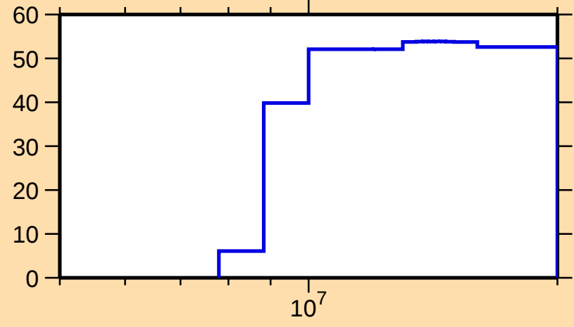
\Delta\sigma/\sigma vs. E for ^{156}\text{Nd}(n,n\text{cont.})
