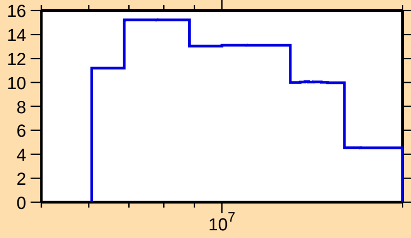
\Delta\sigma/\sigma vs. E for ^{156}\text{Nd}(n,\text{tot.})
