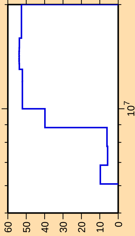
\Delta\sigma/\sigma vs. E for ^{156}\text{Nd}(n,n\text{cont.})
