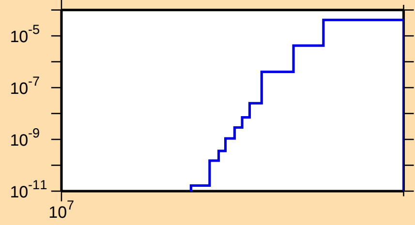
\sigma vs. E for ^{156}\text{Nd}(n,d)
