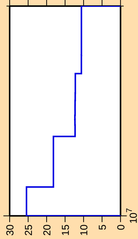
\Delta\sigma/\sigma vs. E for ^{156}\text{Nd}(n,3n)
