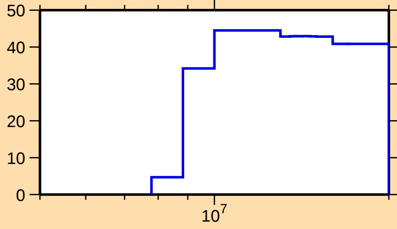
\Delta\sigma/\sigma vs. E for ^{156}\text{Nd}(n,\text{inel.})
