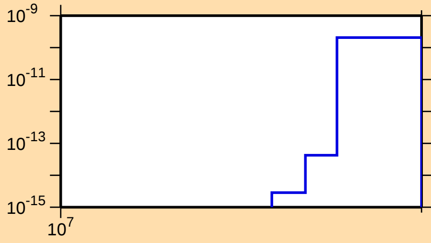
\sigma vs. E for ^{156}\text{Nd}(n,\text{nd})
