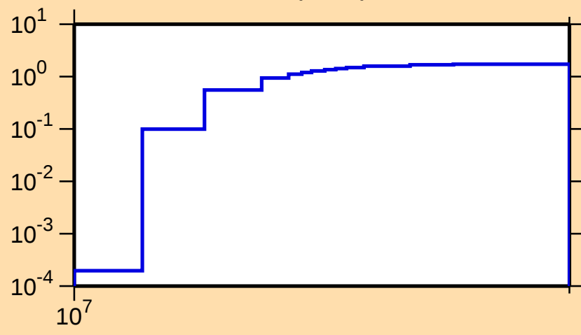
\sigma vs. E for ^{156}\text{Nd}(n,3n)
