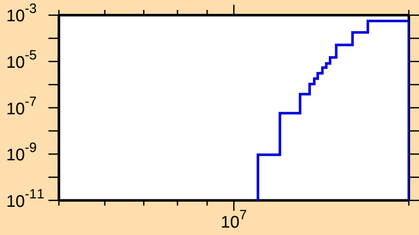
\sigma vs. E for ^{156}\text{Nd}(n,p)
