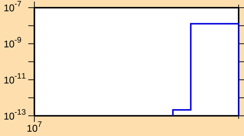
\sigma vs. E for ^{156}\text{Nd}(n,\text{nt})
