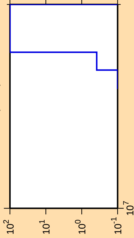
\Delta\sigma/\sigma vs. E for ^{156}\text{Nd}(n,\text{nd})
