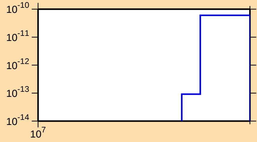
\sigma vs. E for ^{156}\text{Nd}(n,2n\alpha)
