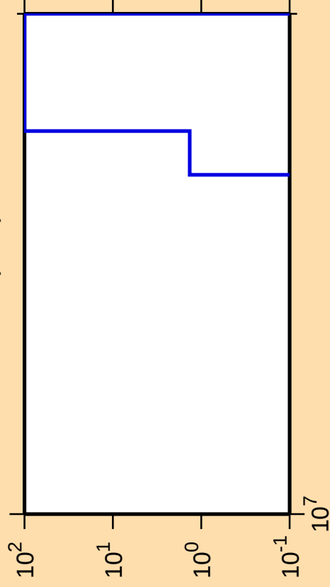
\Delta\sigma/\sigma vs. E for ^{156}\text{Nd}(n,\text{nt})
