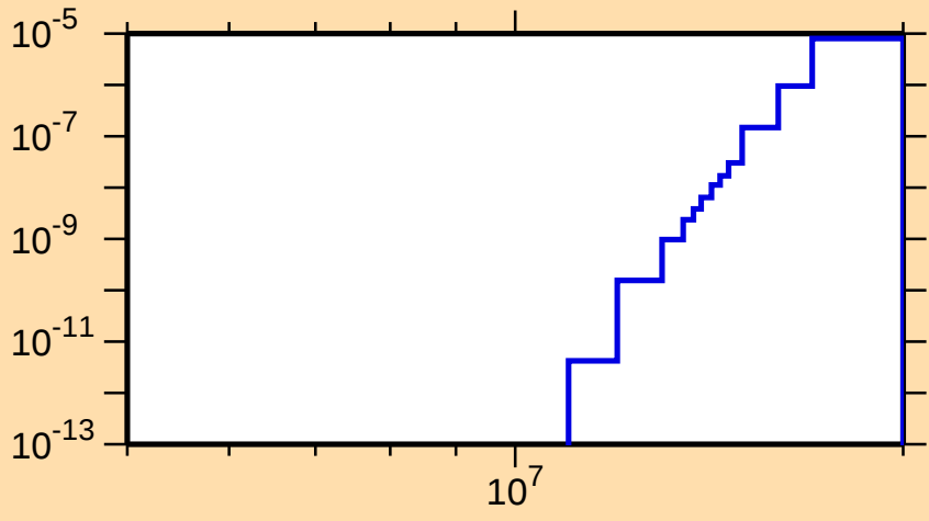
\sigma vs. E for ^{156}\text{Nd}(n,\alpha)
