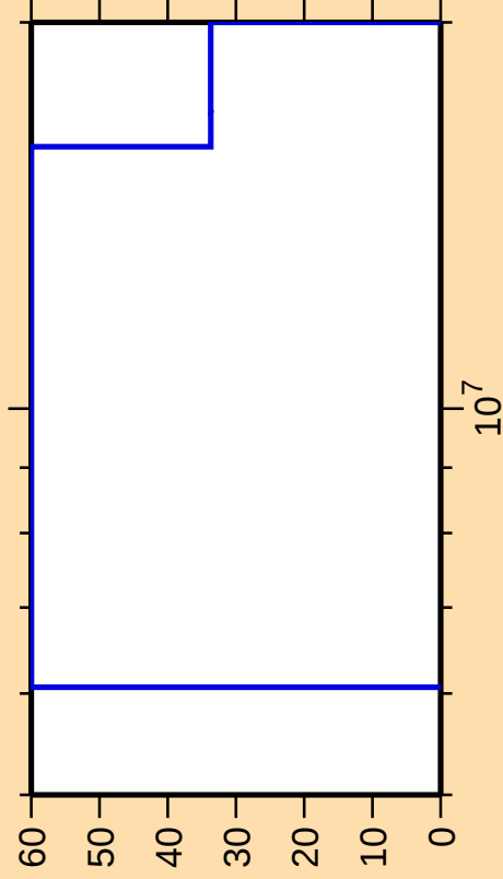
\Delta\sigma/\sigma vs. E for ^{156}\text{Nd}(n,\gamma)
