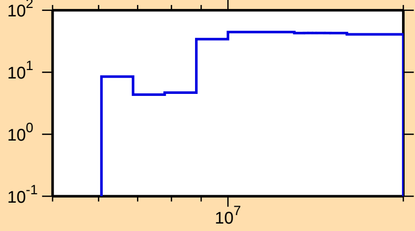
\Delta\sigma/\sigma vs. E for ^{156}\text{Nd}(n,\text{inel.})
