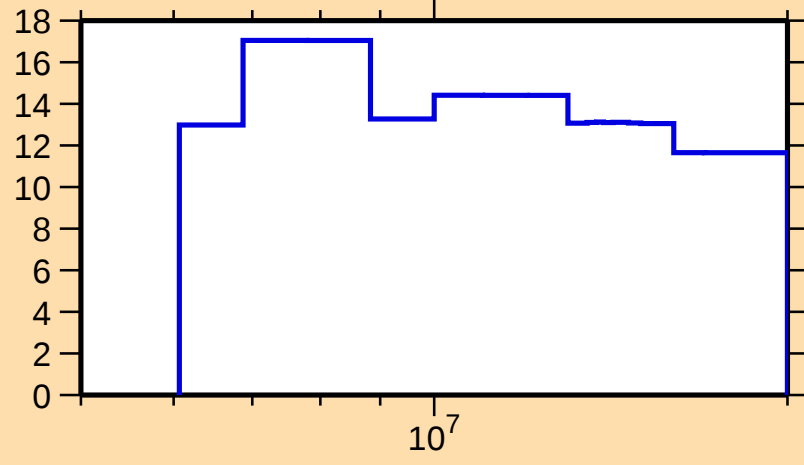
\Delta\sigma/\sigma vs. E for ^{156}\text{Nd}(n,\text{el.})
