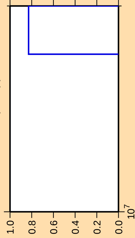
\Delta\sigma/\sigma vs. E for ^{156}\text{Nd}(n,2np)
