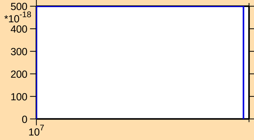
\sigma vs. E for ^{156}\text{Nd}(n,2np)
