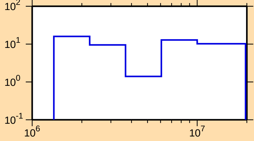
\Delta\sigma/\sigma vs. E for ^{156}\text{Nd}(n,\text{tot.})
