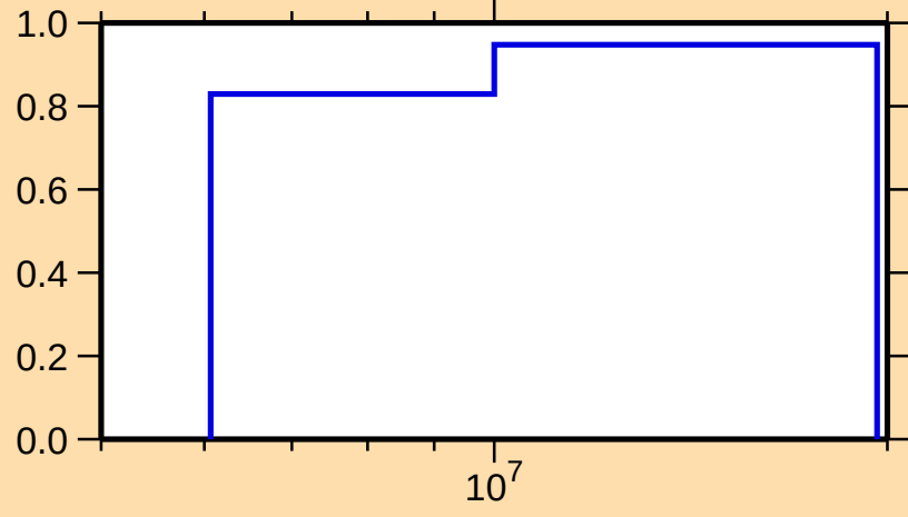
\sigma vs. E for ^{156}\text{Nd}(n,2n)
