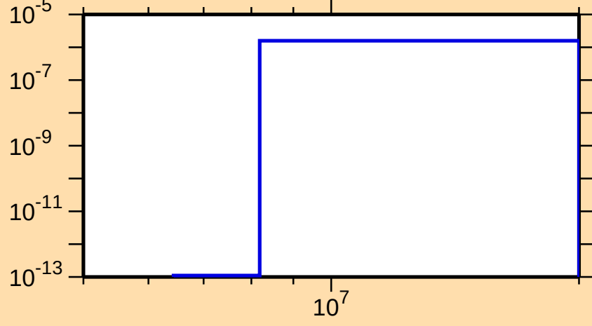
\sigma vs. E for ^{156}\text{Nd}(n,\alpha)
