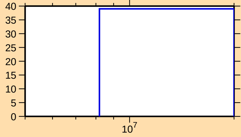
\Delta\sigma/\sigma vs. E for ^{156}\text{Nd}(n,ncont.)
