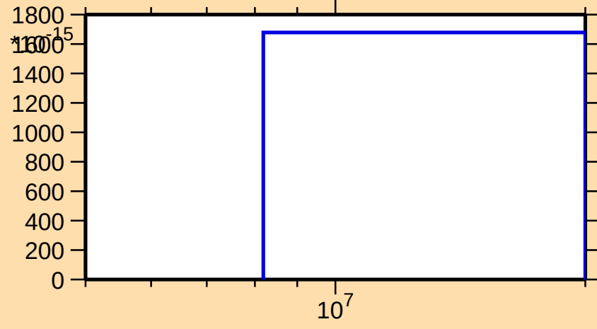
\sigma vs. E for ^{156}\text{Nd}(n,\text{nd})
