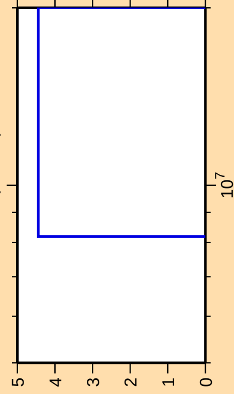
\Delta\sigma/\sigma vs. E for ^{156}\text{Nd}(n,2n\alpha)
