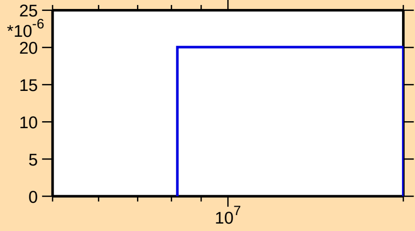
\sigma vs. E for ^{156}\text{Nd}(n,p)
