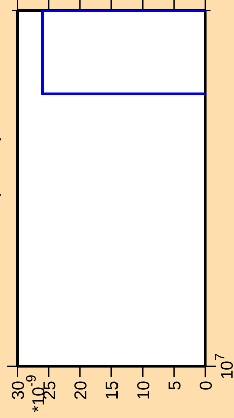
\Delta\sigma/\sigma vs. E for ^{157}\text{Nd}(\text{mt } 11)
