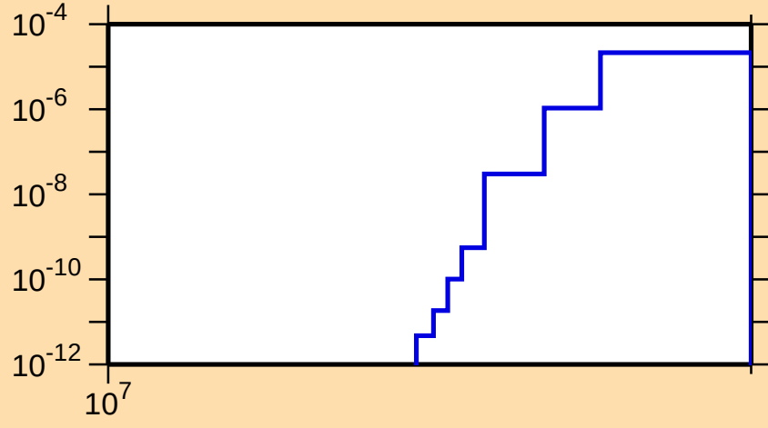
\sigma vs. E for ^{157}\text{Nd}(n,np)
