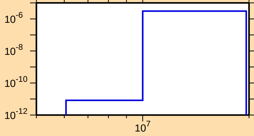
\sigma vs. E for ^{157}\text{Nd}(n,\alpha)
