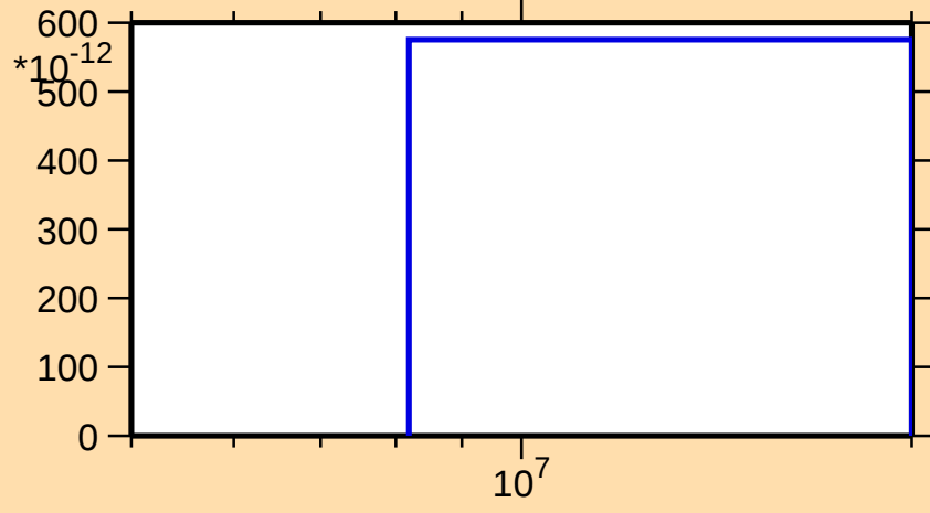
\sigma vs. E for ^{157}\text{Nd}(n,\text{nt})
