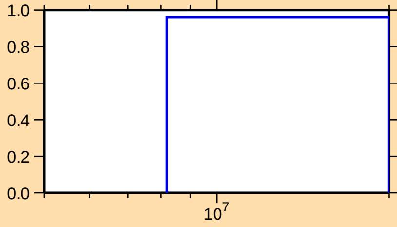
\sigma vs. E for ^{157}\text{Nd}(n,3n)
