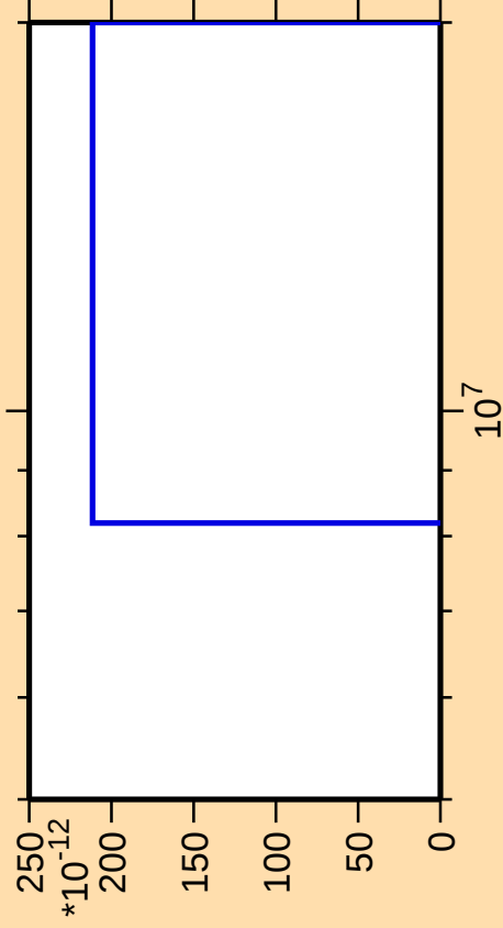
\Delta\sigma/\sigma vs. E for ^{157}\text{Nd}(\text{mt } 11)
