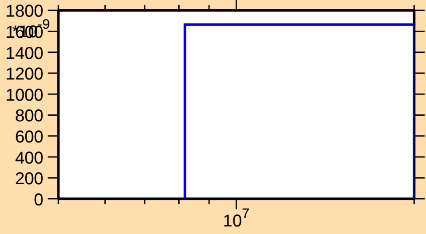
\sigma vs. E for ^{157}\text{Nd}(n,d)
