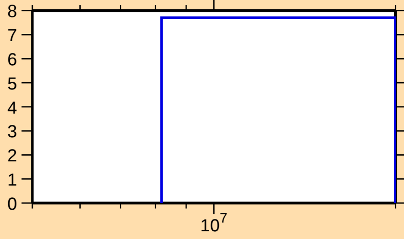
\Delta\sigma/\sigma vs. E for ^{157}\text{Nd}(n,\text{el.})
