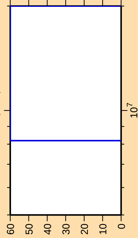
\Delta\sigma/\sigma vs. E for ^{157}\text{Nd}(n,\text{nt})
