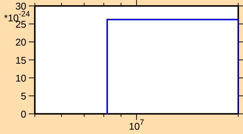
\sigma vs. E for ^{157}\text{Nd}(\text{mt } 11)
