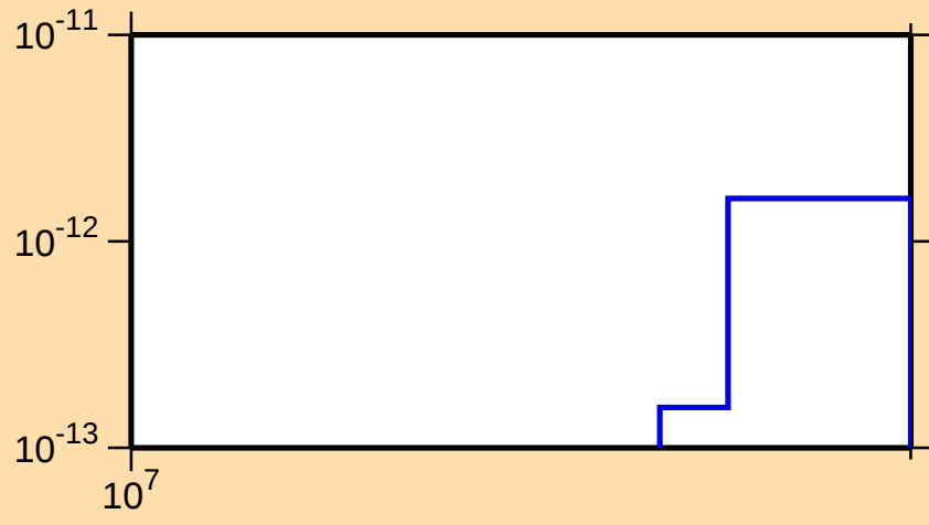
\sigma vs. E for ^{252}\text{No}(n,\text{pd})
