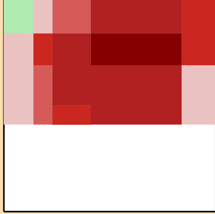
\Delta\sigma/\sigma vs. E for ^{252}\text{No}(n,\text{tot.})
