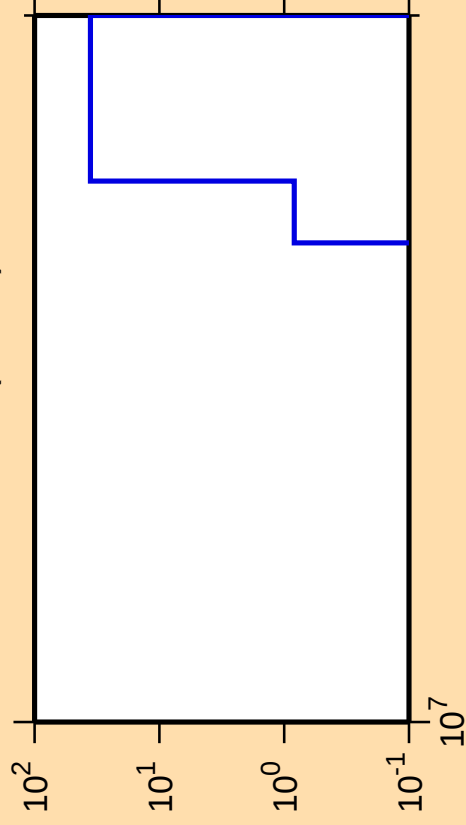
\Delta\sigma/\sigma vs. E for ^{252}\text{No}(\text{mt } 34)
