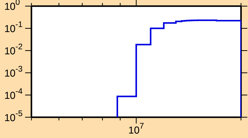
\sigma vs. E for ^{252}\text{No}(n,2n\alpha)
