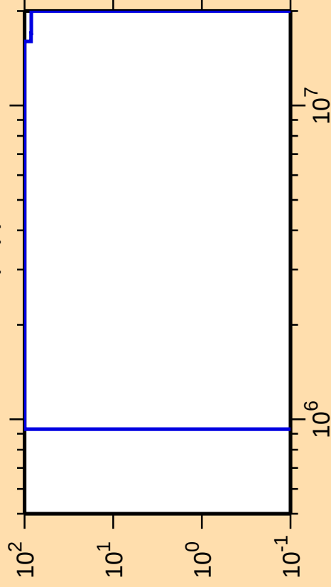
\Delta\sigma/\sigma vs. E for ^{252}\text{No}(n,p)
