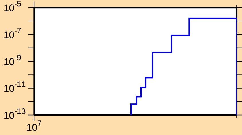
\sigma vs. E for ^{252}\text{No}(n,2np)
