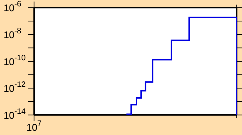
\sigma vs. E for ^{252}\text{No}(n,nt)
