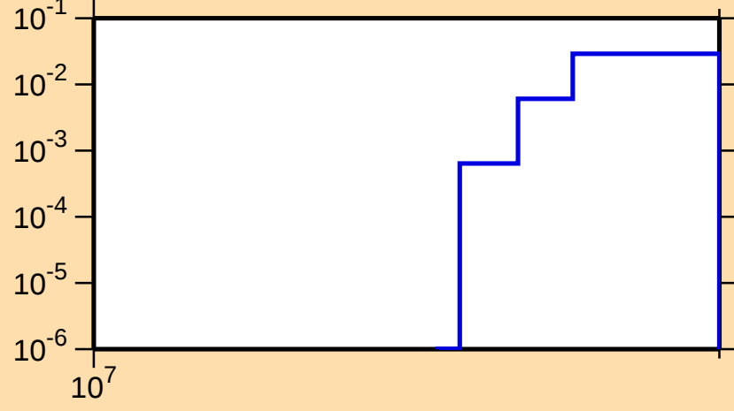
\sigma vs. E for ^{252}\text{No}(n,3n)
