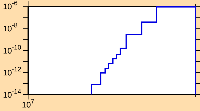
\sigma vs. E for ^{252}\text{No}(n,\text{nd})
