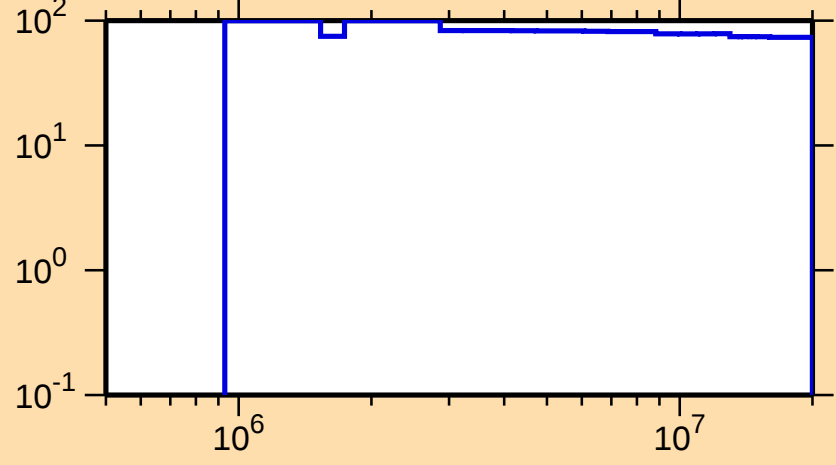
\Delta\sigma/\sigma vs. E for ^{252}\text{No}(n,n\text{cont.})
