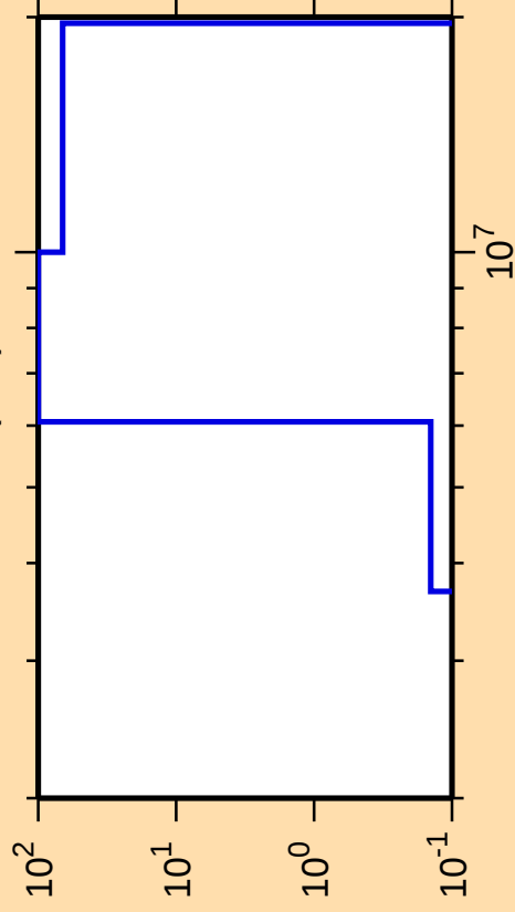
\Delta\sigma/\sigma vs. E for ^{252}\text{No}(n,d)
