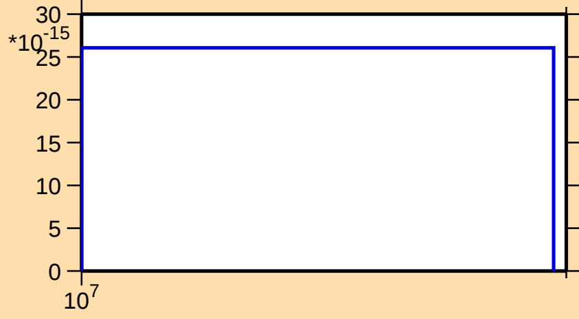
\sigma vs. E for ^{252}\text{No}(n,\text{pd})
