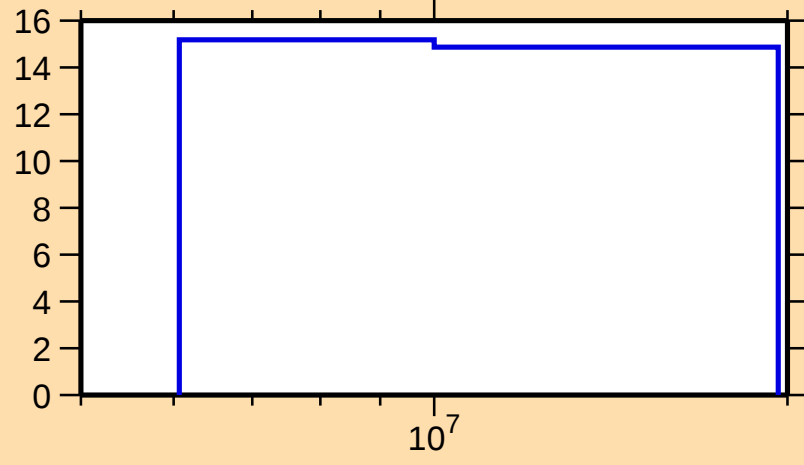
\Delta\sigma/\sigma vs. E for ^{252}\text{No}(n,\text{nonel.})
