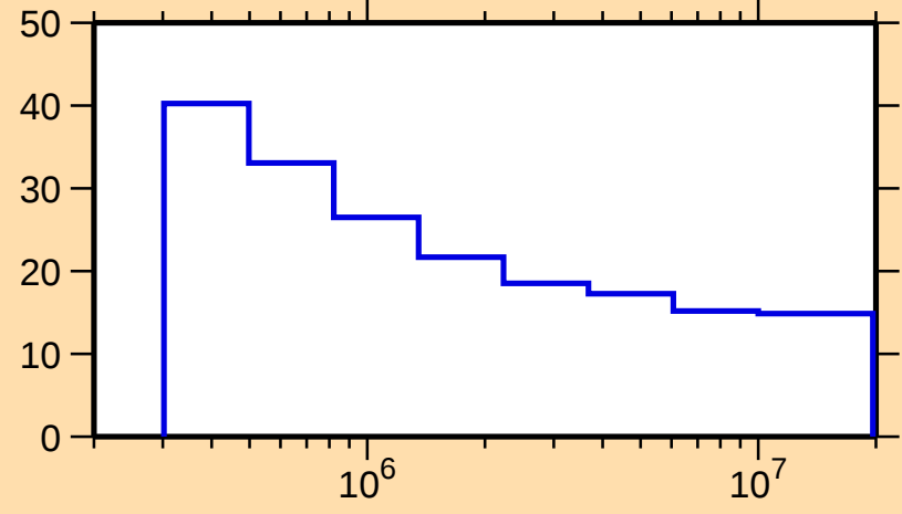
\Delta\sigma/\sigma vs. E for ^{252}\text{No}(n,n\text{onel.})
