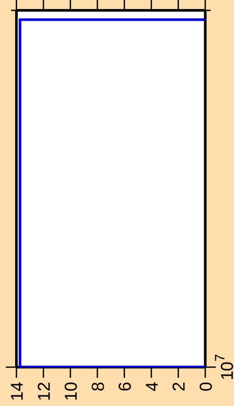
\Delta\sigma/\sigma vs. E for ^{252}\text{No}(\text{mt117})
