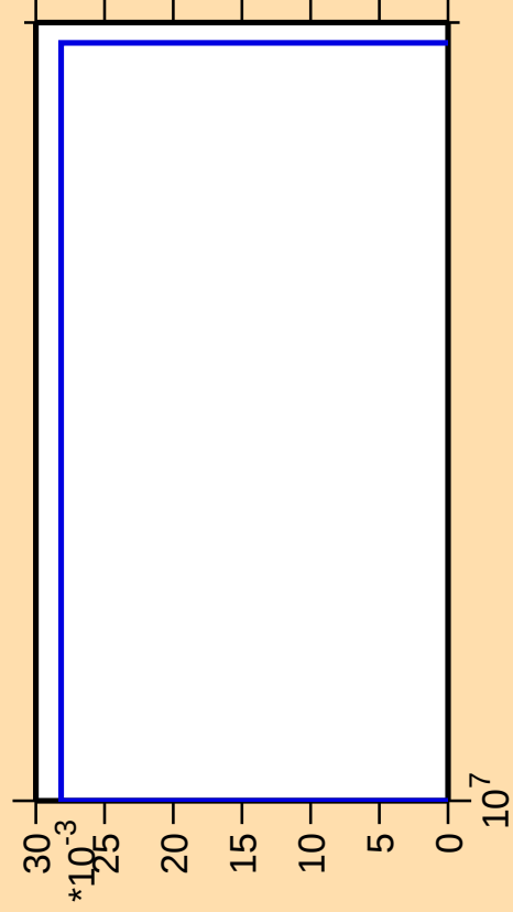
\Delta\sigma/\sigma vs. E for ^{252}\text{No}(n,\text{pt})
