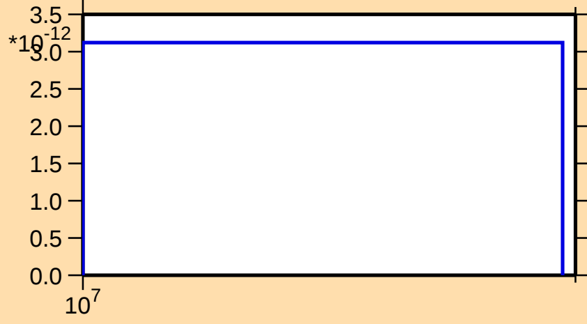
\sigma vs. E for ^{252}\text{No}(\text{mt } 45)
