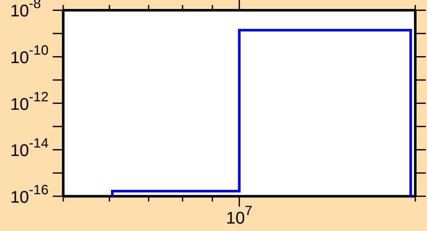
\sigma vs. E for ^{252}\text{No}(n,\text{He}3)
