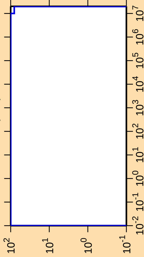
\Delta\sigma/\sigma vs. E for ^{252}\text{No}(n,\alpha)
