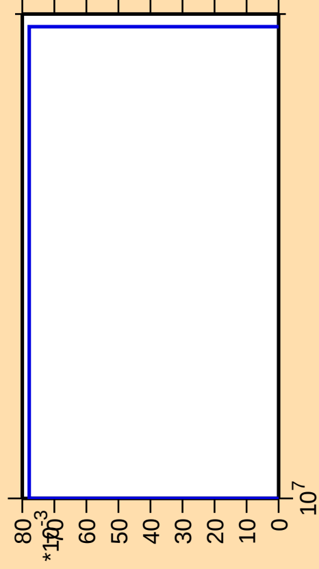
\Delta\sigma/\sigma vs. E for ^{252}\text{No}(n,\text{pd})
