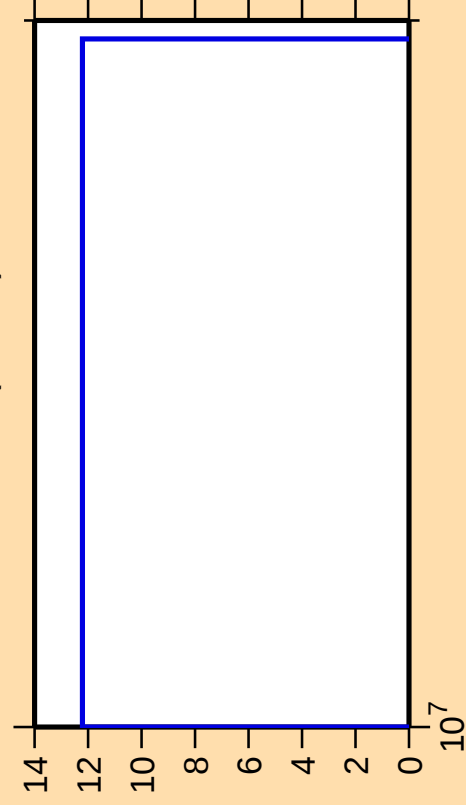
\Delta\sigma/\sigma vs. E for ^{252}\text{No}(\text{mt } 45)
