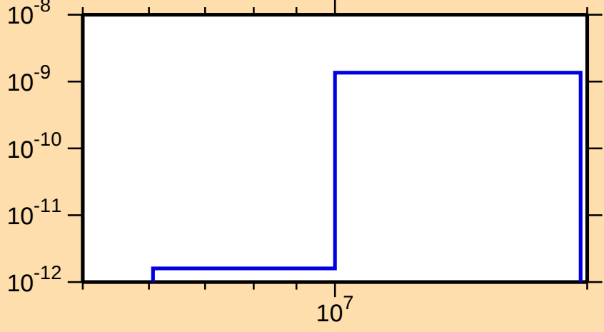
\sigma vs. E for ^{252}\text{No}(n,p\alpha)
