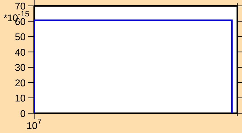
\sigma vs. E for ^{252}\text{No}(\text{mt } 34)
