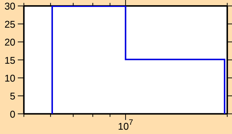
\Delta\sigma/\sigma vs. E for ^{252}\text{No}(n,\text{el.})
