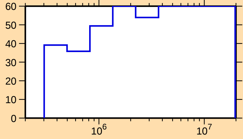
\Delta\sigma/\sigma vs. E for ^{252}\text{No}(n,n_1)
