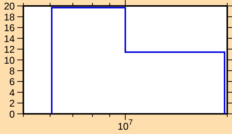
\Delta\sigma/\sigma vs. E for ^{252}\text{No}(n,\text{tot.})
