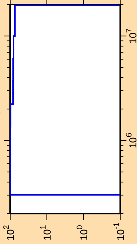
\Delta\sigma/\sigma vs. E for ^{252}\text{No}(n,n\text{cont.})
