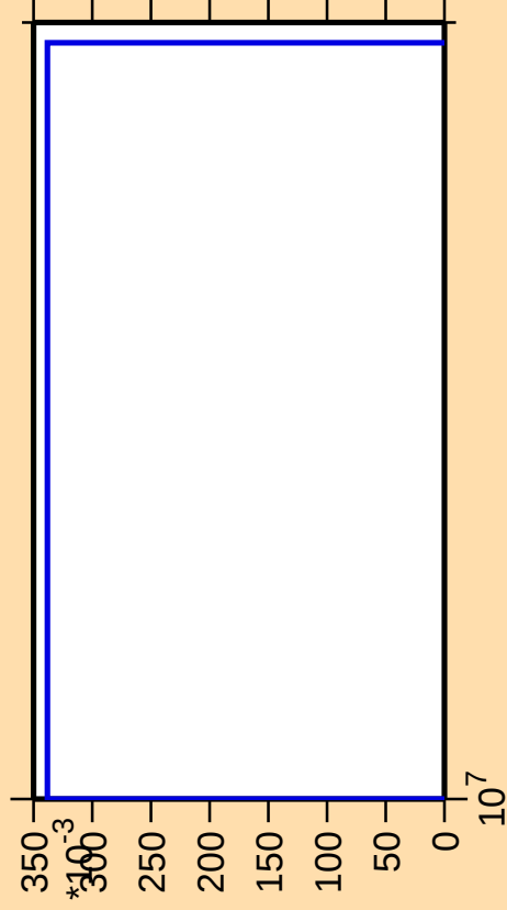
\Delta\sigma/\sigma vs. E for ^{252}\text{No}(\text{mt } 34)
