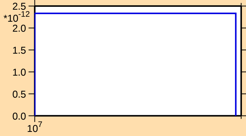
\sigma vs. E for ^{252}\text{No}(\text{mt117})
