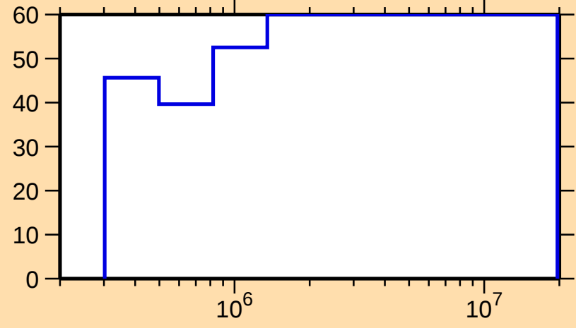
\Delta\sigma/\sigma vs. E for ^{252}\text{No}(n,\text{inel.})
