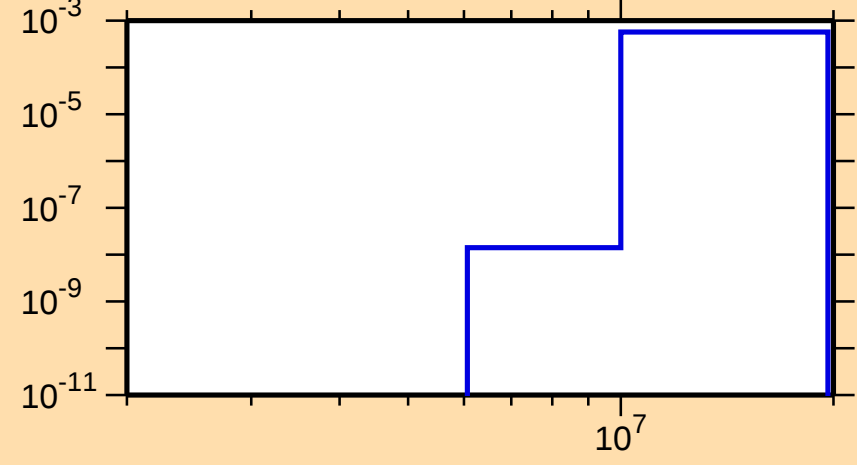
\sigma vs. E for ^{252}\text{No}(n,d)
