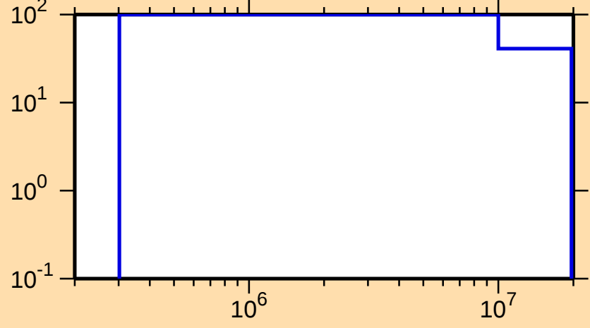
\Delta\sigma/\sigma vs. E for ^{252}\text{No}(n,f)
