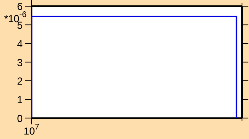
\sigma vs. E for ^{252}\text{No}(n,3n\alpha)
