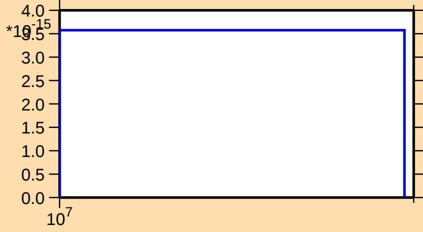
\sigma vs. E for ^{252}\text{No}(n,\text{pt})
