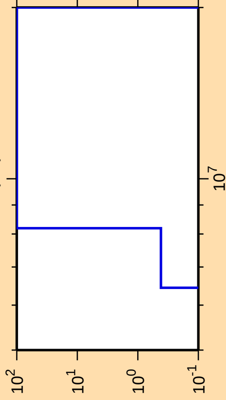
\Delta\sigma/\sigma vs. E for ^{252}\text{No}(n,t)
