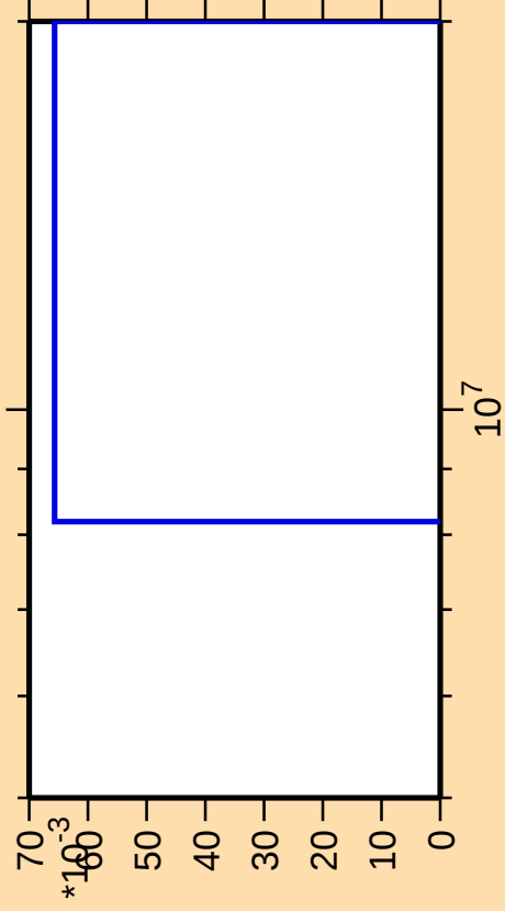
\Delta\sigma/\sigma vs. E for ^{252}\text{No}(n,\text{pd})
