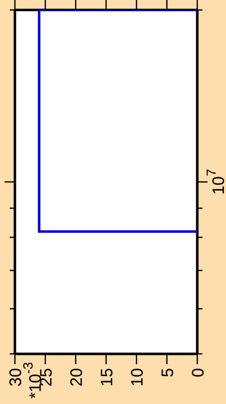
\Delta\sigma/\sigma vs. E for ^{252}\text{No}(n,\text{pt})
