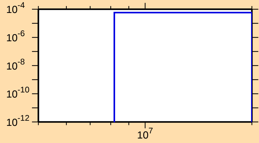
\sigma vs. E for ^{252}\text{No}(n,t)
