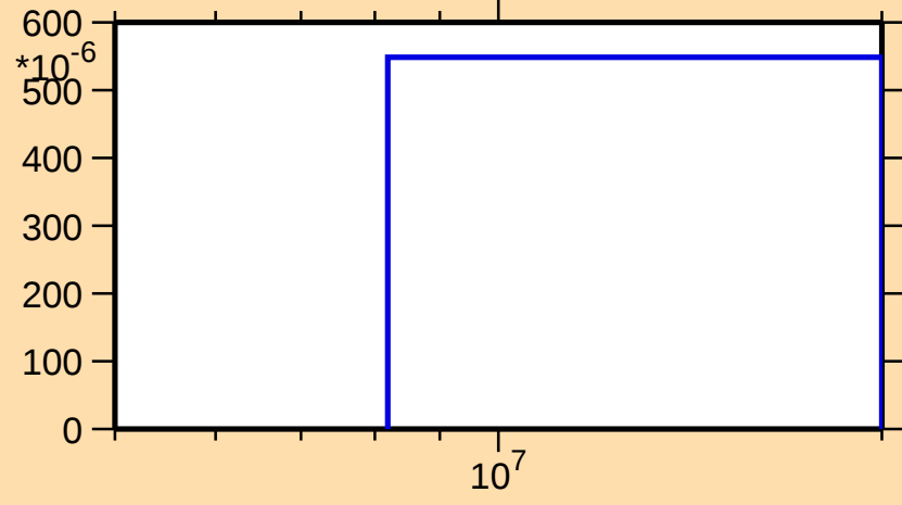
\sigma vs. E for ^{252}\text{No}(n,3n)
