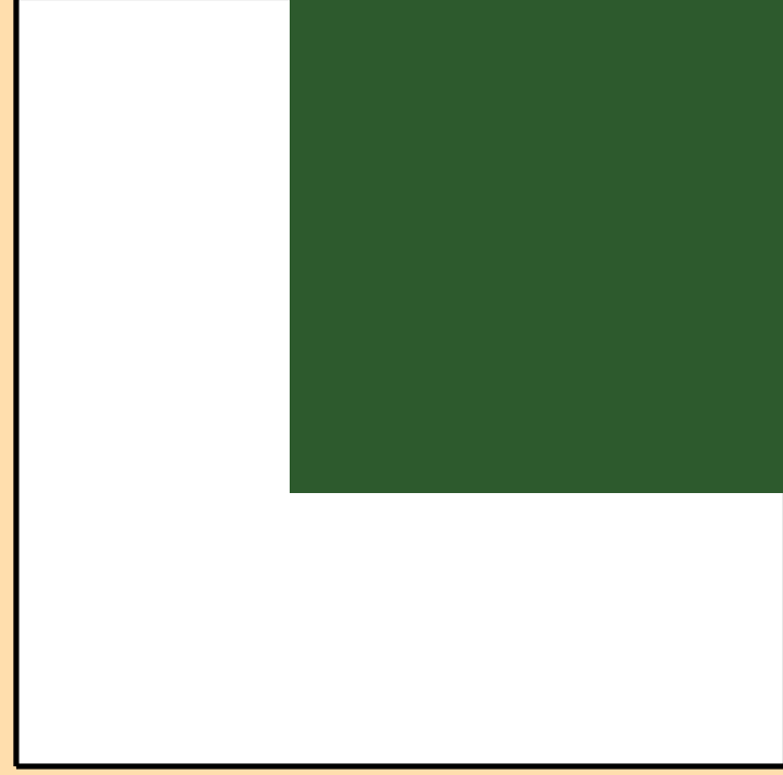
\sigma vs. E for ^{252}\text{No}(\text{mt } 45)
