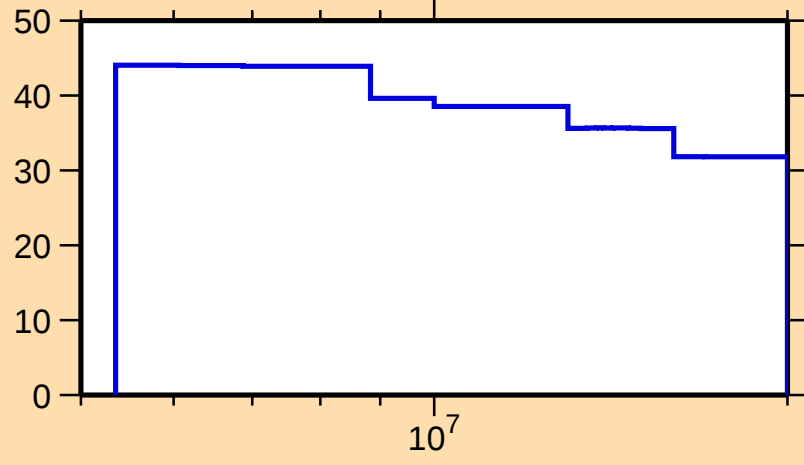
\Delta\sigma/\sigma vs. E for ^{255}\text{No}(n,\text{nonel.})
