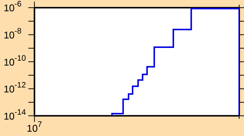
\sigma vs. E for ^{255}\text{No}(n,nt)
