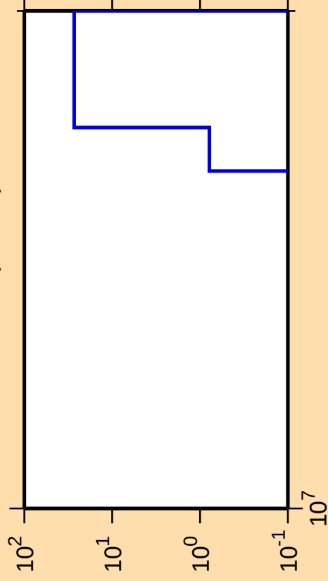
\Delta\sigma/\sigma vs. E for ^{255}\text{No}(\text{mt } 34)
