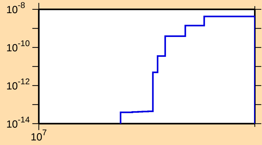
\sigma vs. E for ^{255}\text{No}(n,3n\alpha)
