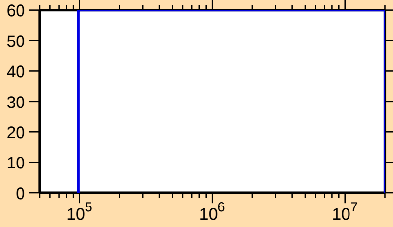
\Delta\sigma/\sigma vs. E for ^{255}\text{No}(n,\text{ncont.})
