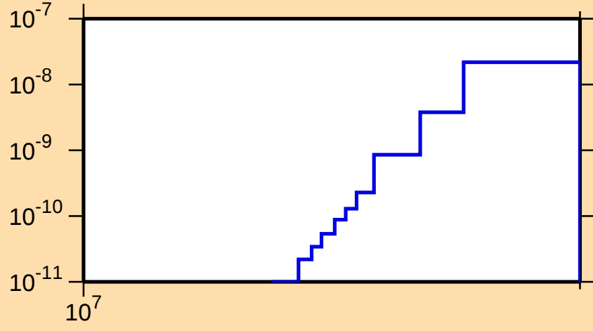
\sigma vs. E for ^{255}\text{No}(n,\text{He}3)
