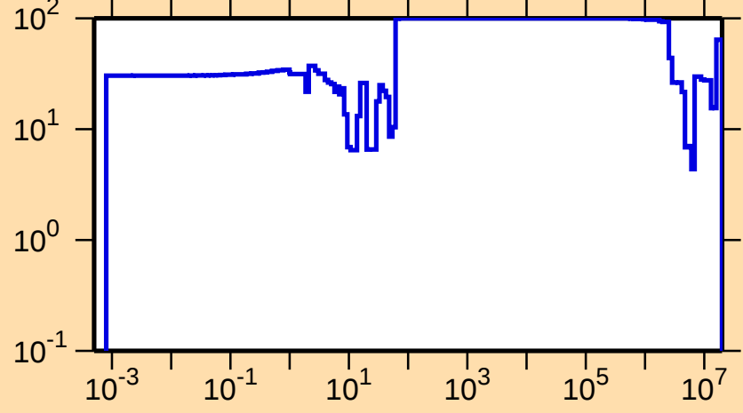
\Delta\sigma/\sigma vs. E for ^{255}\text{No}(n,\gamma)
