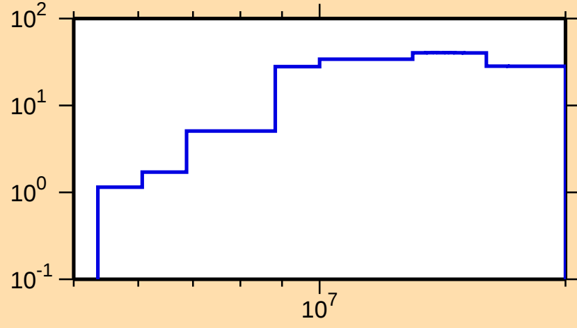
\Delta\sigma/\sigma vs. E for ^{255}\text{No}(n,\text{el.})
