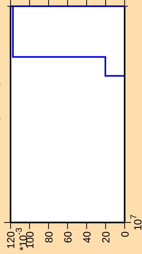
\Delta\sigma/\sigma vs. E for ^{255}\text{No}(\text{mt 45})
