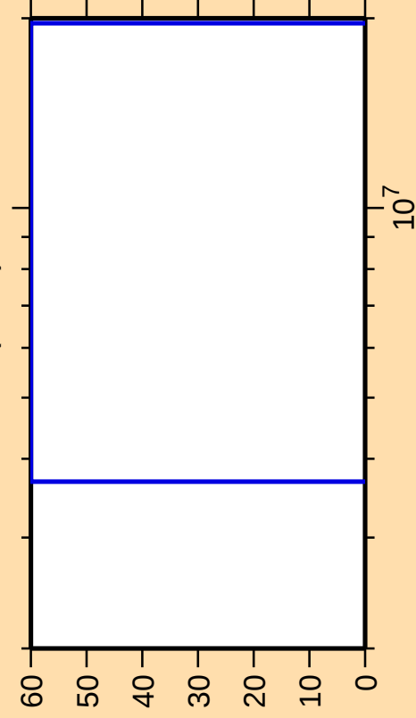
\Delta\sigma/\sigma vs. E for ^{255}\text{No}(n,2n)
