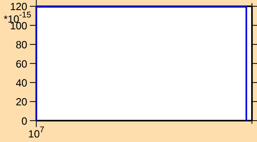
\sigma vs. E for ^{255}\text{No}(\text{mt } 45)
