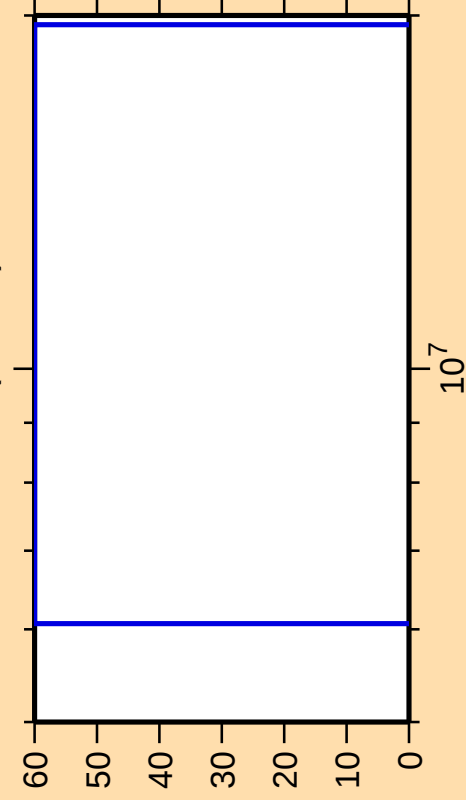
\Delta\sigma/\sigma vs. E for ^{255}\text{No}(n,2n\alpha)
