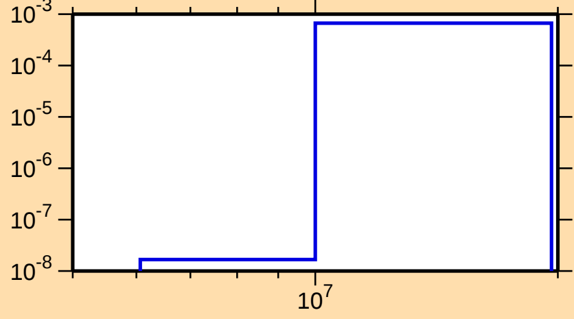
\sigma vs. E for ^{255}\text{No}(n,d)
