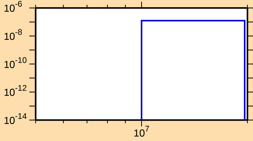
\sigma vs. E for ^{255}\text{No}(n,\text{nd})
