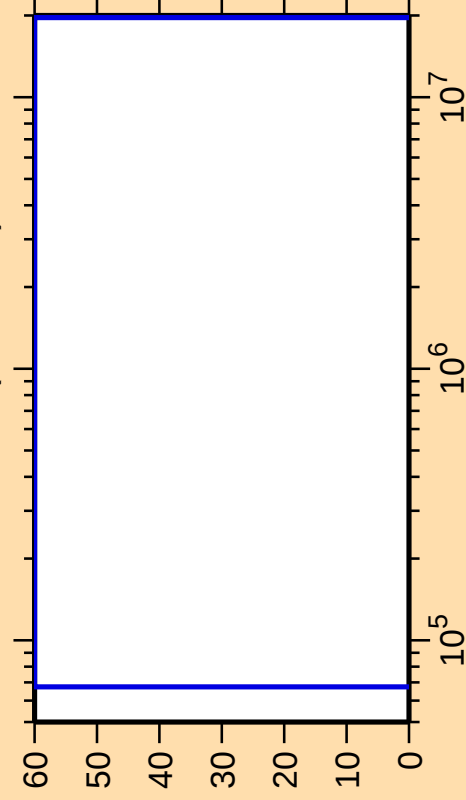
\Delta\sigma/\sigma vs. E for ^{255}\text{No}(n,n\text{cont.})
