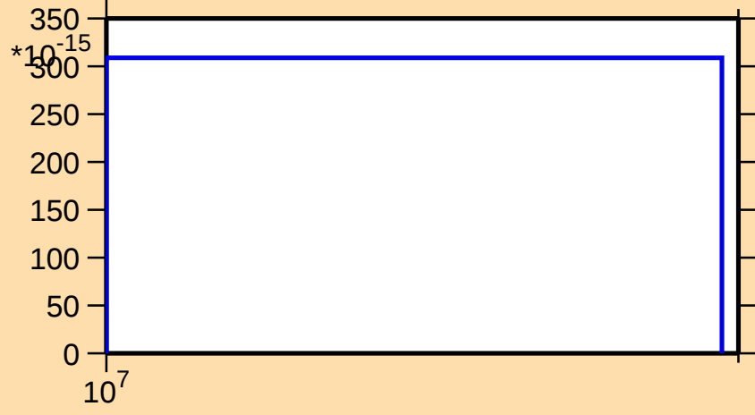
\sigma vs. E for ^{255}\text{No}(\text{mt } 34)
