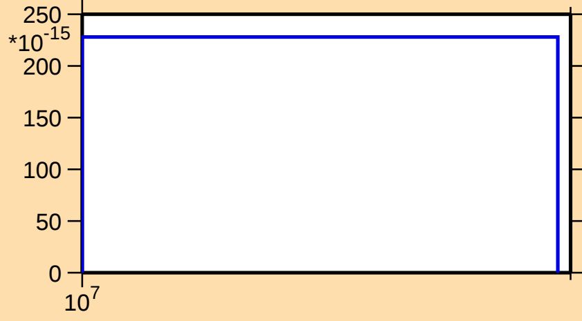
\sigma vs. E for ^{255}\text{No}(\text{mt117})
