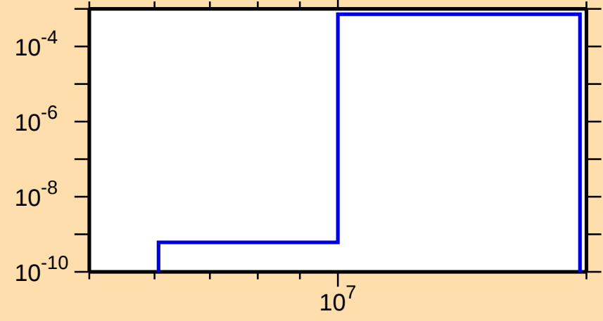
\sigma vs. E for ^{255}\text{No}(n,2n\alpha)
