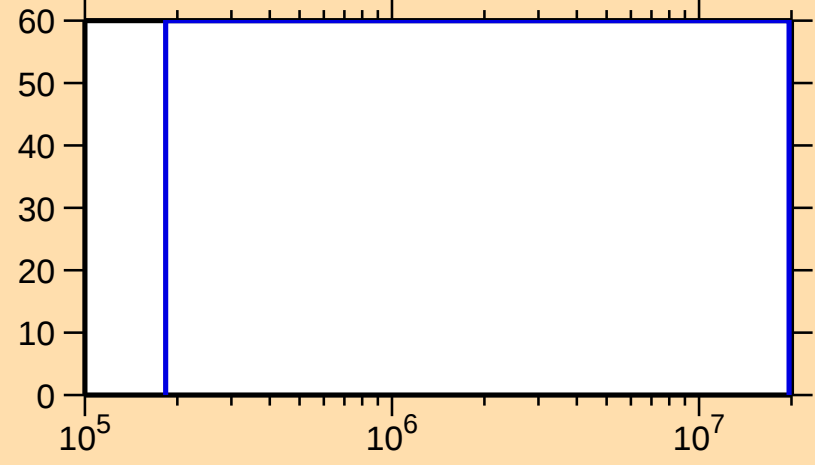
\Delta\sigma/\sigma vs. E for ^{255}\text{No}(n,n\text{cont.})
