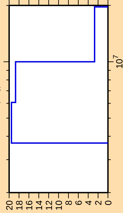
\Delta\sigma/\sigma vs. E for ^{255}\text{No}(n,\gamma)
