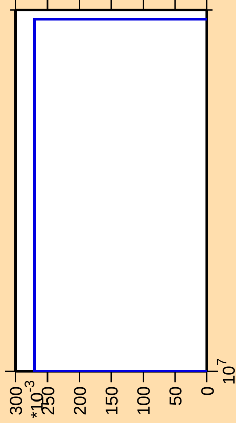
\Delta\sigma/\sigma vs. E for ^{255}\text{No}(\text{mt } 34)
