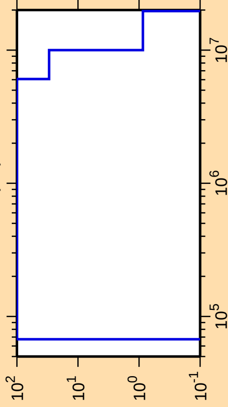
\Delta\sigma/\sigma vs. E for ^{255}\text{No}(n,f)
