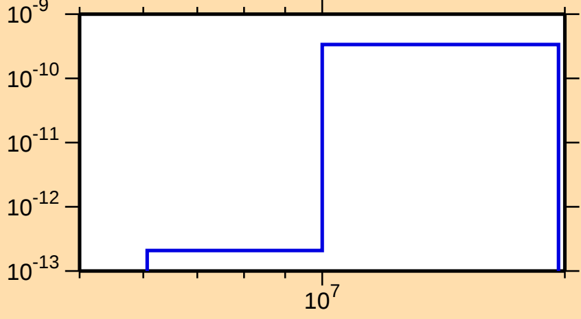
\sigma vs. E for ^{255}\text{No}(n,p\alpha)
