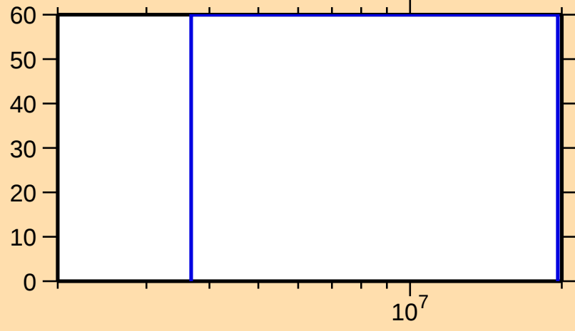
\Delta\sigma/\sigma vs. E for ^{255}\text{No}(n,2n)
