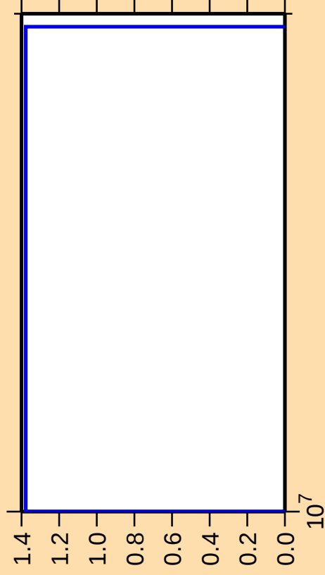
\Delta\sigma/\sigma vs. E for ^{255}\text{No}(\text{mt117})
