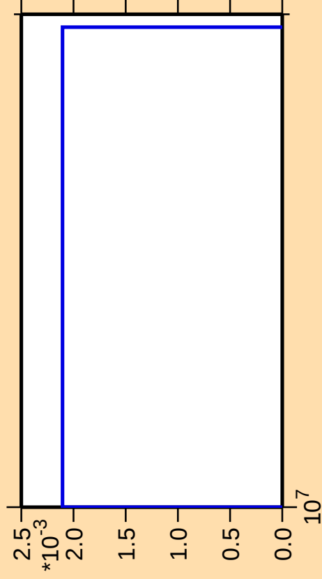
\Delta\sigma/\sigma vs. E for ^{255}\text{No}(\text{mt } 45)
