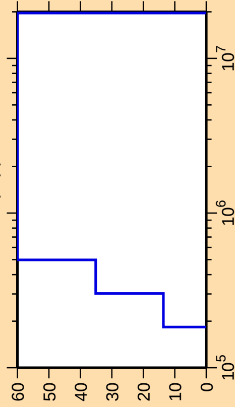
\Delta\sigma/\sigma vs. E for ^{255}\text{No}(n,p)
