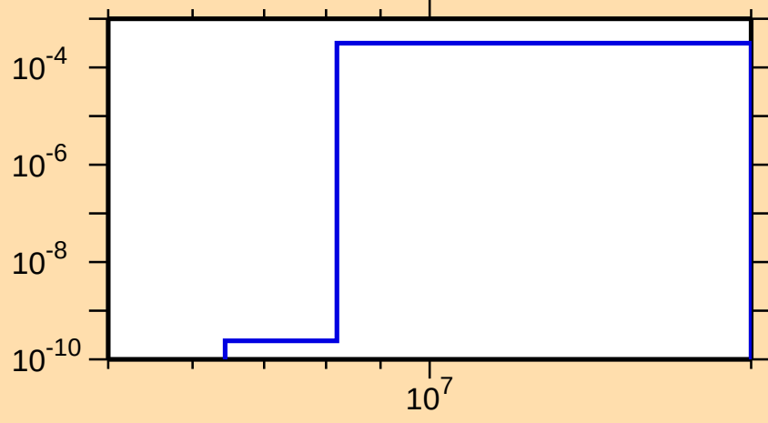
\sigma vs. E for ^{255}\text{No}(n,np)
