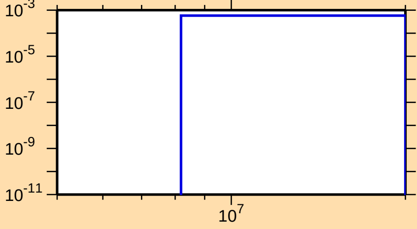
\sigma vs. E for ^{255}\text{No}(n,2n\alpha)
