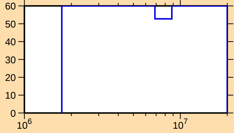
\Delta\sigma/\sigma vs. E for ^{256}\text{No}(n,\gamma)
