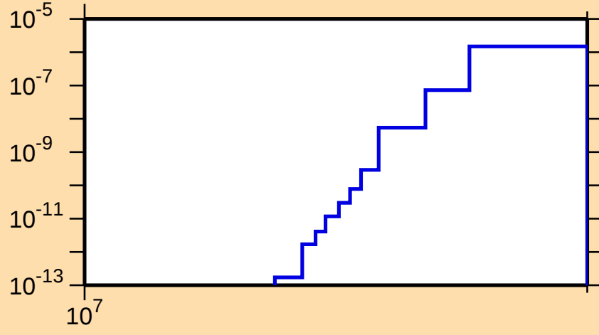
\sigma vs. E for ^{256}\text{No}(n,\text{nd})
