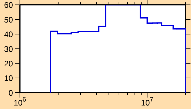
\Delta\sigma/\sigma vs. E for ^{256}\text{No}(n,n\text{cont.})
