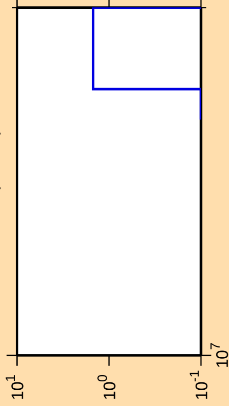
\Delta\sigma/\sigma vs. E for ^{256}\text{No}(\text{mt } 34)
