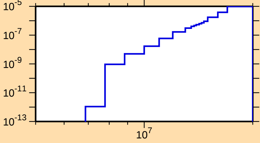
\sigma vs. E for ^{256}\text{No}(n,2n\alpha)
