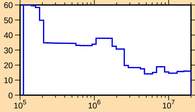
\Delta\sigma/\sigma vs. E for ^{228}\text{Pa}(n,n\text{onel.})
