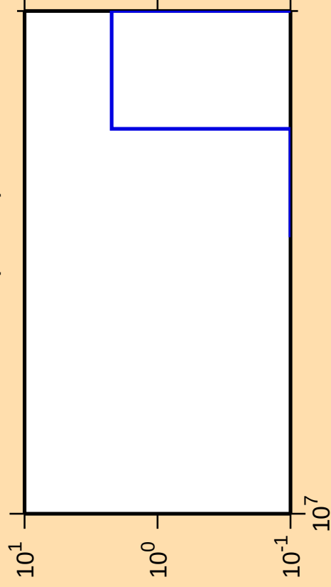
\Delta\sigma/\sigma vs. E for ^{228}\text{Pa}(\text{mt } 11)
