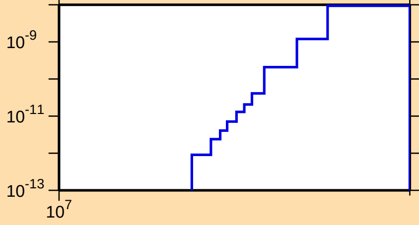
\sigma vs. E for ^{228}\text{Pa}(n,\text{He3})
