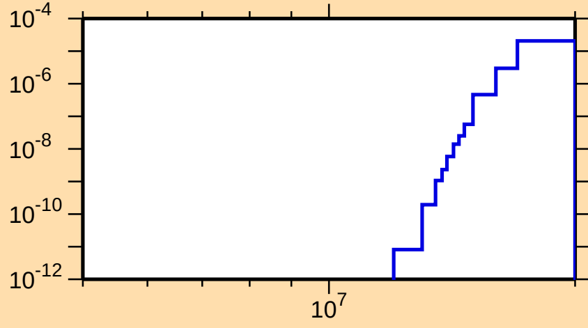
\sigma vs. E for ^{228}\text{Pa}(n,2np)
