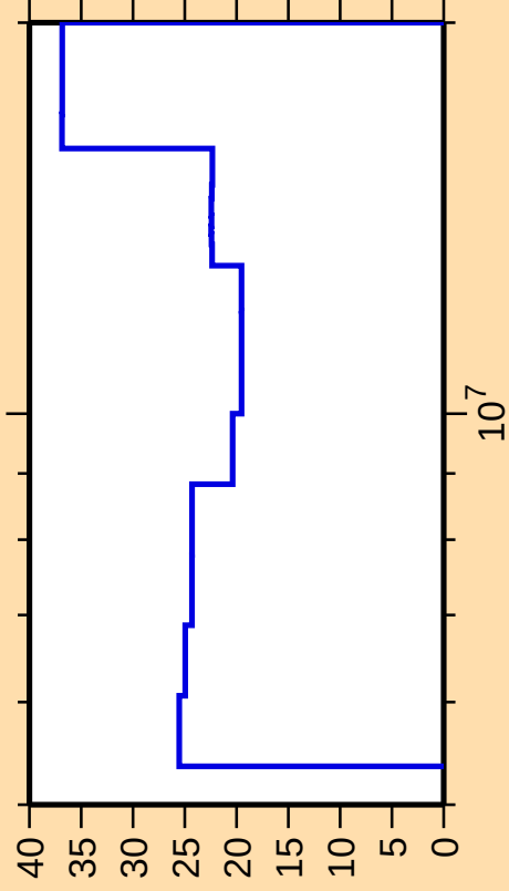
\Delta\sigma/\sigma vs. E for ^{228}\text{Pa}(n,f)
