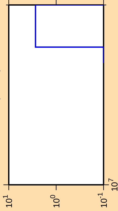
\Delta\sigma/\sigma vs. E for ^{228}\text{Pa} (mt 34)
