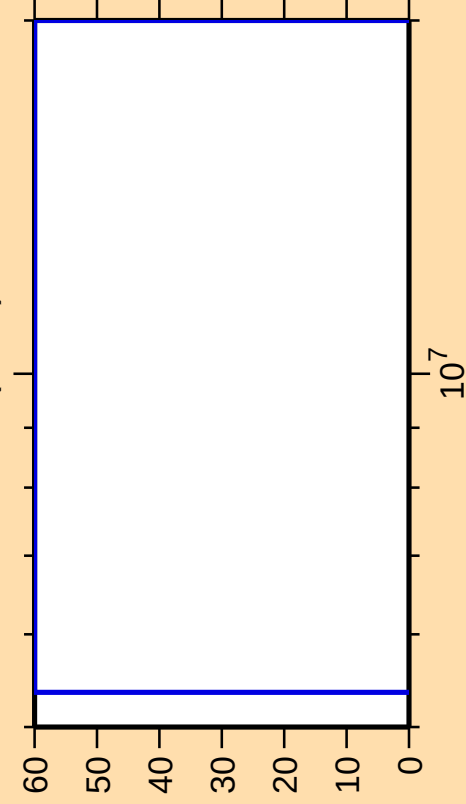
\Delta\sigma/\sigma vs. E for ^{228}\text{Pa}(n,2n)
