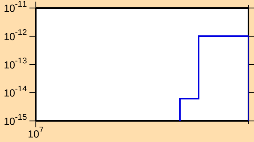
\sigma vs. E for ^{228}\text{Pa} (mt 34)
