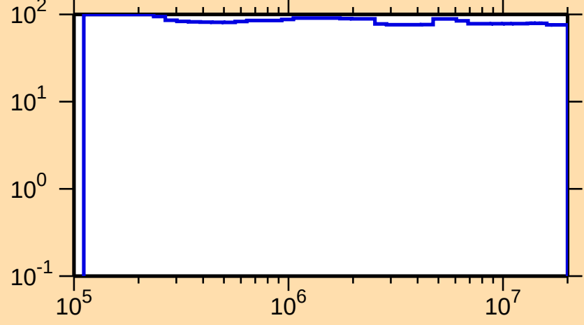
\Delta\sigma/\sigma vs. E for ^{228}\text{Pa}(n,\text{inel.})
