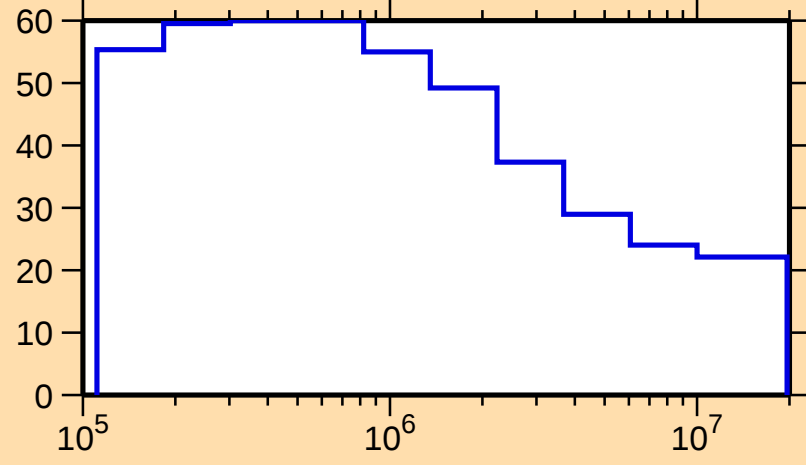
\Delta\sigma/\sigma vs. E for ^{228}\text{Pa}(n,f)
