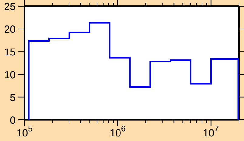
\Delta\sigma/\sigma vs. E for ^{228}\text{Pa}(n,\text{tot.})
