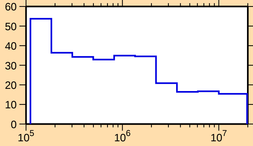
\Delta\sigma/\sigma vs. E for ^{228}\text{Pa}(\text{n},\text{nonel.})
