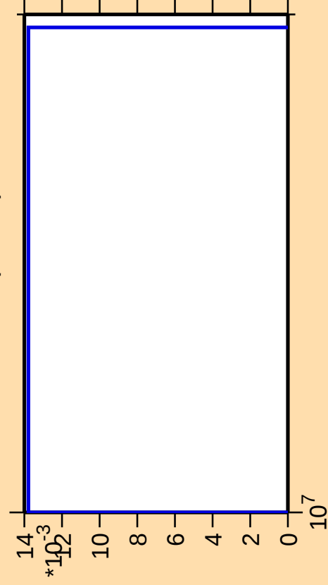
\Delta\sigma/\sigma vs. E for ^{228}\text{Pa} (mt 11)
