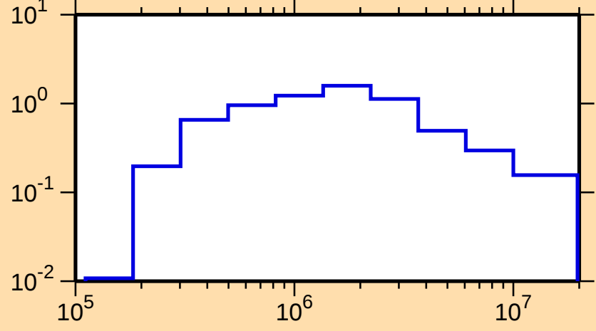
\sigma vs. E for ^{228}\text{Pa}(n,\text{inel.})
