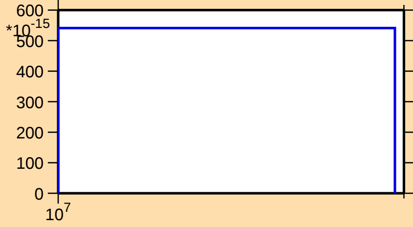
\sigma vs. E for ^{228}\text{Pa}(\text{mt117})
