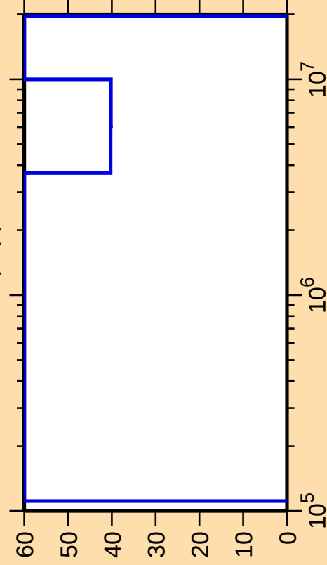
\Delta\sigma/\sigma vs. E for ^{228}\text{Pa}(n,p)
