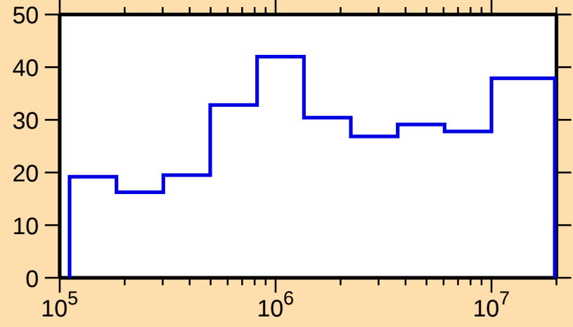
\Delta\sigma/\sigma vs. E for ^{228}\text{Pa}(\text{n,el.})
