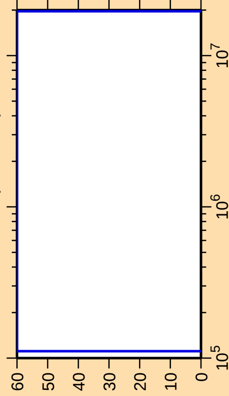
\Delta\sigma/\sigma vs. E for ^{228}\text{Pa}(n,\text{ncont.})
