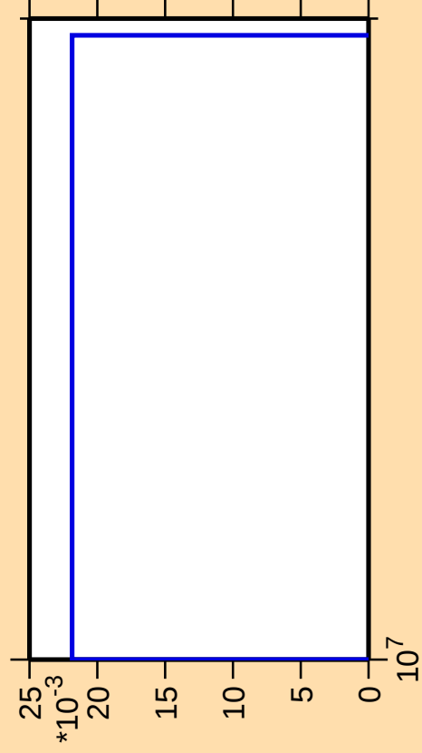
\Delta\sigma/\sigma vs. E for ^{228}\text{Pa}(\text{mt } 34)
