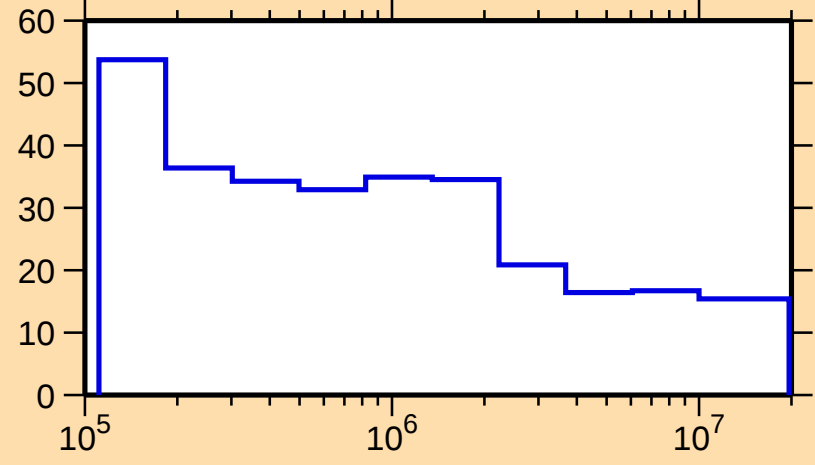
\Delta\sigma/\sigma vs. E for ^{228}\text{Pa}(\text{n,nonel.})
