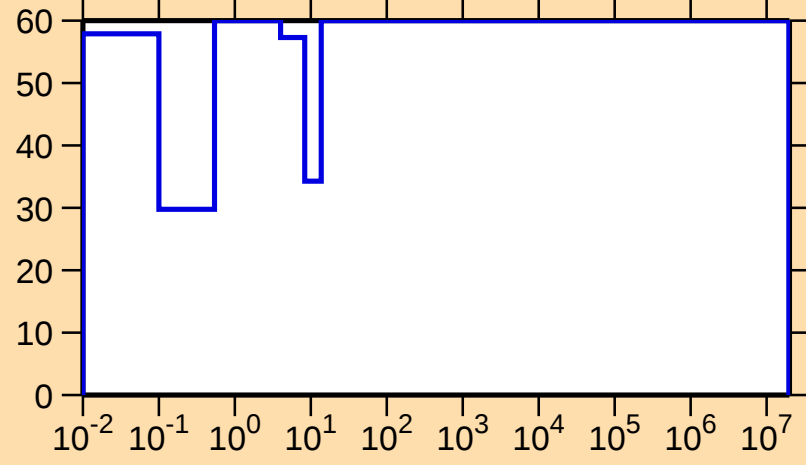
\Delta\sigma/\sigma vs. E for ^{228}\text{Pa}(n,\gamma)
