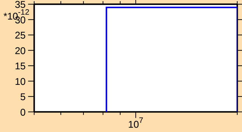
\sigma vs. E for ^{228}\text{Pa}(n,p\alpha)
