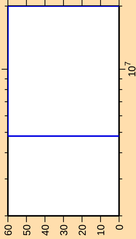
\Delta\sigma/\sigma vs. E for ^{228}\text{Pa}(n,n\text{cont.})
