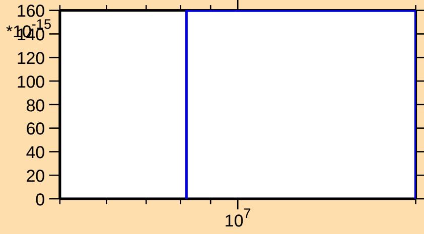
\sigma vs. E for ^{228}\text{Pa}(\text{mt } 45)
