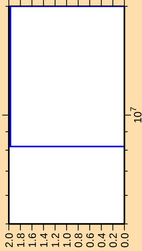
\Delta\sigma/\sigma vs. E for ^{228}\text{Pa}(\text{mt117})
