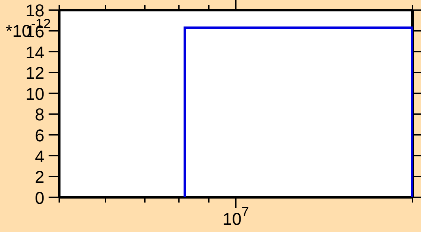
\sigma vs. E for ^{228}\text{Pa}(n,3n\alpha)
