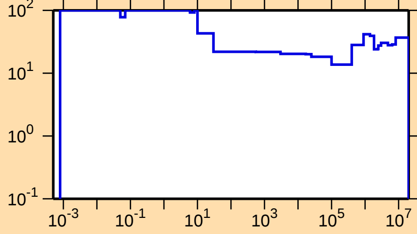
\Delta\sigma/\sigma vs. E for ^{228}\text{Pa}(n,\text{el.})
