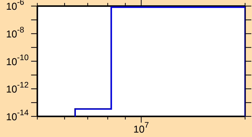
\sigma vs. E for ^{228}\text{Pa}(n,2n\alpha)
