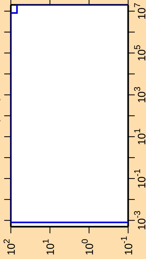
\Delta\sigma/\sigma vs. E for ^{228}\text{Pa}(n,\alpha)
