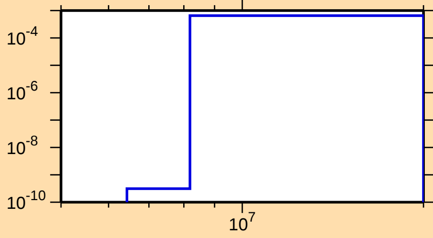
\sigma vs. E for ^{228}\text{Pa}(n,d)
