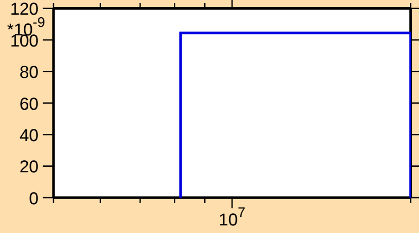
\sigma vs. E for ^{228}\text{Pa}(n,nt)
