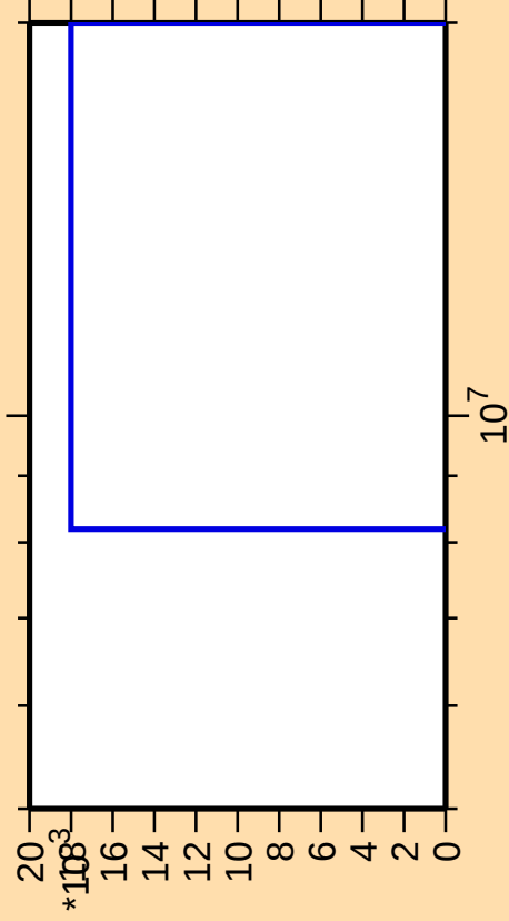
\Delta\sigma/\sigma vs. E for ^{228}\text{Pa}(\text{mt 11})
