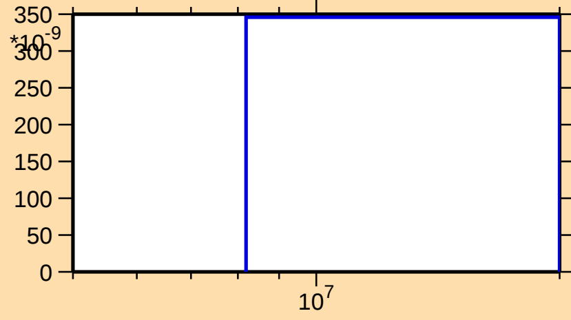
\sigma vs. E for ^{228}\text{Pa}(n,2np)
