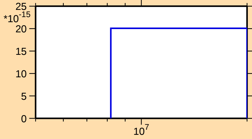
\sigma vs. E for ^{228}\text{Pa}(\text{mt 11})
