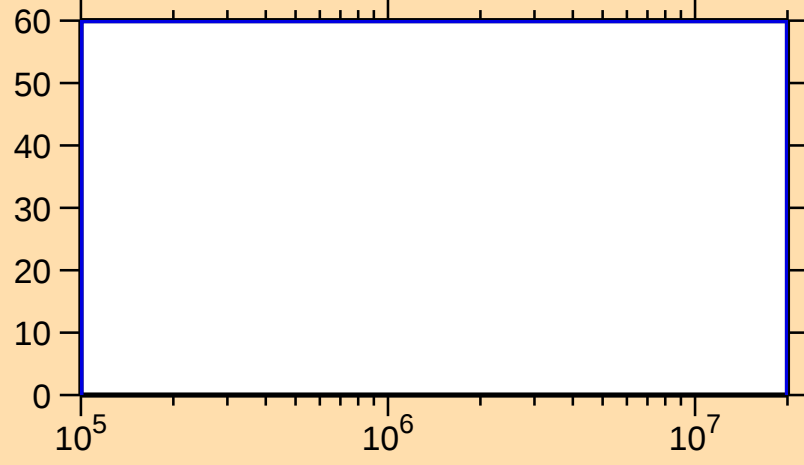
\Delta\sigma/\sigma vs. E for ^{228}\text{Pa}(\text{n},\text{inel.})
