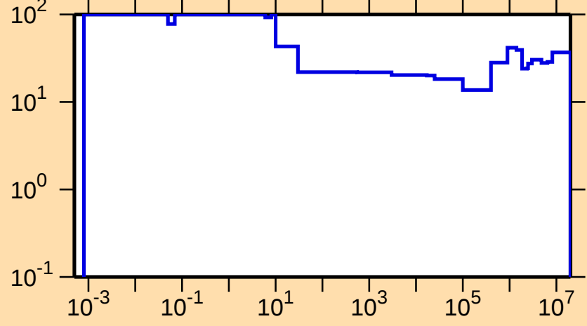
\Delta\sigma/\sigma vs. E for ^{228}\text{Pa}(n,\text{el.})
