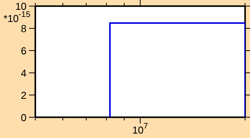
\sigma vs. E for ^{228}\text{Pa}(\text{mt } 34)
