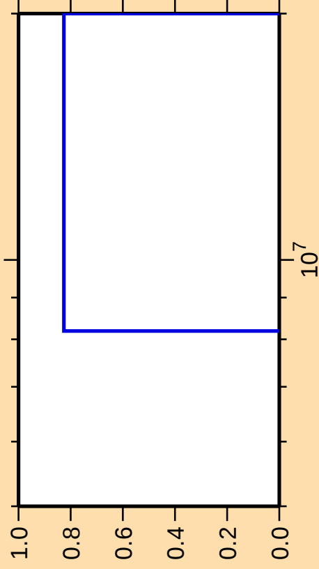
\Delta\sigma/\sigma vs. E for ^{228}\text{Pa}(\text{mt } 45)
