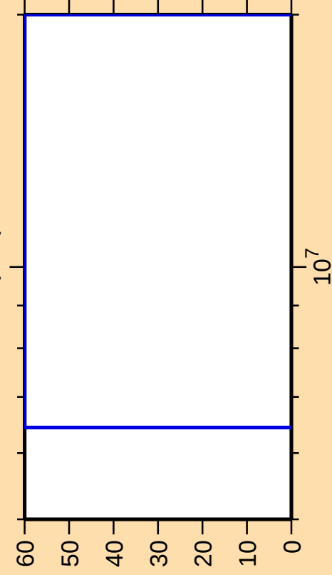
\Delta\sigma/\sigma vs. E for ^{228}\text{Pa}(n,d)
