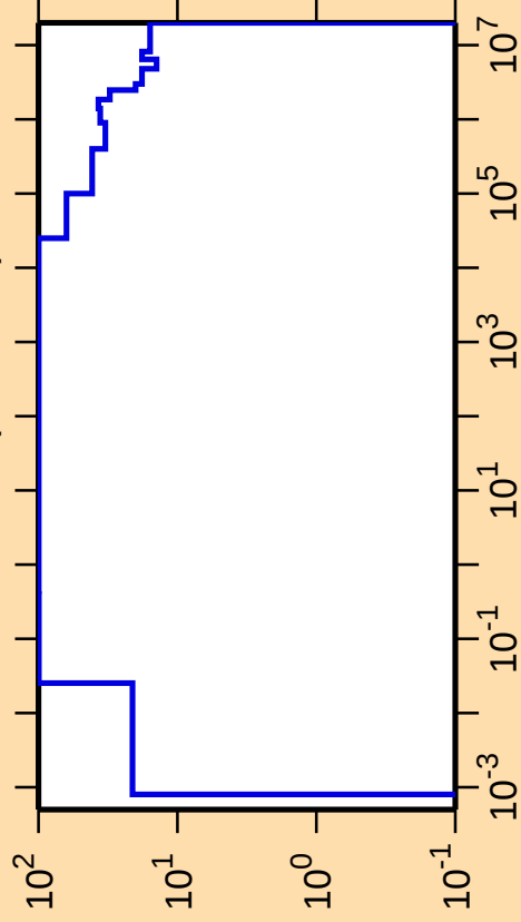
\Delta\sigma/\sigma vs. E for ^{228}\text{Pa}(n,\text{nonel.})
