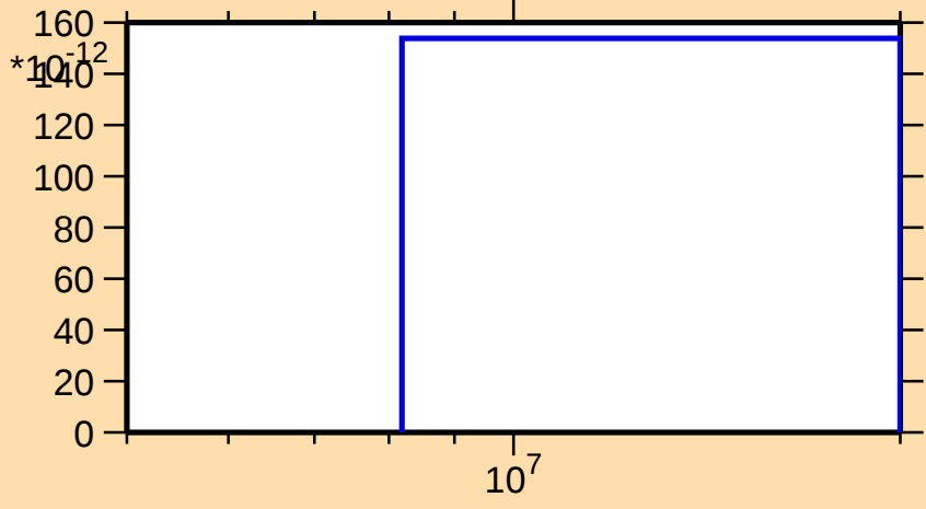
\sigma vs. E for ^{228}\text{Pa}(n,\text{He3})
