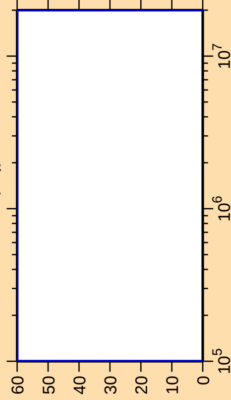
\Delta\sigma/\sigma vs. E for ^{228}\text{Pa}(n,\gamma)
