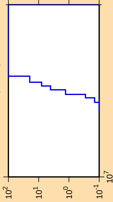
\Delta\sigma/\sigma vs. E for ^{136}\text{Pm}(\text{mt } 34)
