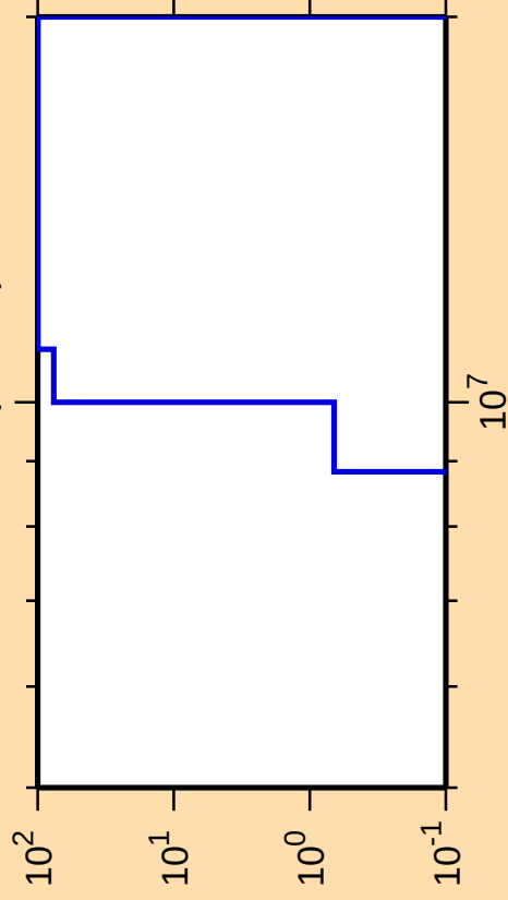
\Delta\sigma/\sigma vs. E for ^{136}\text{Pm}(\text{mt } 45)
