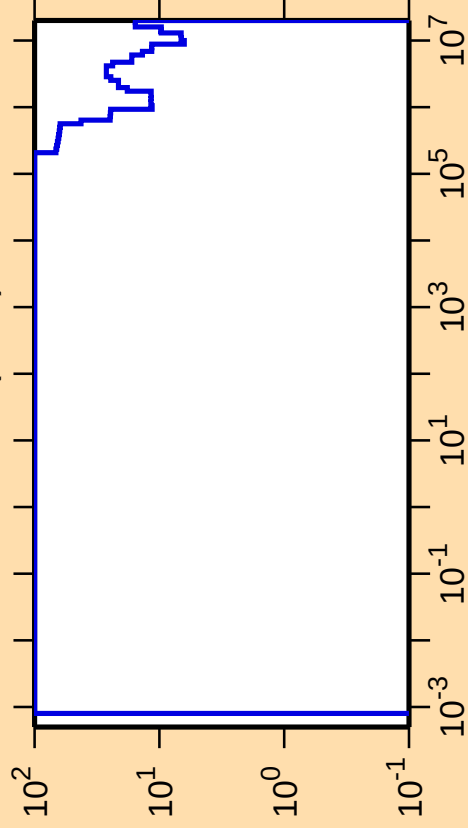
\Delta\sigma/\sigma vs. E for ^{136}\text{Pm}(n,\text{el.})
