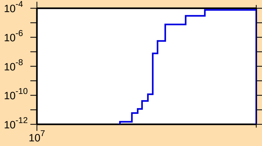
\sigma vs. E for ^{136}\text{Pm}(n,2n\alpha)
