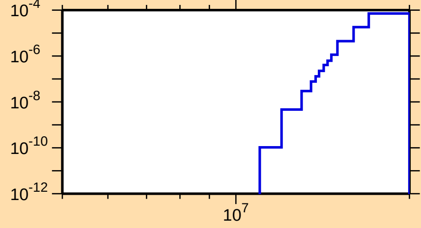
\sigma vs. E for ^{136}\text{Pm}(n,\text{pd})
