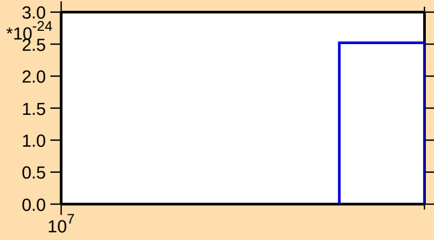
\sigma vs. E for ^{136}\text{Pm}(\text{mt 11})
