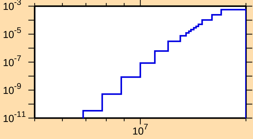
\sigma vs. E for ^{136}\text{Pm}(n,\text{He3})
