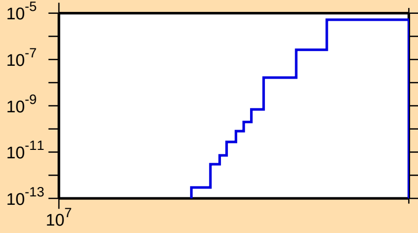
\sigma vs. E for ^{136}\text{Pm}(n,\text{pt})
