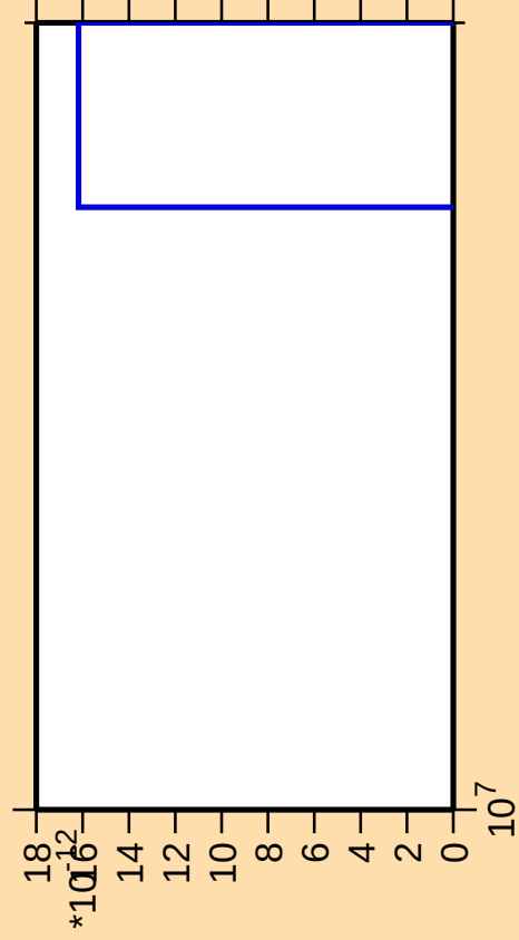
\Delta\sigma/\sigma vs. E for ^{136}\text{Pm}(\text{mt 11})
