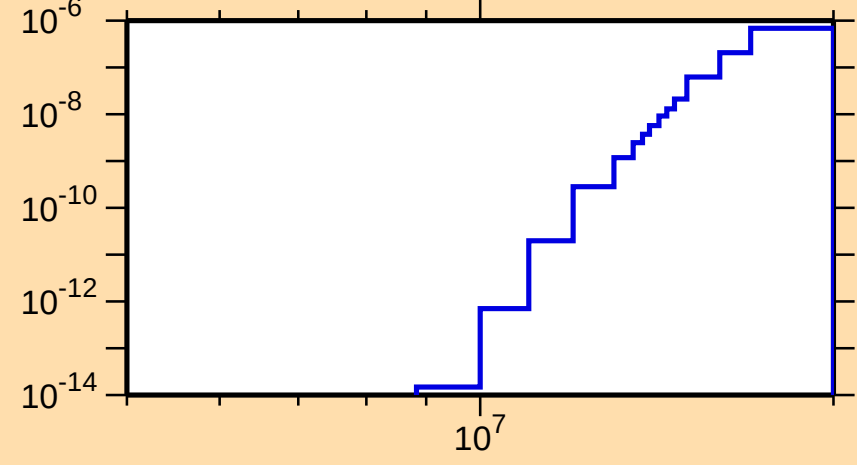
\sigma vs. E for ^{136}\text{Pm}(\text{mt117})
