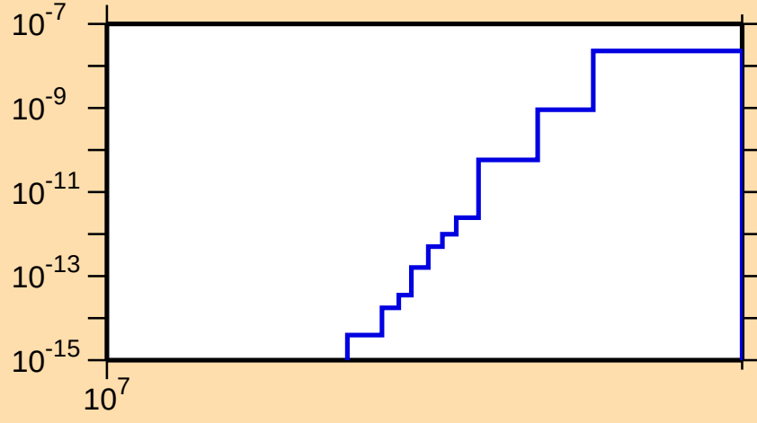
\sigma vs. E for ^{136}\text{Pm}(\text{mt } 34)
