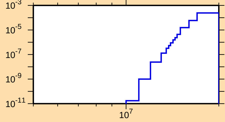
\sigma vs. E for ^{136}\text{Pm}(\text{mt } 45)
