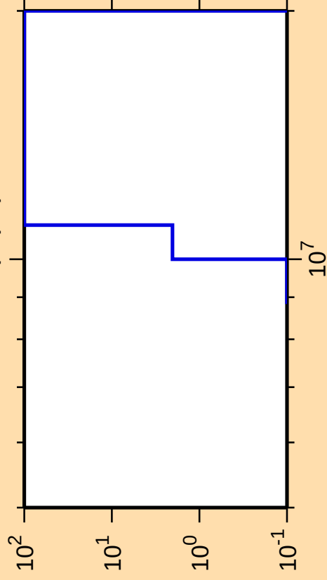
\Delta\sigma/\sigma vs. E for ^{136}\text{Pm}(n,\text{pd})
