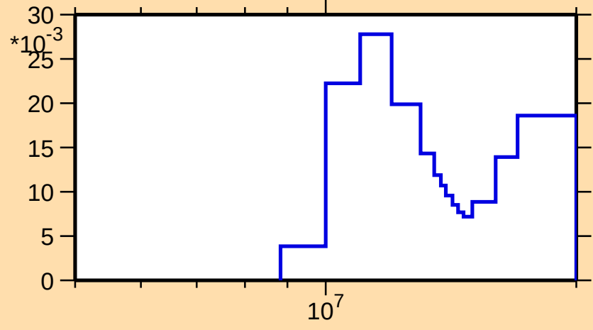
\sigma vs. E for ^{136}\text{Pm}(n,2n)
