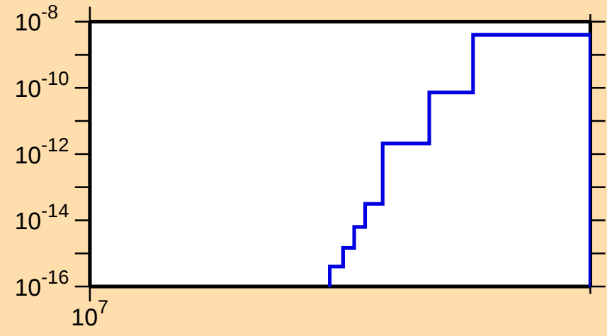
\sigma vs. E for ^{236}\text{Pu}(n,\text{nt})
