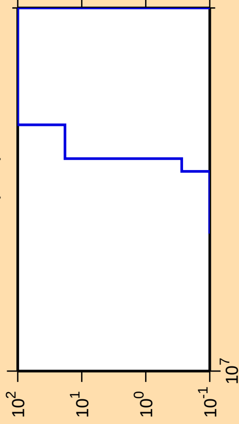
\Delta\sigma/\sigma vs. E for ^{236}\text{Pu}(n,\text{nt})
