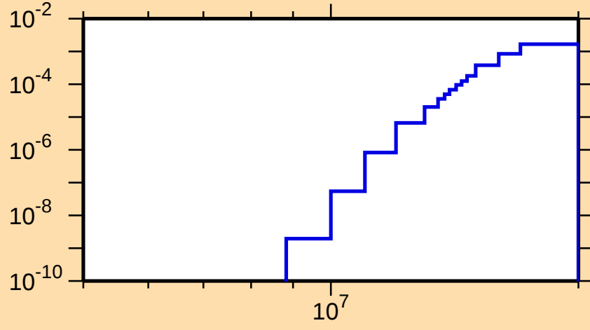
\sigma vs. E for ^{236}\text{Pu}(n,d)
