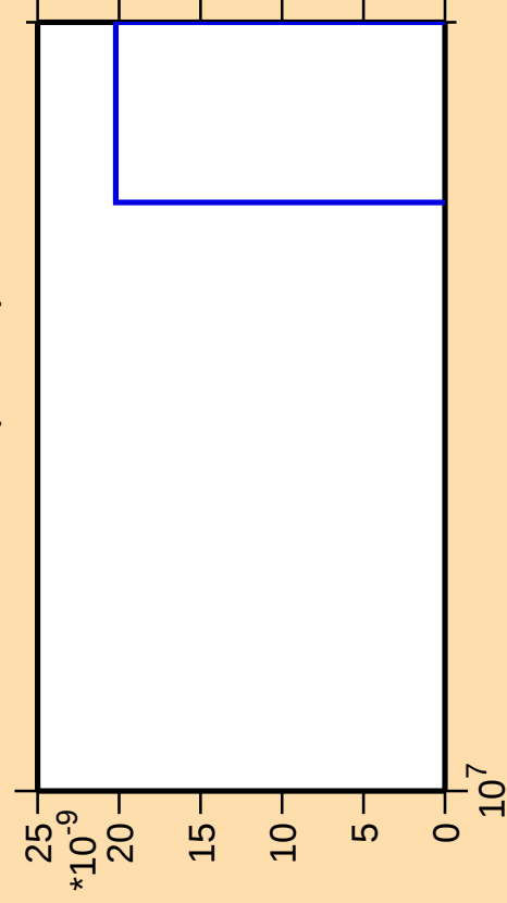
\Delta\sigma/\sigma vs. E for ^{236}\text{Pu} (mt 42)
