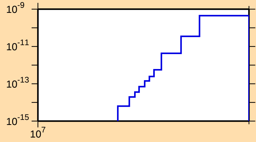
\sigma vs. E for ^{236}\text{Pu}(n,\text{He3})
