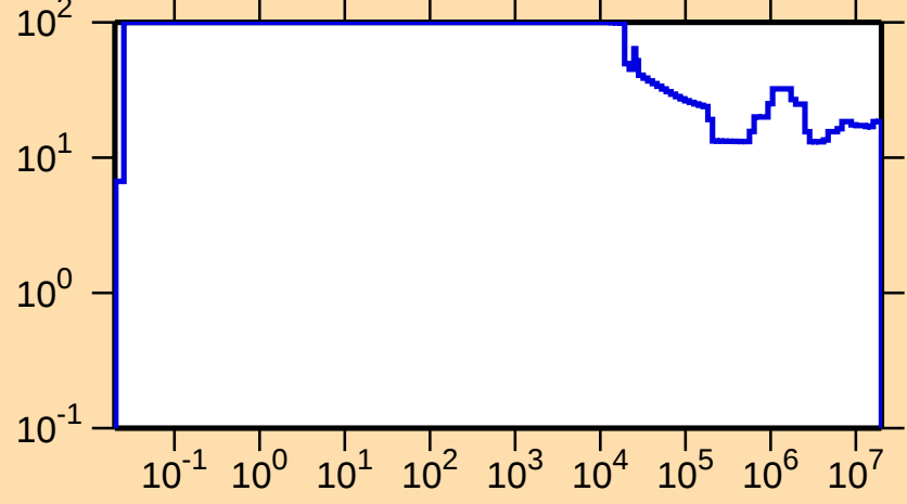
\Delta\sigma/\sigma vs. E for ^{236}\text{Pu}(n,\text{nonel.})
