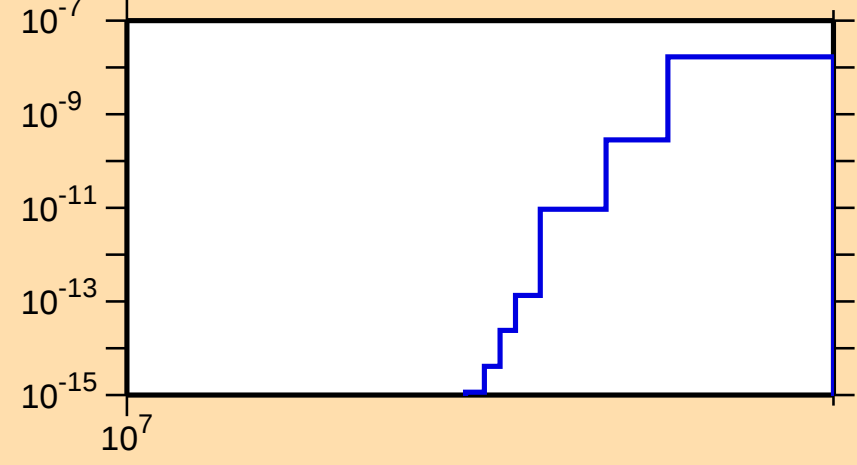
\sigma vs. E for ^{236}\text{Pu}(n,\text{nd})
