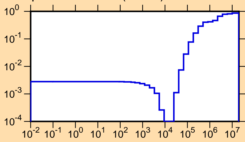
\mu vs. E for ^{236}\text{Pu}(\text{mt251})
