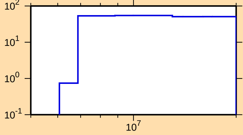
\Delta\sigma/\sigma vs. E for ^{244}\text{Pu}(n,p)
