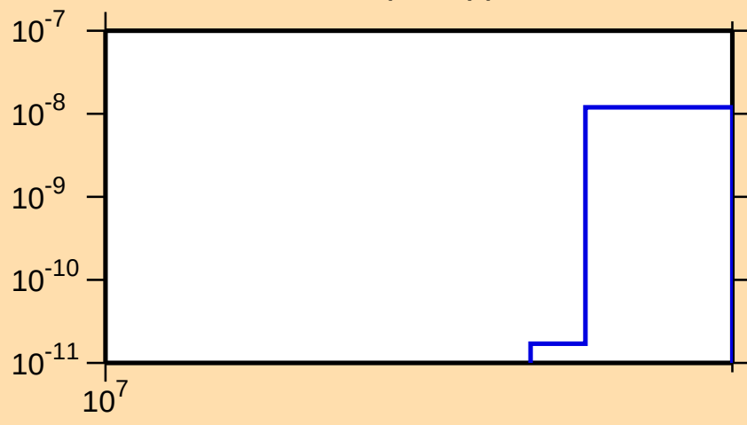
\sigma vs. E for ^{244}\text{Pu}(n,2np)
