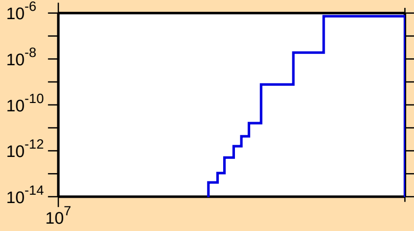
\sigma vs. E for ^{244}\text{Pu}(n,\text{nt})
