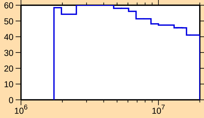
\Delta\sigma/\sigma vs. E for ^{244}\text{Pu}(n,n\text{onel.})
