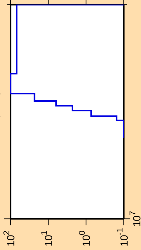
\Delta\sigma/\sigma vs. E for ^{244}\text{Pu}(n,\text{nt})
