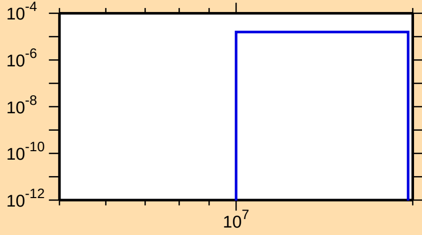
\sigma vs. E for ^{244}\text{Pu}(n,t)
