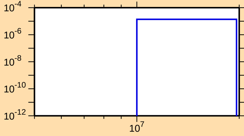
\sigma vs. E for ^{244}\text{Pu}(n,d)
