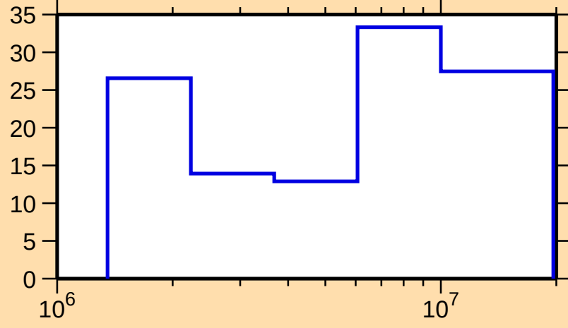
\Delta\sigma/\sigma vs. E for ^{244}\text{Pu}(n,\text{f})
