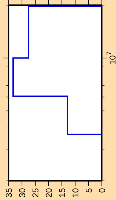
\Delta\sigma/\sigma vs. E for ^{244}\text{Pu}(n,f)
