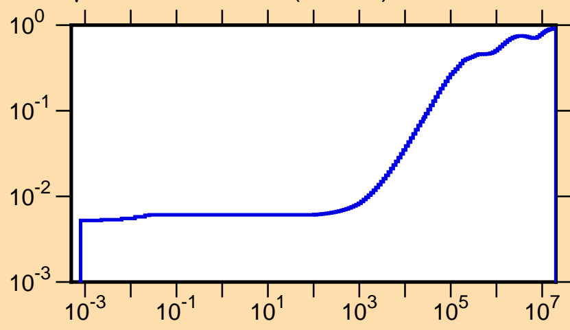
\mu vs. E for ^{130}\text{Sm}(\text{mt251})
