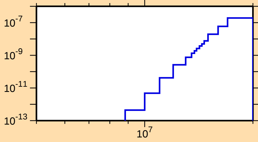
\sigma vs. E for ^{130}\text{Sm}(\text{mt117})
