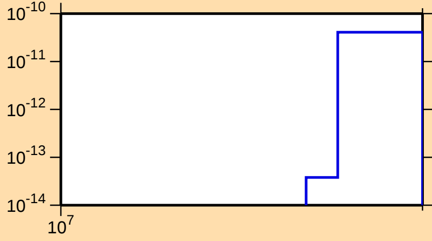
\sigma vs. E for ^{130}\text{Sm}(n,2n\alpha)
