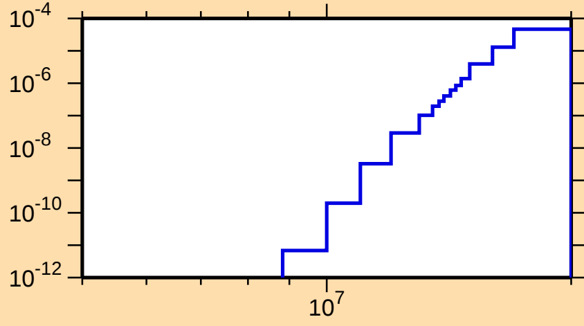
\sigma vs. E for ^{130}\text{Sm}(\text{mt } 45)
