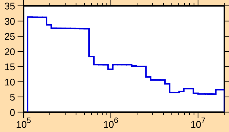
\Delta\sigma/\sigma vs. E for ^{130}\text{Sm}(n,\text{nonel.})
