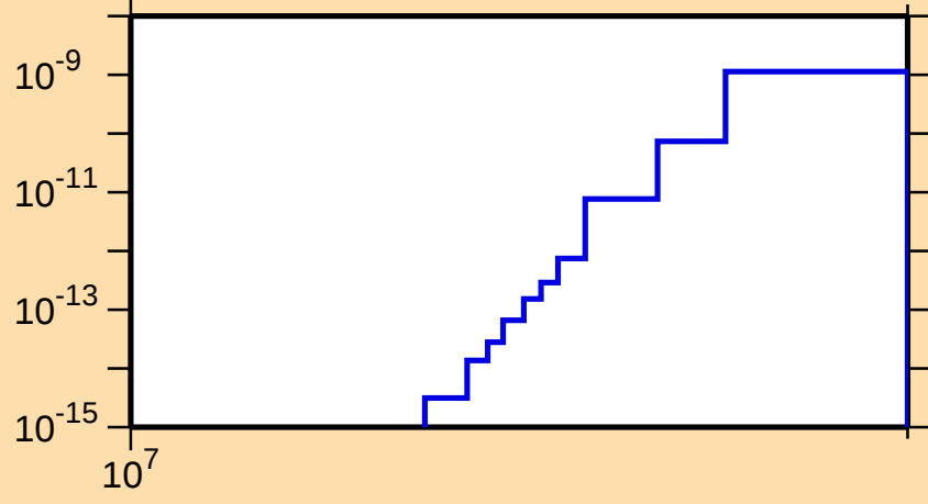
\sigma vs. E for ^{130}\text{Sm}(\text{mt } 34)
