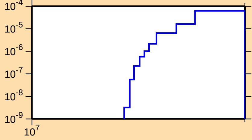
\sigma vs. E for ^{130}\text{Sm}(n,2n)
