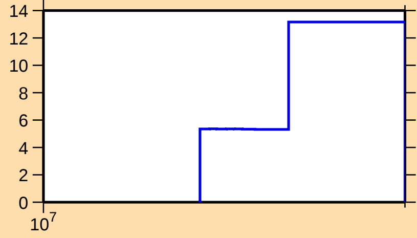
\Delta\sigma/\sigma vs. E for ^{130}\text{Sm}(n,\text{el.})
