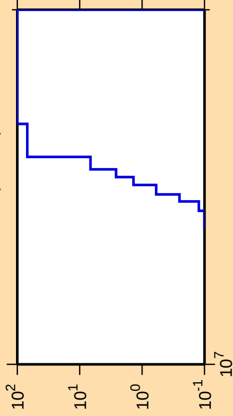
\Delta\sigma/\sigma vs. E for ^{130}\text{Sm}(\text{mt } 34)
