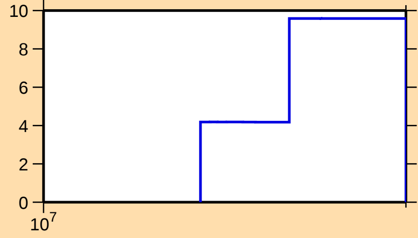
\Delta\sigma/\sigma vs. E for ^{130}\text{Sm}(n,\text{tot.})
