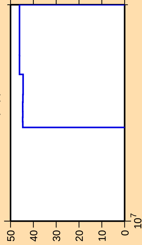
\Delta\sigma/\sigma vs. E for ^{130}\text{Sm}(n,p)
