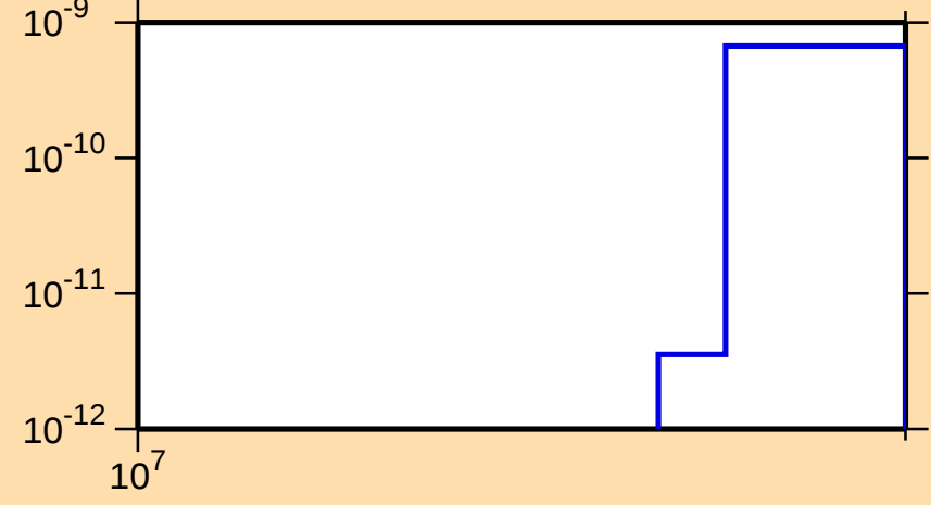
\sigma vs. E for ^{130}\text{Sm}(n,\text{nd})
