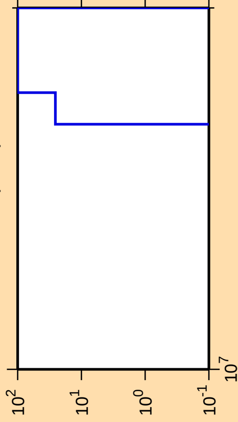
\Delta\sigma/\sigma vs. E for ^{130}\text{Sm}(n,\text{nd})
