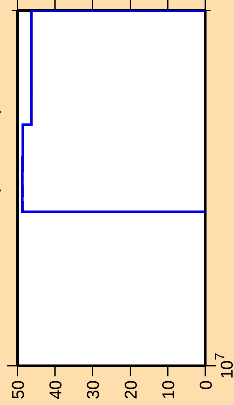
\Delta\sigma/\sigma vs. E for ^{130}\text{Sm}(n,n\text{cont.})
