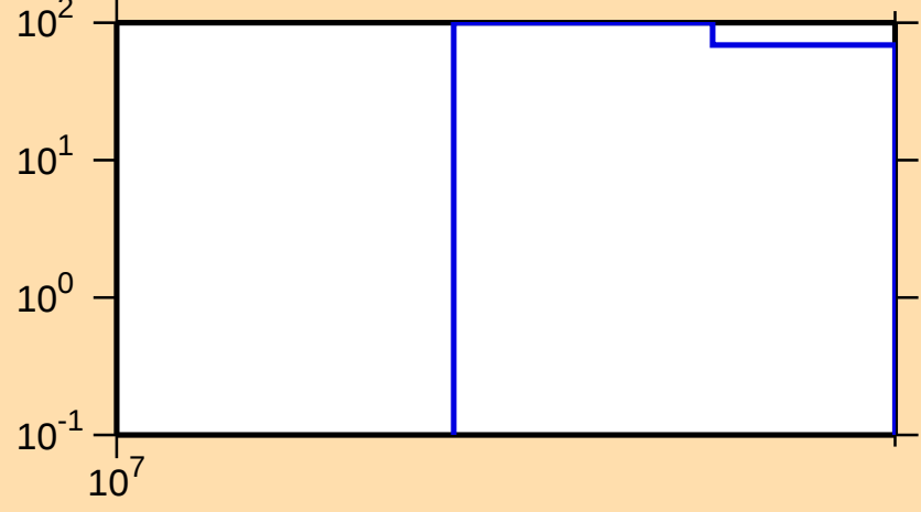
\Delta\sigma/\sigma vs. E for ^{130}\text{Sm}(n,2n)
