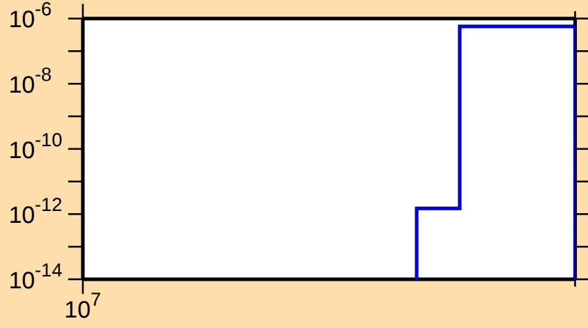
\sigma vs. E for ^{130}\text{Sm}(n,2np)
