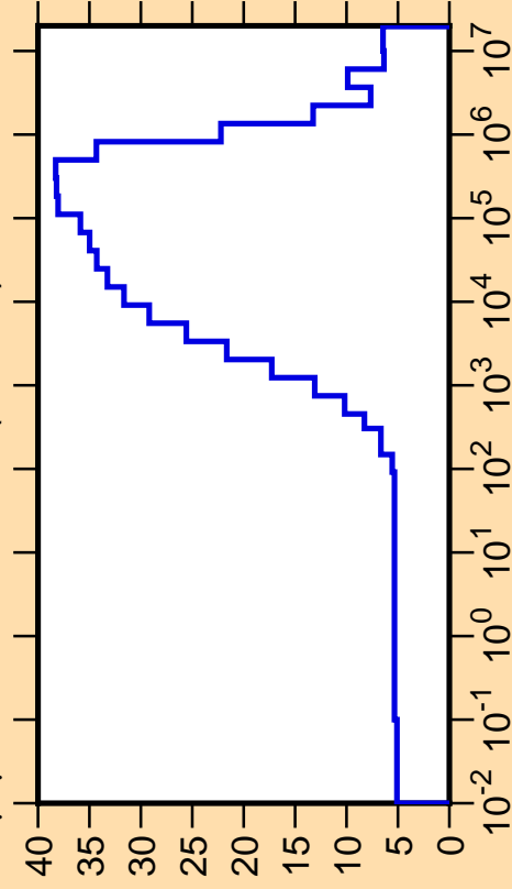
\Delta\mu/\mu vs. E for ^{130}\text{Sm}(\text{mt251})
