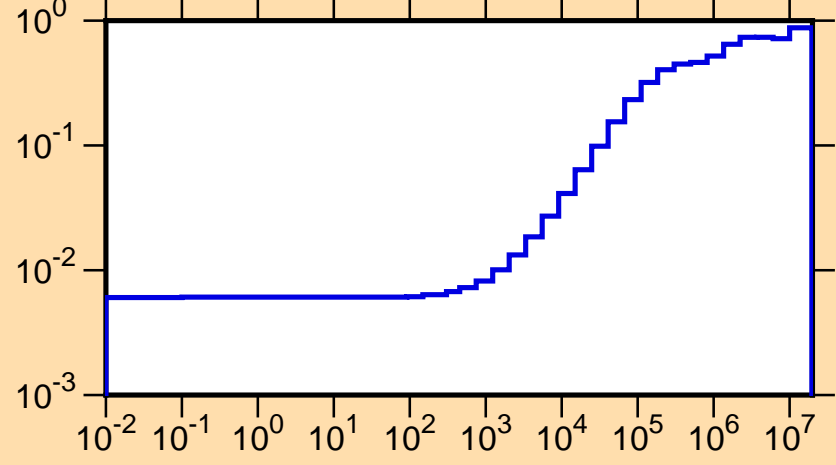
\mu vs. E for ^{130}\text{Sm}(\text{mt251})
