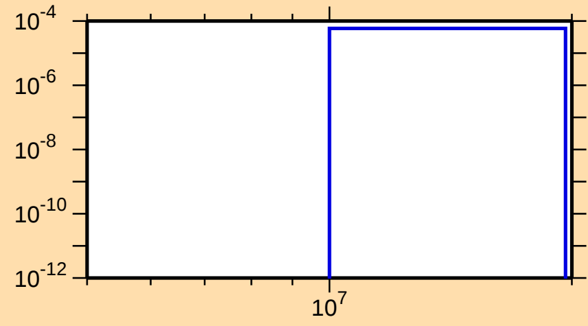
\sigma vs. E for ^{130}\text{Sm}(n,t)
