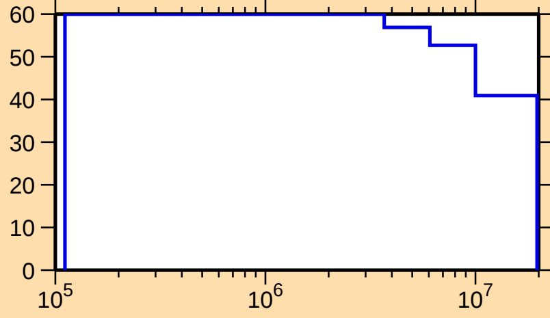
\Delta\sigma/\sigma vs. E for ^{130}\text{Sm}(n,\text{inel.})
