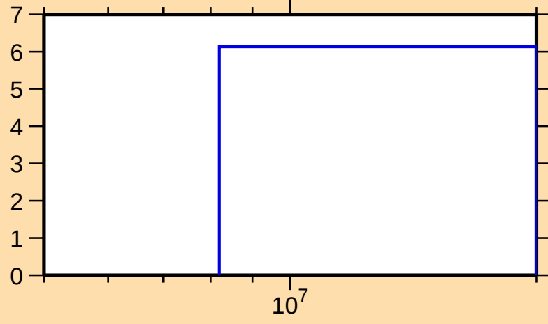
\Delta\sigma/\sigma vs. E for ^{130}\text{Sm}(n,\text{nonel.})
