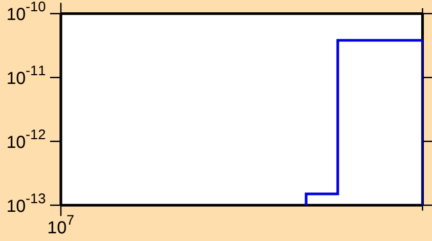
\sigma vs. E for ^{138}\text{Sm}(\text{mt } 34)
