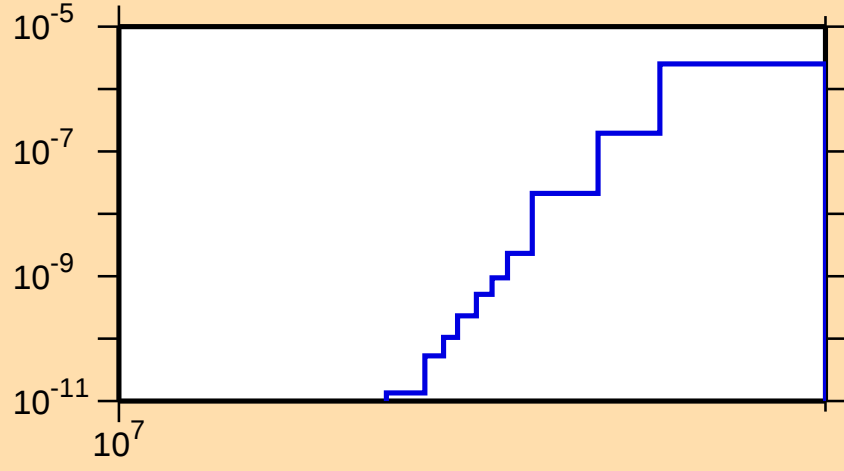
\sigma vs. E for ^{138}\text{Sm}(\text{mt } 45)
