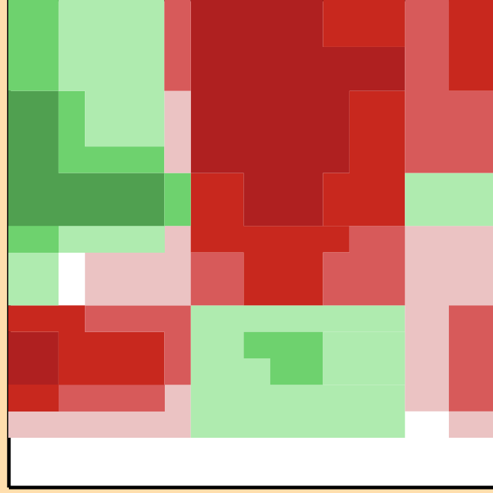
\Delta\sigma/\sigma vs. E for ^{138}\text{Sm}(n,\text{el.})
